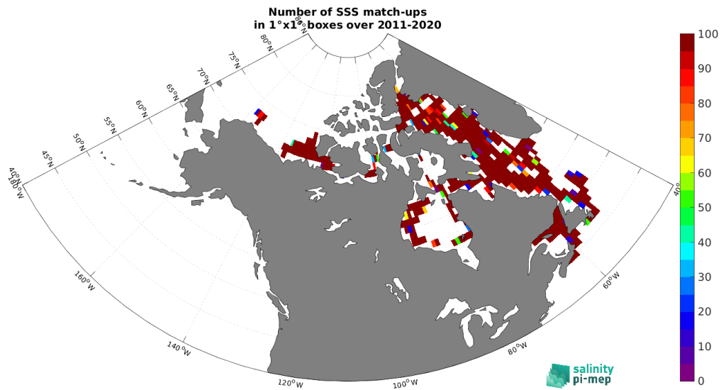
Figure 5: Number of SSS match-ups between TSG (Amundsen) SSS and the SMOS SSS L4 v2 - Daily (BEC) SSS product for the Global Ocean Pi-MEP region over 1°×1° boxes and for the full satellite product period.
