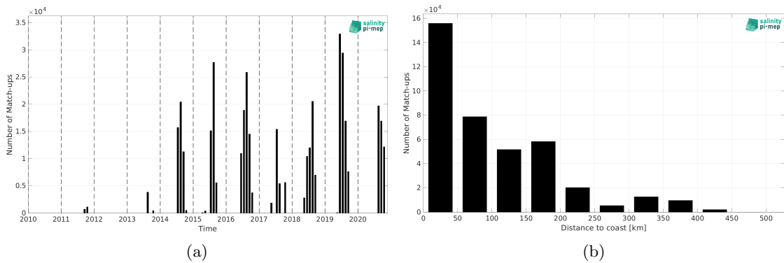
Figure 2: Number of match-ups between TSG (Amundsen) and SMOS SSS L4 v2 - Daily (BEC) SSS as a function of time (a) and as function of the distance to coast (b) over the Global Ocean Pi-MEP region and for the full satellite product period.
