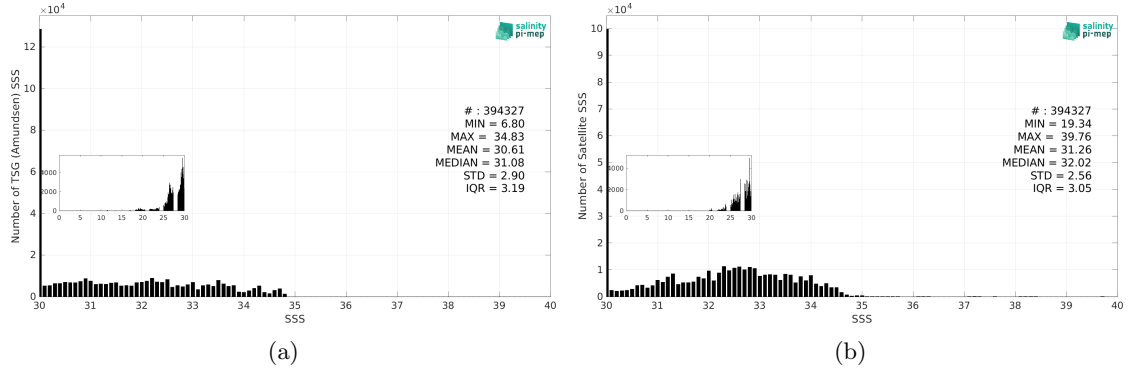
Figure 3: Histograms of SSS from TSG (Amundsen) (a) and SMOS SSS L4 v2 - Daily (BEC) (b) considering all match-up pairs per bins of 0.1 over the Global Ocean Pi-MEP region and for the full satellite product period.
