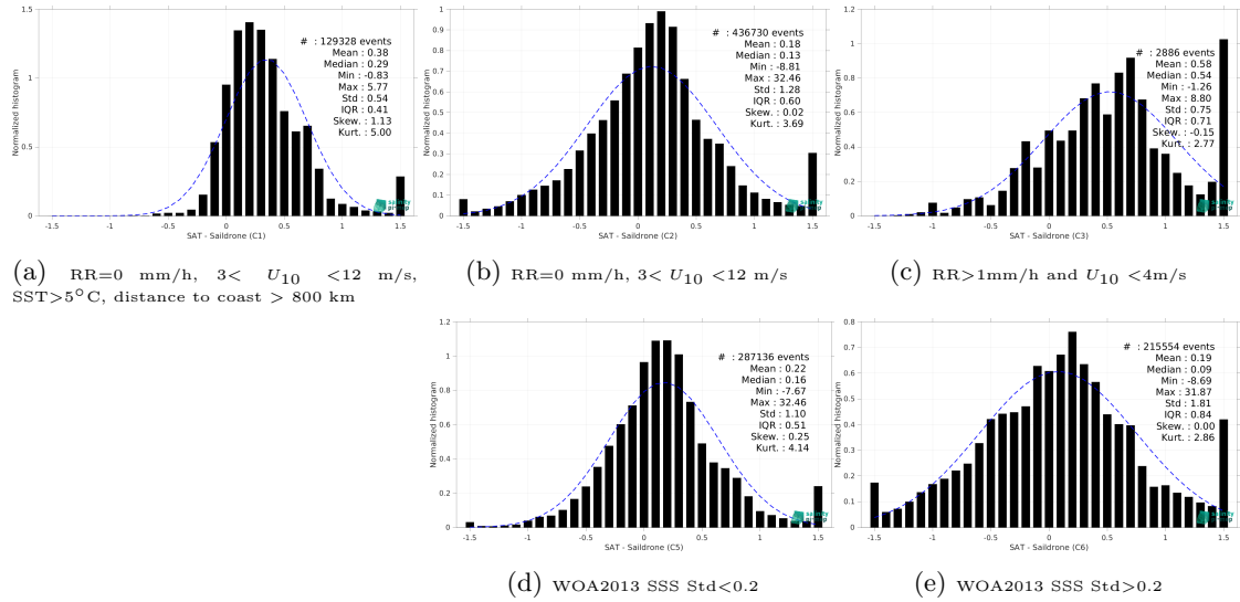
Figure 15: Normalized histogram of \Delta\text{SSS} (SMOS SSS L4 v2 - Daily (BEC) - Saildrone) for 5 different subdatasets corresponding to: RR=0 mm/h, 3 < U_{10} < 12 m/s, SST>5°C, distance to coast > 800 km (a), RR=0 mm/h, 3 < U_{10} < 12 m/s (b), RR>1mm/h and U_{10} < 4 m/s (c), WOA2013 SSS Std<0.2 (d), WOA2013 SSS Std>0.2 (e).
