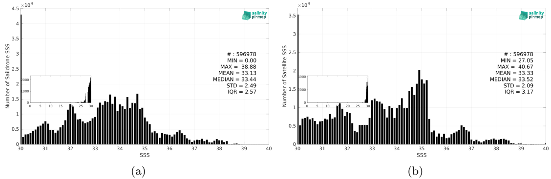
Figure 3: Histograms of SSS from Saildrone (a) and SMOS SSS L4 v2 - Daily (BEC) (b) considering all match-up pairs per bins of 0.1 over the Global Ocean Pi-MEP region and for the full satellite product period.
