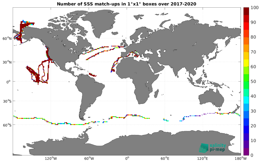
Figure 4: Number of SSS match-ups between Saildrone SSS and the SMOS SSS L4 v2 - Daily (BEC) SSS product for the Global Ocean Pi-MEP region over 1°×1° boxes and for the full satellite product period.
