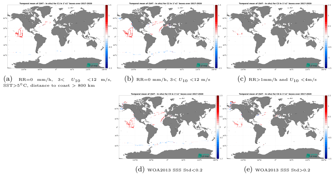
Figure 12: Temporal mean gridded over spatial boxes of size 1^\circ \times 1^\circ of \Delta SSS (SMOS SSS L4 v2 - Daily (BEC) - Saldrone) for 5 different subdatasets corresponding to:RR=0 mm/h, 3 < U_{10} < 12 m/s, SST > 5^\circ\text{C} , distance to coast > 800 km (a), RR=0 mm/h, 3 < U_{10} < 12 m/s (b), RR > 1 mm/h and U_{10} < 4 m/s (c), WOA2013 SSS Std < 0.2 (d), WOA2013 SSS Std > 0.2 (e).
