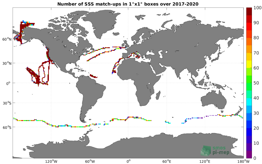
Figure 4: Number of SSS match-ups between Saildrone SSS and the SMOS SSS L4 v2 - Daily (BEC) SSS product for the Global Ocean Pi-MEP region over 1^\circ \times 1^\circ boxes and for the full satellite product period.
