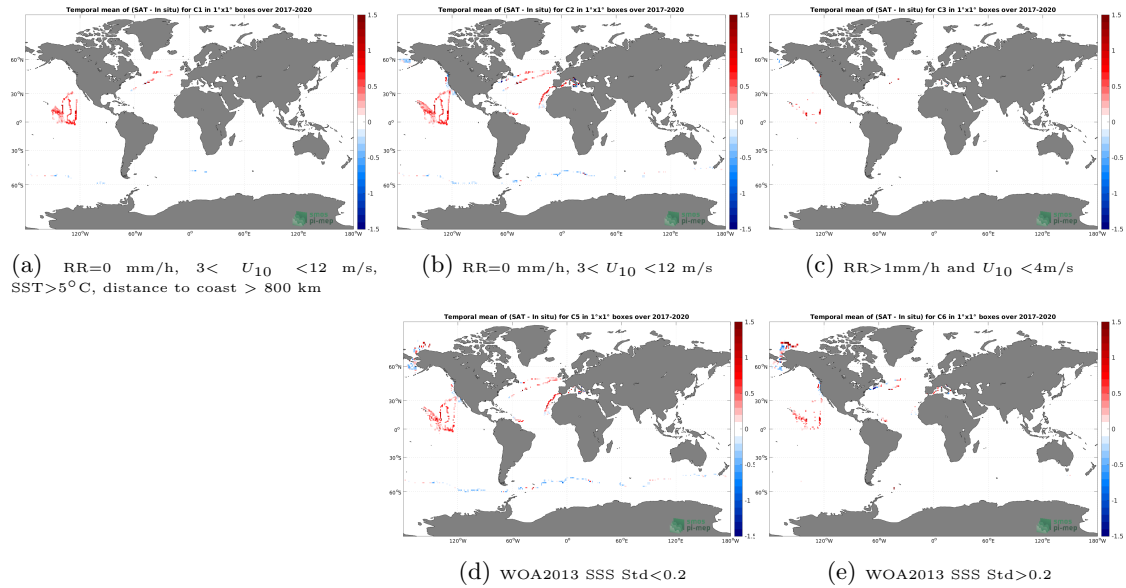
Figure 12: Temporal mean gridded over spatial boxes of size 1^\circ \times 1^\circ of \Delta SSS (SMOS SSS L4 v2 - Daily (BEC) - Sairdrone) for 5 different subdatasets corresponding to:RR=0 mm/h, 3 < U_{10} < 12 m/s, SST >5^\circ\text{C} , distance to coast > 800 km (a), RR=0 mm/h, 3 < U_{10} < 12 m/s (b), RR >1 mm/h and U_{10} < 4 m/s (c), WOA2013 SSS Std <0.2 (d), WOA2013 SSS Std >0.2 (e).
