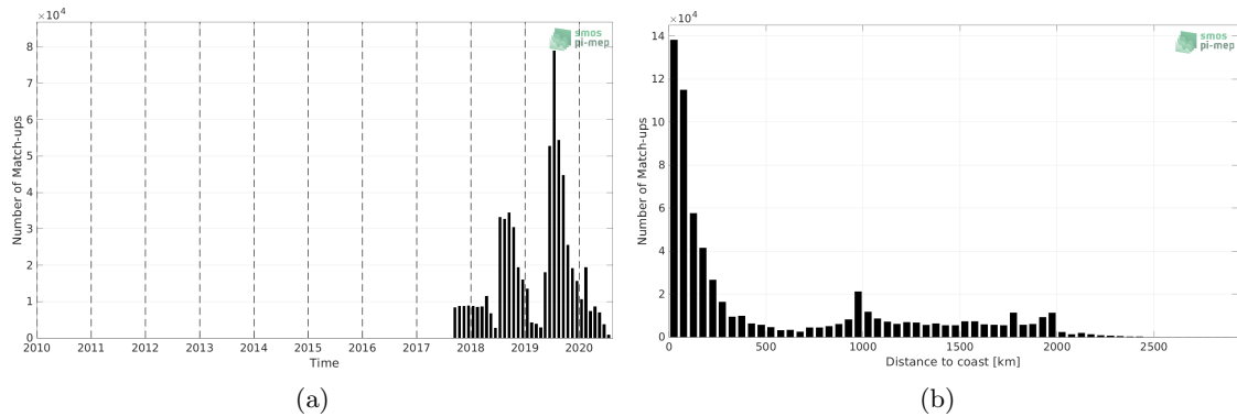
Figure 1: Number of match-ups between Saildrone and SMOS SSS L4 v2 - Daily (BEC) SSS as a function of time (a) and as function of the distance to coast (b) over the Global Ocean Pi-MEP region and for the full satellite product period.
