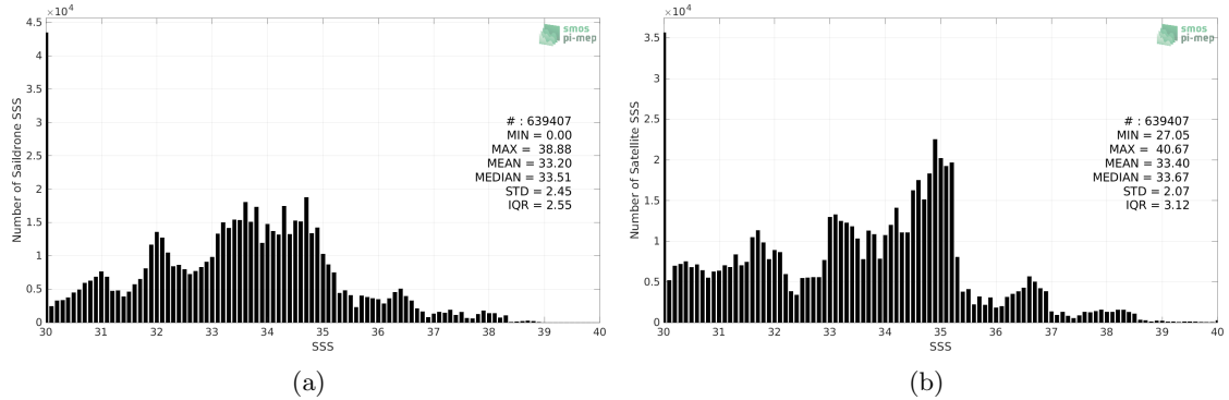
Figure 2: Histograms of SSS from Saildrone (a) and SMOS SSS L4 v2 - Daily (BEC) (b) considering all match-up pairs per bins of 0.1 over the Global Ocean Pi-MEP region and for the full satellite product period.
