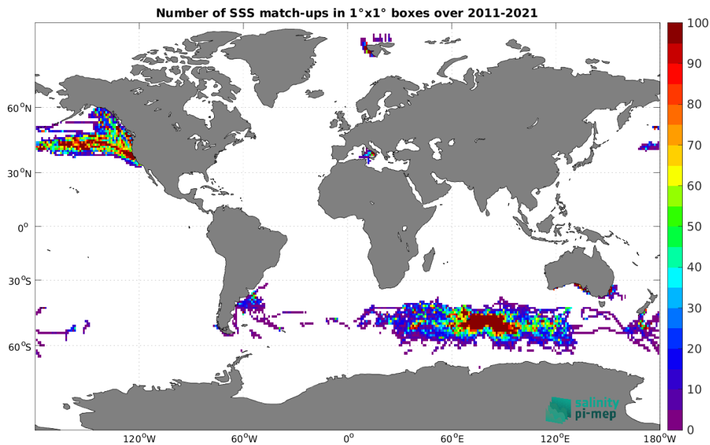
Figure 5: Number of SSS match-ups between Marine mammals SSS and the SMOS SSS L4 v2 - Daily (BEC) SSS product for the Global Ocean Pi-MEP region over 1^\circ \times 1^\circ boxes and for the full satellite product period.
