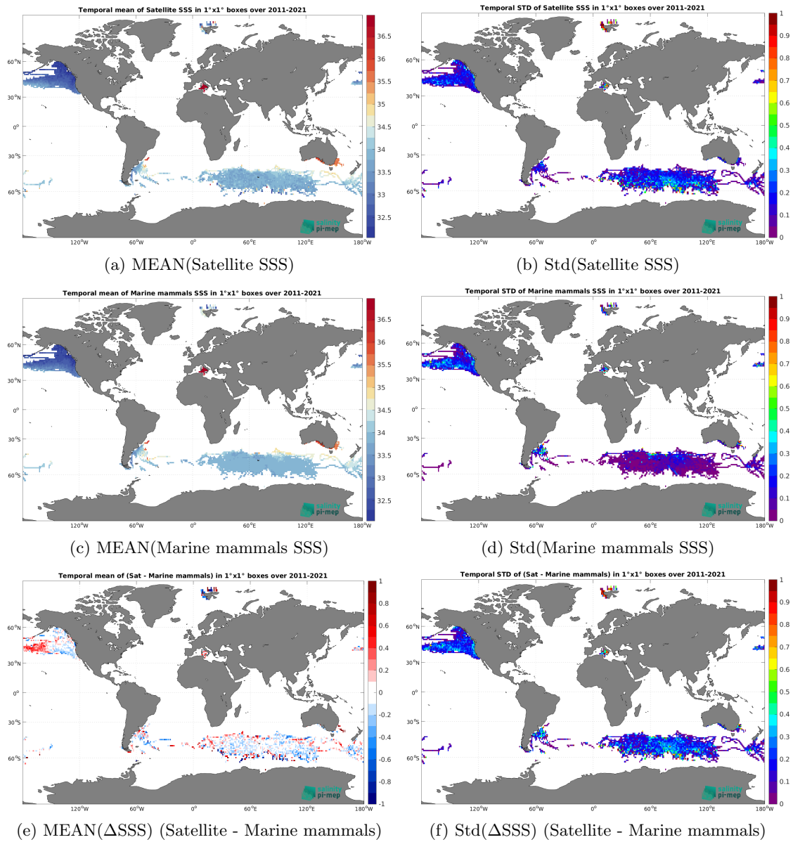
Figure 7: Temporal mean (left) and Std (right) of SSS from SMOS SSS L4 v2 - Daily (BEC) (top), Marine mammals (middle), and of \Delta SSS (Satellite - Marine mammals). Only match-up pairs are used to generate these maps.
