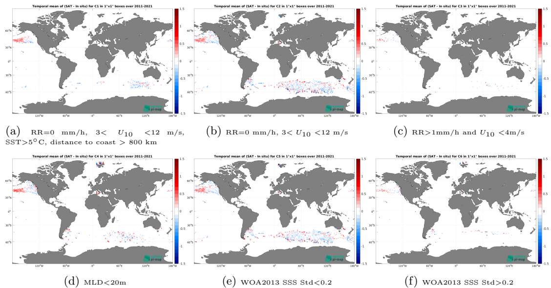
Figure 14: Temporal mean gridded over spatial boxes of size 1^\circ \times 1^\circ of \Delta SSS (SMOS SSS L4 v2 - Daily (BEC) - Marine mammals) for 6 different subdatasets corresponding to:RR=0 mm/h, 3 < U_{10} < 12 m/s, SST >5^\circ\text{C} , distance to coast > 800 km (a), RR=0 mm/h, 3 < U_{10} < 12 m/s (b), RR >1 mm/h and U_{10} < 4 m/s (c),MLD <20 m (d),WOA2013 SSS Std <0.2 (e),WOA2013 SSS Std >0.2 (f).
