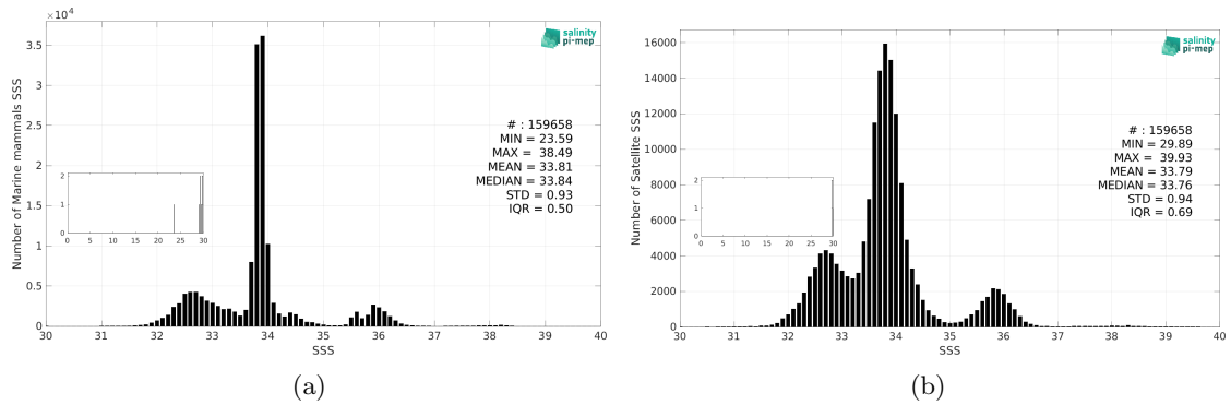
Figure 3: Histograms of SSS from Marine mammals (a) and SMOS SSS L4 v2 - Daily (BEC) (b) considering all match-up pairs per bins of 0.1 over the Global Ocean Pi-MEP region and for the full satellite product period.
