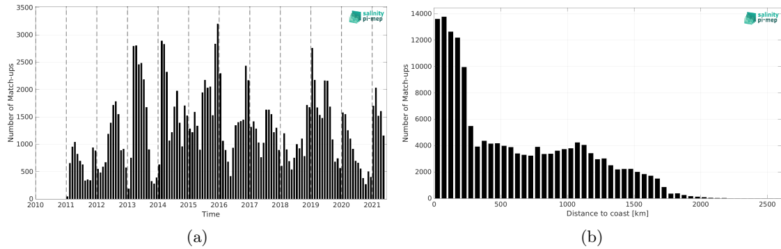
Figure 2: Number of match-ups between Marine mammals and SMOS SSS L4 v2 - Daily (BEC) SSS as a function of time (a) and as function of the distance to coast (b) over the Global Ocean Pi-MEP region and for the full satellite product period.
