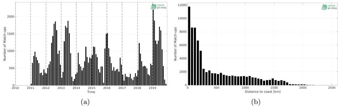
Figure 1: Number of match-ups between Marine mammals and SMOS SSS L4 v2 - Daily (BEC) SSS as a function of time (a) and as function of the distance to coast (b) over the Global Ocean Pi-MEP region and for the full satellite product period.
