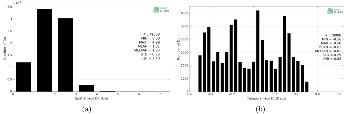
Figure 5: Histograms of the spatial (a) and temporal (b) lags between the location/time of the Marine mammals measurement and the date of the corresponding SMOS SSS L4 v2 - Daily (BEC) SSS pixel.
