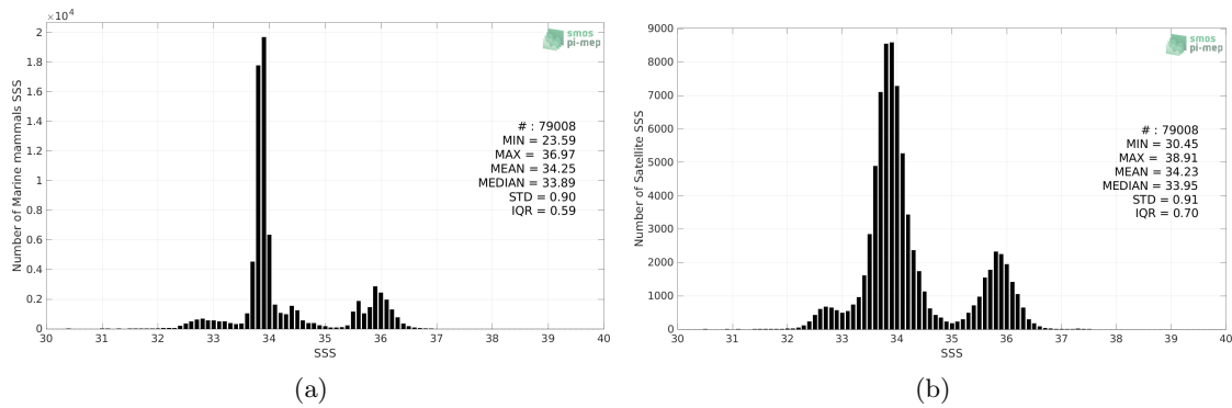
Figure 2: Histograms of SSS from Marine mammals (a) and SMOS SSS L4 v2 - Daily (BEC) (b) considering all match-up pairs per bins of 0.1 over the Global Ocean Pi-MEP region and for the full satellite product period.
