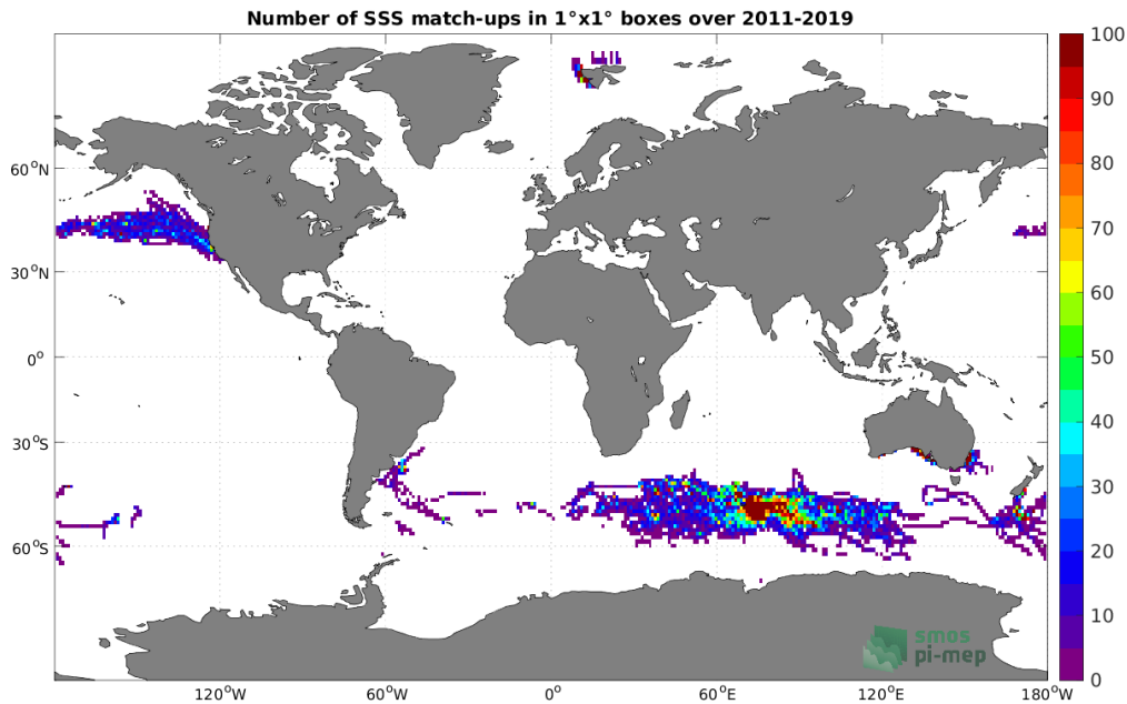
Figure 4: Number of SSS match-ups between Marine mammals SSS and the SMOS SSS L4 v2 - Daily (BEC) SSS product for the Global Ocean Pi-MEP region over 1^\circ \times 1^\circ boxes and for the full satellite product period.
