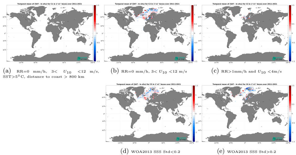
Figure 14: Temporal mean gridded over spatial boxes of size 1^\circ \times 1^\circ of \Delta SSS (SMOS SSS L4 v2 - Daily (BEC) - ICES) for 5 different subdatasets corresponding to:RR=0 mm/h, 3 < U_{10} < 12 m/s, SST>5°C, distance to coast > 800 km (a), RR=0 mm/h, 3 < U_{10} < 12 m/s (b), RR>1mm/h and U_{10} < 4 m/s (c), WOA2013 SSS Std<0.2 (d), WOA2013 SSS Std>0.2 (e).
