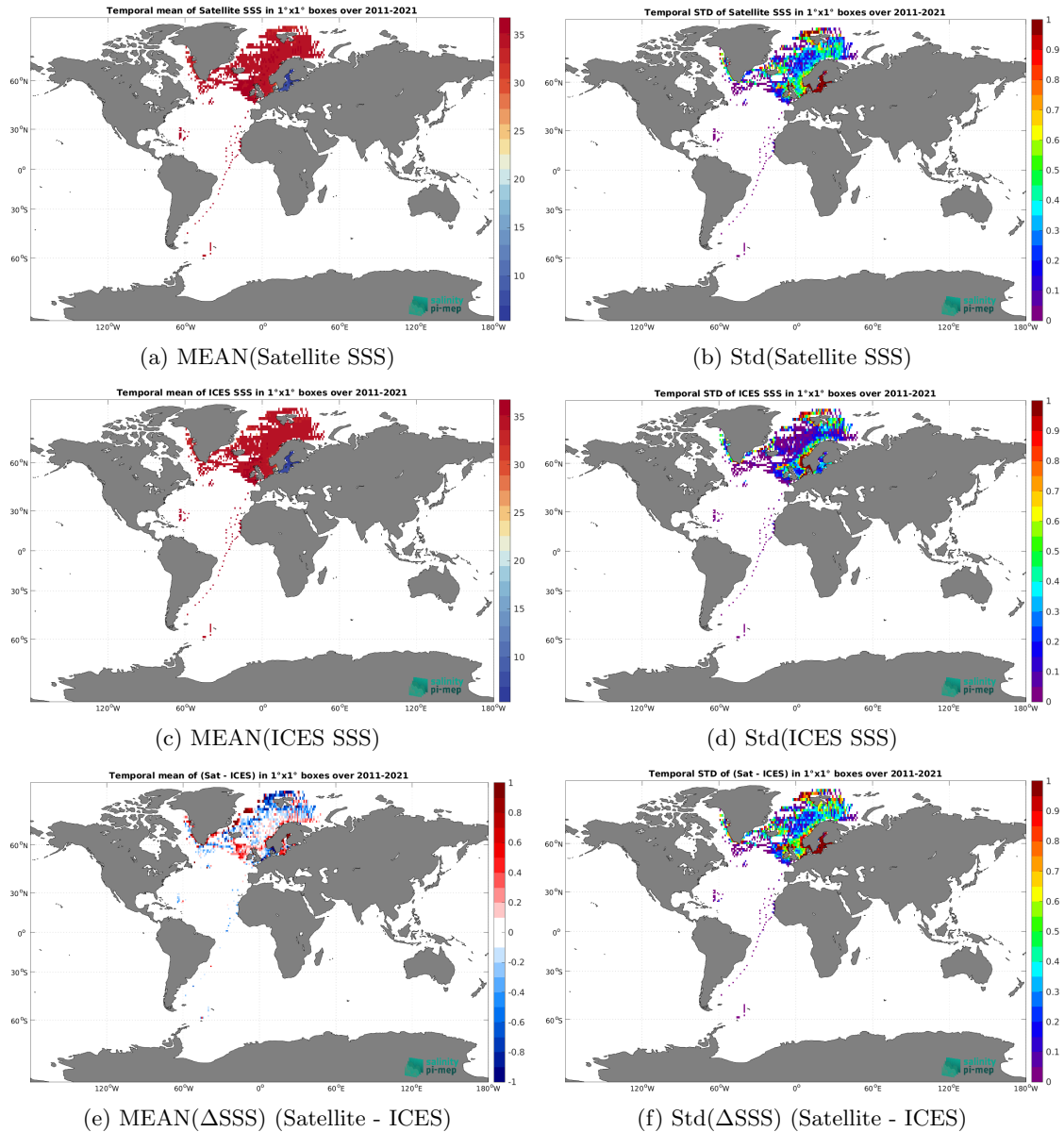
Figure 6: Temporal mean (left) and Std (right) of SSS from SMOS SSS L4 v2 - Daily (BEC) (top), ICES (middle), and of \Delta SSS (Satellite - ICES). Only match-up pairs are used to generate these maps.
