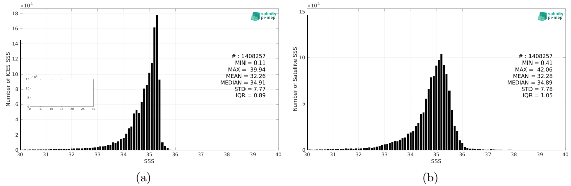
Figure 2: Histograms of SSS from ICES (a) and SMOS SSS L4 v2 - Daily (BEC) (b) considering all match-up pairs per bins of 0.1 over the Global Ocean Pi-MEP region and for the full satellite product period.
