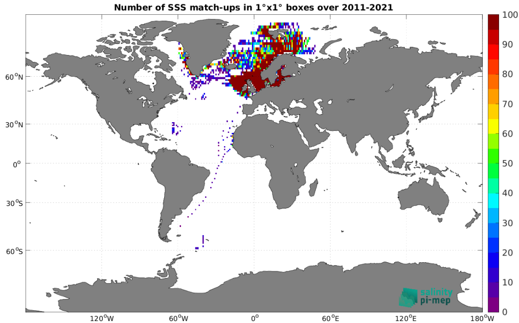
Figure 4: Number of SSS match-ups between ICES SSS and the SMOS SSS L4 v2 - Daily (BEC) SSS product for the Global Ocean Pi-MEP region over 1^\circ \times 1^\circ boxes and for the full satellite product period.
