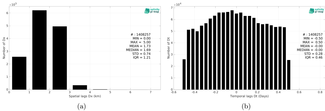
Figure 5: Histograms of the spatial (a) and temporal (b) lags between the location/time of the ICES measurement and the date of the corresponding SMOS SSS L4 v2 - Daily (BEC) SSS pixel.
