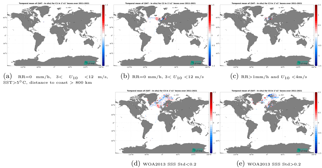
Figure 12: Temporal mean gridded over spatial boxes of size 1^\circ \times 1^\circ of \Delta SSS (SMOS SSS L4 v2 - Daily (BEC) - ICES) for 5 different subdatasets corresponding to:RR=0 mm/h, 3 < U_{10} < 12 m/s, SST >5^\circ\text{C} , distance to coast > 800 km (a), RR=0 mm/h, 3 < U_{10} < 12 m/s (b), RR >1 mm/h and U_{10} < 4 m/s (c), WOA2013 SSS Std <0.2 (d), WOA2013 SSS Std >0.2 (e).
