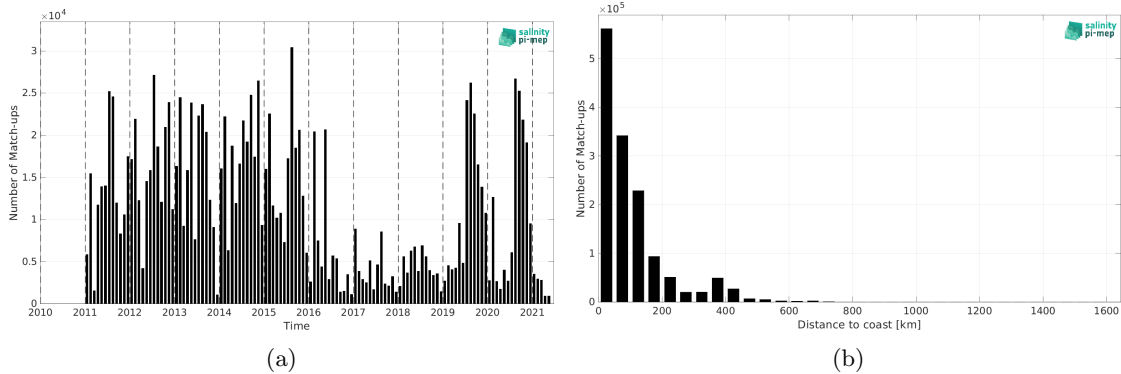
Figure 1: Number of match-ups between ICES and SMOS SSS L4 v2 - Daily (BEC) SSS as a function of time (a) and as function of the distance to coast (b) over the Global Ocean Pi-MEP region and for the full satellite product period.
