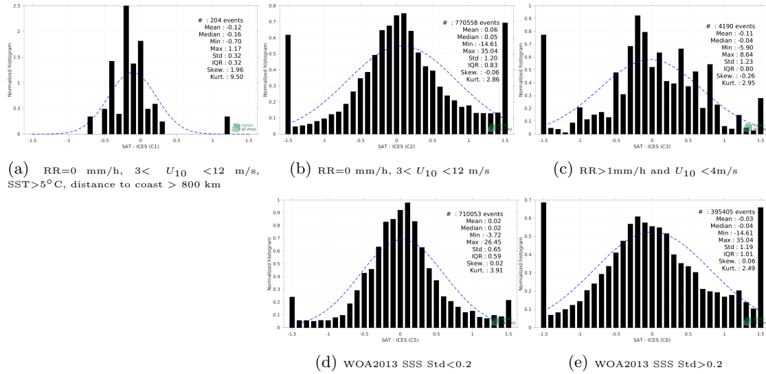
Figure 13: Normalized histogram of \Delta SSS (SMOS SSS L4 v2 - Daily (BEC) - ICES) for 5 different subdatasets corresponding to: RR=0 mm/h, 3 < U_{10} < 12 m/s, SST>5°C, distance to coast > 800 km (a), RR=0 mm/h, 3 < U_{10} < 12 m/s (b), RR>1mm/h and U_{10} < 4 m/s (c), WOA2013 SSS Std<0.2 (d), WOA2013 SSS Std>0.2 (e).
