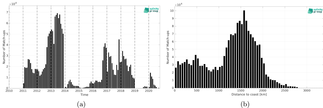
Figure 1: Number of match-ups between Surface drifters and SMOS SSS L4 v2 - Daily (BEC) SSS as a function of time (a) and as function of the distance to coast (b) over the Global Ocean Pi-MEP region and for the full satellite product period.
