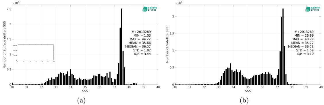
Figure 2: Histograms of SSS from Surface drifters (a) and SMOS SSS L4 v2 - Daily (BEC) (b) considering all match-up pairs per bins of 0.1 over the Global Ocean Pi-MEP region and for the full satellite product period.
