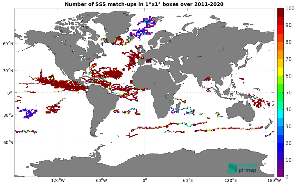
Figure 3: Number of SSS match-ups between Surface drifters SSS and the SMOS SSS L4 v2 - Daily (BEC) SSS product for the Global Ocean Pi-MEP region over 1°x1° boxes and for the full satellite product period.
