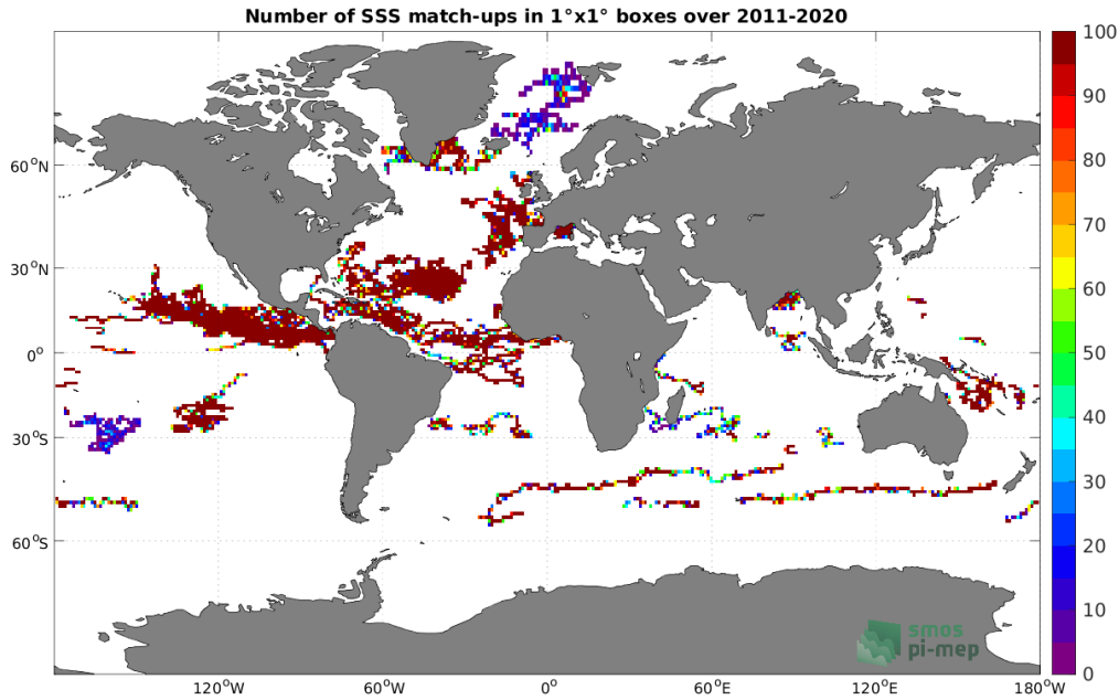
Figure 3: Number of SSS match-ups between Surface drifters SSS and the SMOS SSS L4 v2 - Daily (BEC) SSS product for the Global Ocean Pi-MEP region over 1°×1° boxes and for the full satellite product period.
