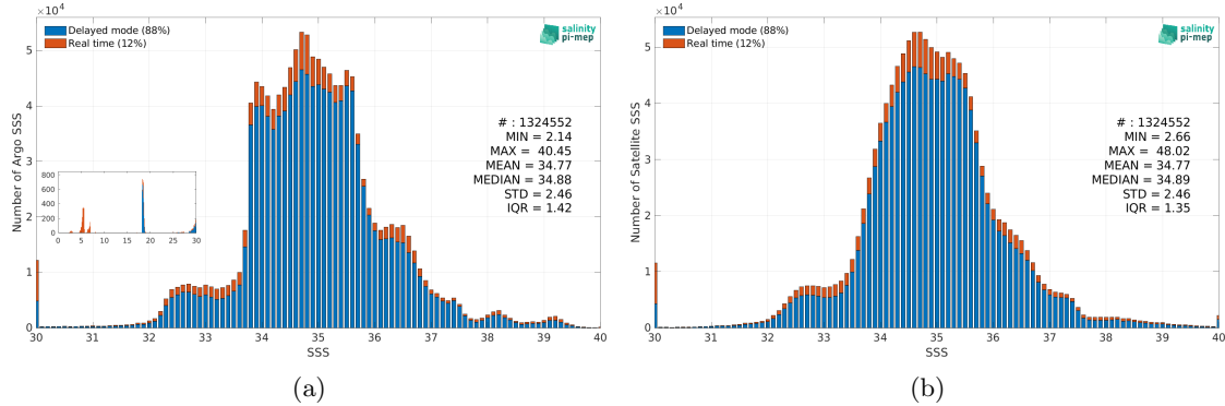
Figure 2: Histograms of SSS from Argo (a) and SMOS SSS L4 v2 - Daily (BEC) (b) considering all match-up pairs per bins of 0.1 over the Global Ocean Pi-MEP region and for the full satellite product period.
