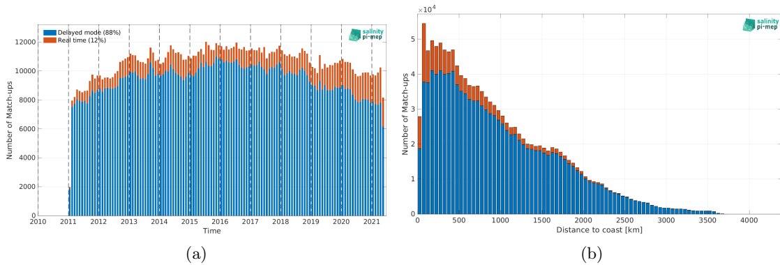
Figure 1: Number of match-ups between Argo and SMOS SSS L4 v2 - Daily (BEC) SSS as a function of time (a) and as function of the distance to coast (b) over the Global Ocean Pi-MEP region and for the full satellite product period.
