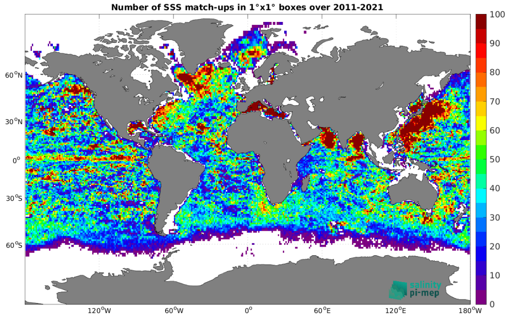
Figure 4: Number of SSS match-ups between Argo SSS and the SMOS SSS L4 v2 - Daily (BEC) SSS product for the Global Ocean Pi-MEP region over 1^\circ \times 1^\circ boxes and for the full satellite product period.
