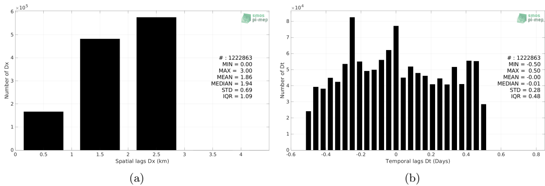
Figure 5: Histograms of the spatial (a) and temporal (b) lags between the location/time of the Argo measurement and the date of the corresponding SMOS SSS L4 v2 - Daily (BEC) SSS pixel.
