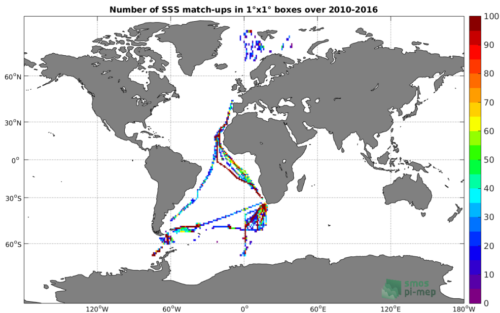
Figure 4: Number of SSS match-ups between TSG-POLARSTERN SSS and the SMOS-L3-ICDC-V3-MONTHLY-0.5DEG SSS product for the Global Ocean Pi-MEP region over 1°x1° boxes and for the full satellite product period.
