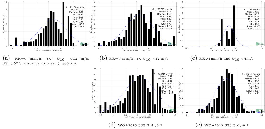
Figure 13: Normalized histogram of \Delta SSS (SMOS SSS L3 v3 Monthly (ICDC) - TSG (NCEI-0170743)) for 5 different subdatasets corresponding to: RR=0 mm/h, 3 < U_{10} < 12 m/s, SST>5°C, distance to coast > 800 km (a), RR=0 mm/h, 3 < U_{10} < 12 m/s (b), RR>1mm/h and U_{10} < 4 m/s (c), WOA2013 SSS Std<0.2 (d), WOA2013 SSS Std>0.2 (e).
