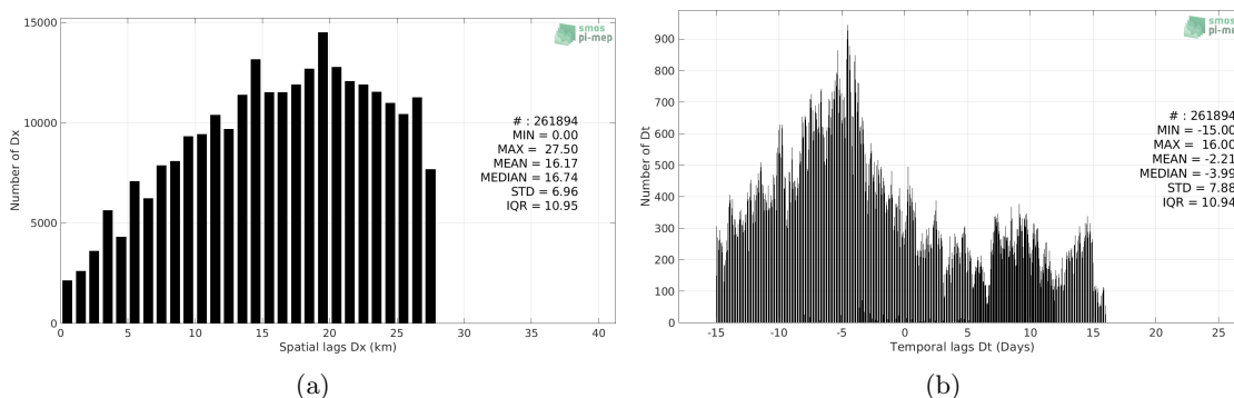
Figure 5: Histograms of the spatial (a) and temporal (b) lags between the location/time of the TSG (NCEI-0170743) measurement and the date of the corresponding SMOS SSS L3 v3 Monthly (ICDC) SSS pixel.
