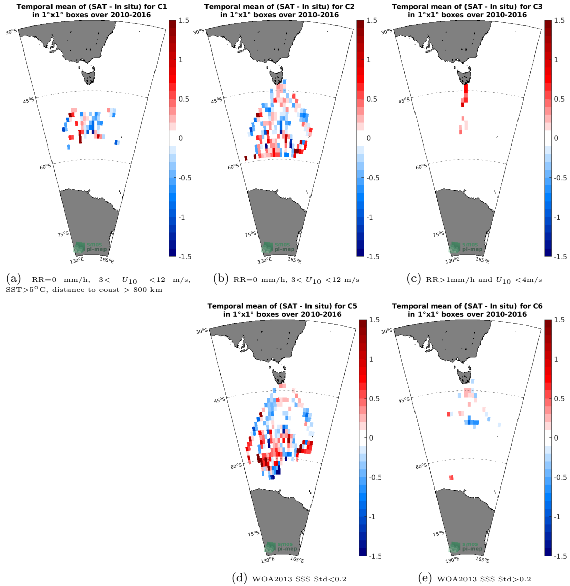
Figure 12: Temporal mean gridded over spatial boxes of size 1^\circ \times 1^\circ of \Delta\text{SSS} (SMOS SSS L3 v3 Monthly (ICDC) - TSG (LEGOS-Survostral)) for 5 different subdatasets corresponding to: RR=0 mm/h, 3 < U_{10} < 12 m/s, SST > 5^\circ\text{C} , distance to coast > 800 km (a), RR=0 mm/h, 3 < U_{10} < 12 m/s (b), RR > 1 mm/h and U_{10} < 4 m/s (c), WOA2013 SSS Std < 0.2 (d), WOA2013 SSS Std > 0.2 (e).
