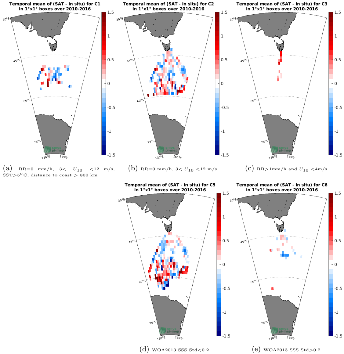
Figure 12: Temporal mean gridded over spatial boxes of size 1°x1° of \Delta SSS (SMOS SSS L3 v3 Monthly (ICDC) - TSG (LEGOS-Survostral)) for 5 different subdatasets corresponding to:RR=0 mm/h, 3 < U_{10} < 12 m/s, SST>5°C, distance to coast > 800 km (a), RR=0 mm/h, 3 < U_{10} < 12 m/s (b), RR>1mm/h and U_{10} < 4 m/s (c), WOA2013 SSS Std<0.2 (d), WOA2013 SSS Std>0.2 (e).
