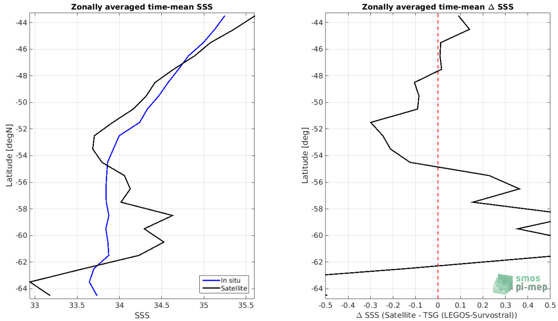
Figure 8: Left panel: Zonal mean SSS from SMOS SSS L3 v3 Monthly (ICDC) satellite product (black) and from TSG (LEGOS-Survostral) (blue). Right panel: Zonal mean of \Delta SSS (Satellite - TSG (LEGOS-Survostral)) for all the collected Pi-MEP match-up pairs estimated over the full satellite product period.
