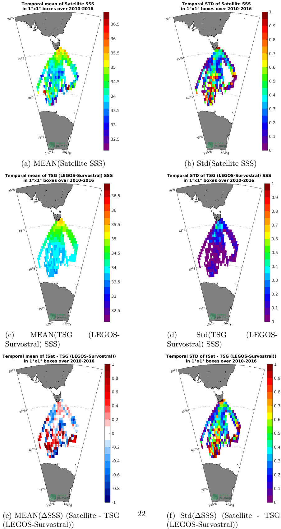
Figure 6: Temporal mean (left) and Std (right) of SSS from SMOS SSS L3 v3 Monthly (ICDC) (top), TSG (LEGOS-Survostral) (middle), and of \Delta SSS (Satellite - TSG (LEGOS-Survostral)). Only match-up pairs are used to generate these maps.
