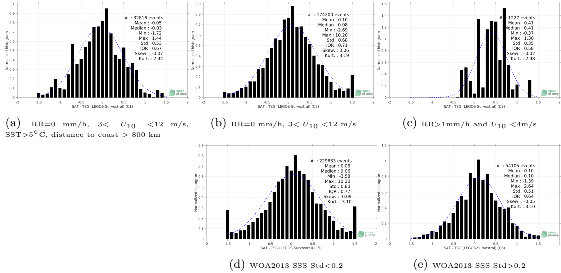
Figure 13: Normalized histogram of \Delta SSS (SMOS SSS L3 v3 Monthly (ICDC) - TSG (LEGOS-Survostral)) for 5 different subdatasets corresponding to: RR=0 mm/h, 3 < U_{10} < 12 m/s, SST > 5°C, distance to coast > 800 km (a), RR=0 mm/h, 3 < U_{10} < 12 m/s (b), RR > 1mm/h and U_{10} < 4 m/s (c), WOA2013 SSS Std < 0.2 (d), WOA2013 SSS Std > 0.2 (e).
