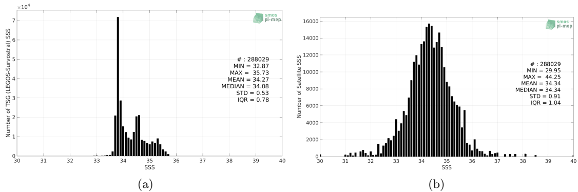
Figure 2: Histograms of SSS from TSG (LEGOS-Survostral) (a) and SMOS SSS L3 v3 Monthly (ICDC) (b) considering all match-up pairs per bins of 0.1 over the Global Ocean Pi-MEP region and for the full satellite product period.
