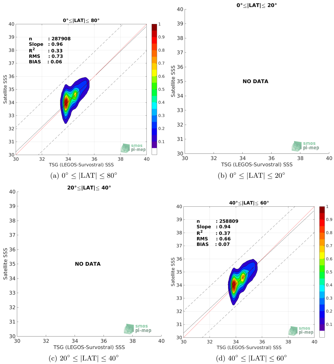
Figure 9: Contour maps of the concentration of SMOS SSS L3 v3 Monthly (ICDC) SSS (y-axis) versus TSG (LEGOS-Survostral) SSS (x-axis) at match-up pairs for different latitude bands. For each plot, the red line shows x=y . The black thin and dashed lines indicate a linear fit through the data cloud and the \pm 95\% confidence levels, respectively. The number match-up pairs n , the slope and R^2 coefficient of the linear fit, the root mean square (RMS) and the mean bias between satellite and in situ data are indicated for each latitude band in each plots.
