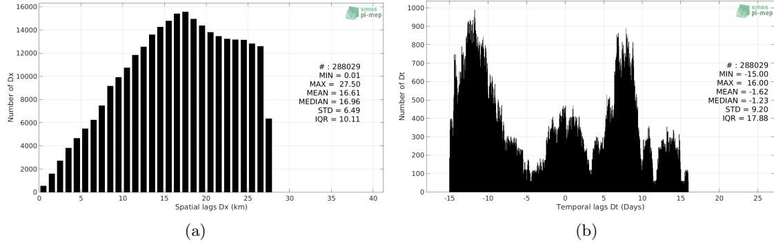
Figure 5: Histograms of the spatial (a) and temporal (b) lags between the time of the TSG (LEGOS-Survostral) measurements and the date of the corresponding SMOS SSS L3 v3 Monthly (ICDC) SSS product.
