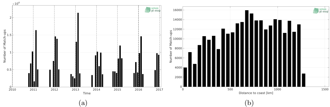
Figure 1: Number of match-ups between TSG (LEGOS-Survostral) and SMOS SSS L3 v3 Monthly (ICDC) SSS as a function of time (a) and as function of the distance to coast (b) over the Global Ocean Pi-MEP region and for the full satellite product period.
