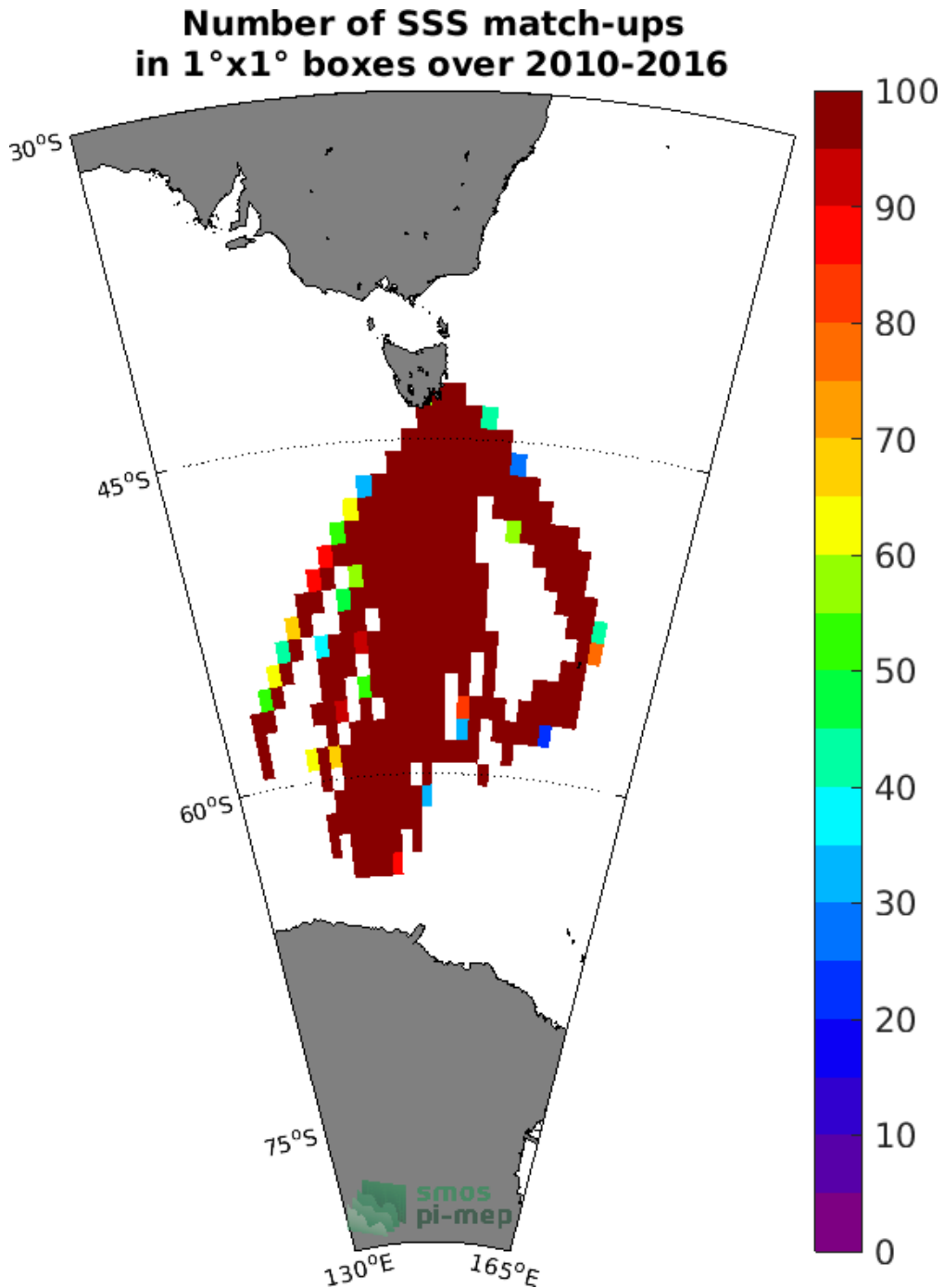
Figure 4: Number of SSS match-ups between TSG (LEGOS-Survostral) SSS and the SMOS SSS L3 v3 Monthly (ICDC) SSS product for the Global Ocean Pi-MEP region over 1°x1° boxes and for the full satellite product period.
