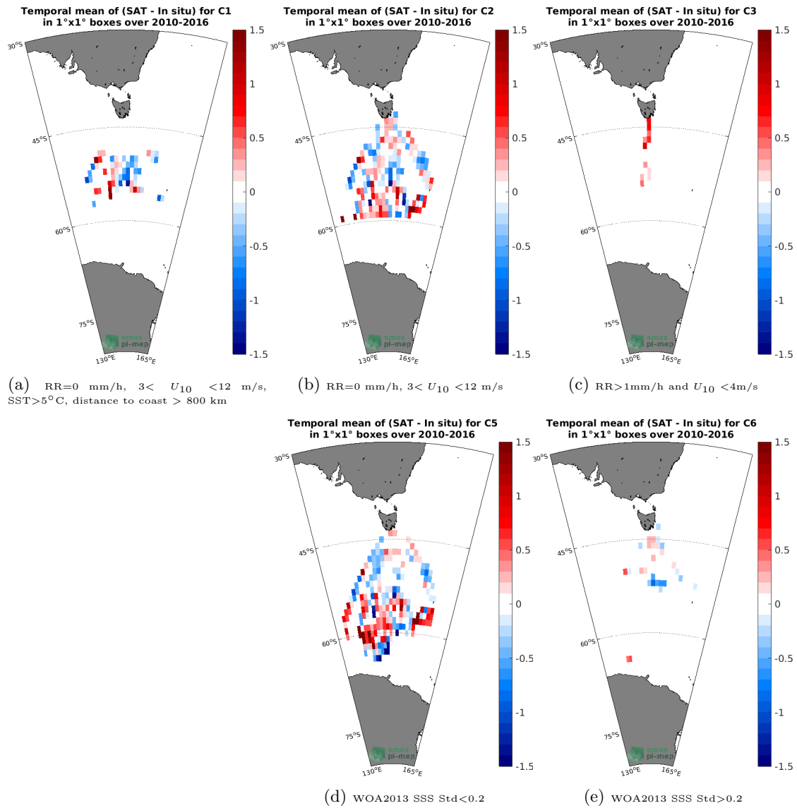
Figure 12: Temporal mean gridded over spatial boxes of size 1°x1° of \Delta SSS (SMOS SSS L3 v3 Monthly (ICDC) - TSG (LEGOS-Survostral)) for 5 different subdatasets corresponding to:RR=0 mm/h, 3 < U_{10} < 12 m/s, SST>5°C, distance to coast > 800 km (a), RR=0 mm/h, 3 < U_{10} < 12 m/s (b), RR>1mm/h and U_{10} < 4 m/s (c), WOA2013 SSS Std<0.2 (d), WOA2013 SSS Std>0.2 (e).
