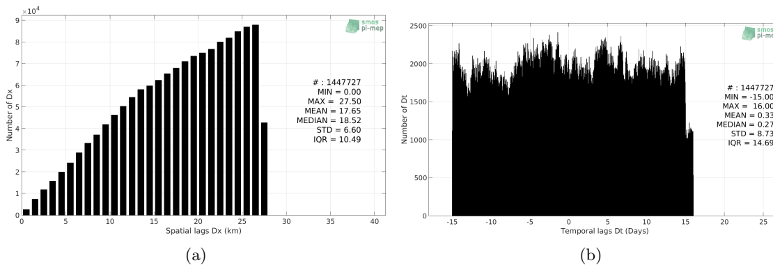
Figure 5: Histograms of the spatial (a) and temporal (b) lags between the location/time of the TSG (LEGOS-DM) measurement and the date of the corresponding SMOS SSS L3 v3 Monthly (ICDC) SSS pixel.
