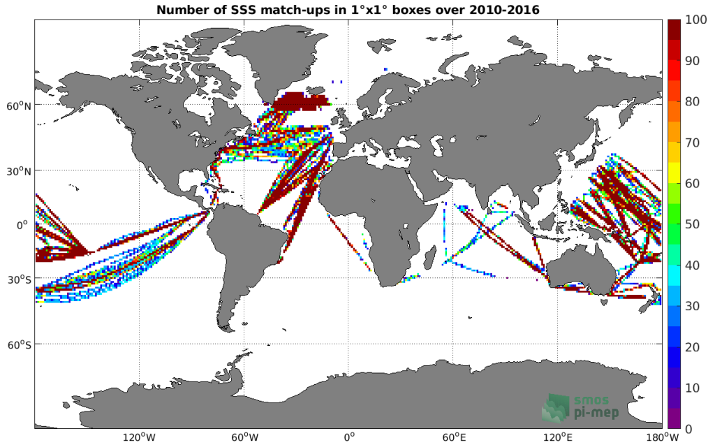
Figure 4: Number of SSS match-ups between TSG (LEGOS-DM) SSS and the SMOS SSS L3 v3 Monthly (ICDC) SSS product for the Global Ocean Pi-MEP region over 1^\circ \times 1^\circ boxes and for the full satellite product period.
