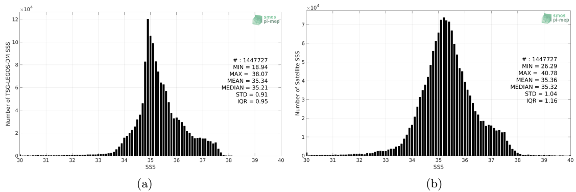
Figure 2: Histograms of SSS from TSG-LEGOS-DM (a) and SMOS-L3-ICDC-V3-MONTHLY-0.5DEG (b) considering all match-up pairs per bins of 0.1 over the Global Ocean Pi-MEP region and for the full satellite product period.
