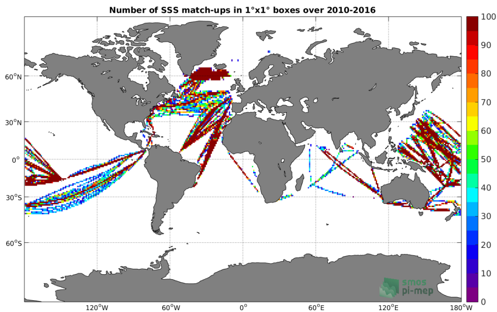
Figure 4: Number of SSS match-ups between TSG-LEGOS-DM SSS and the SMOS-L3-ICDC-V3-MONTHLY-0.5DEG SSS product for the Global Ocean Pi-MEP region over 1^\circ \times 1^\circ boxes and for the full satellite product period.
