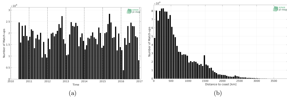
Figure 1: Number of match-ups between TSG-LEGOS-DM and SMOS-L3-ICDC-V3-MONTHLY-0.5DEG SSS as a function of time (a) and as function of the distance to coast (b) over the Global Ocean Pi-MEP region and for the full satellite product period.
