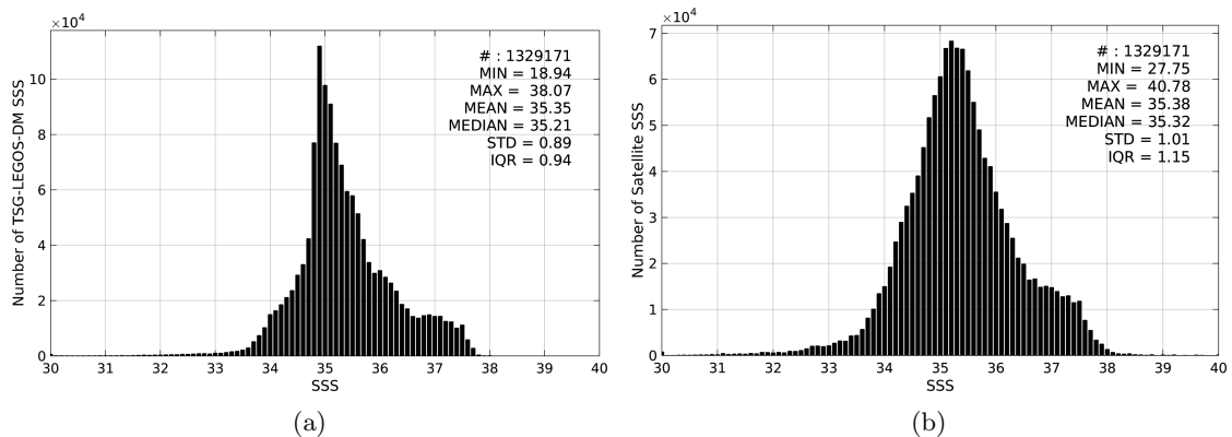
Figure 2: Histograms of SSS from TSG-LEGOS-DM (a) and SMOS-L3-ICDC-V3-MONTHLY-0.5DEG (b) considering all match-up pairs per bins of 0.1 over the Global Ocean Pi-MEP region and for the full satellite product period.
