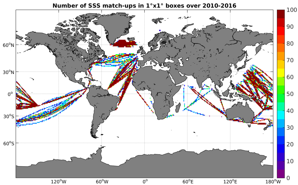
Figure 4: Number of SSS match-ups between TSG-LEGOS-DM SSS and the SMOS-L3-ICDC-V3-MONTHLY-0.5DEG SSS product for the Global Ocean Pi-MEP region over 1^\circ \times 1^\circ boxes and for the full satellite product period.
