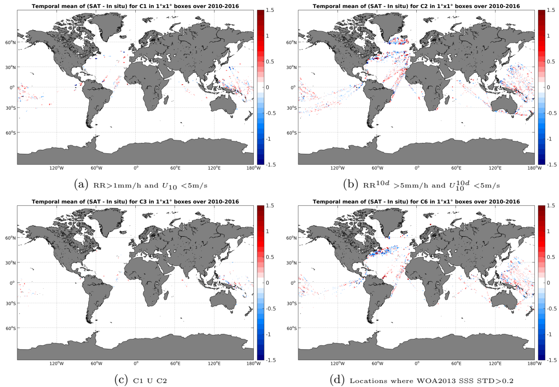
Figure 12: Temporal mean gridded over spatial boxes of size 1^\circ \times 1^\circ of \Delta SSS (SMOS-L3-ICDC-V3-MONTHLY-0.5DEG - TSG-LEGOS-DM) for 4 different subdatasets corresponding to: RR > 1\text{mm/h} and U_{10} < 5\text{m/s} (a), RR^{10d} > 5\text{mm/h} and U_{10}^{10d} < 5\text{m/s} (b), C1 U C2 (c), Locations where WOA2013 SSS STD > 0.2 (d).
