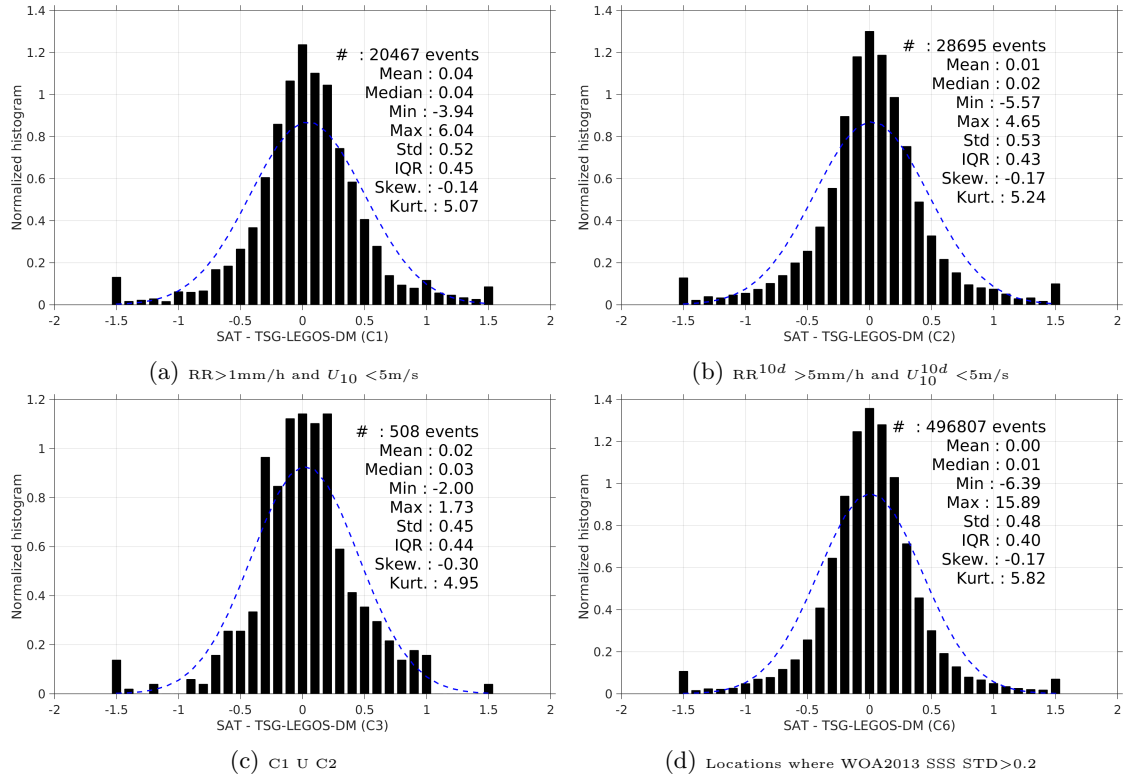
Figure 13: Normalized histogram of \Delta SSS (SMOS-L3-ICDC-V3-MONTHLY-0.5DEG - TSG-LEGOS-DM) for 6 different subdatasets corresponding to: RR > 1mm/h and U_{10} < 5 m/s (a), RR^{10d} > 5 mm/h and U_{10}^{10d} < 5 m/s (b), C1 U C2 (c), Locations where WOA2013 SSS STD > 0.2 (d).
