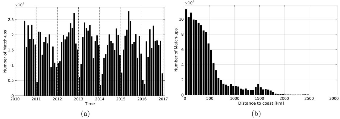
Figure 1: Number of match-ups between TSG-LEGOS-DM and SMOS-L3-ICDC-V3-MONTHLY-0.5DEG SSS as a function of time (a) and as function of the distance to coast (b) over the Global Ocean Pi-MEP region and for the full satellite product period.
