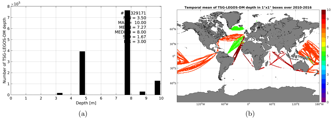
Figure 3: Histograms of the depth of the upper level SSS measurements from TSG-LEGOS-DM in the Match-up DataBase for the Global Ocean Pi-MEP region (a) and temporal mean spatial distribution of pressure of the in situ SSS data over 1^\circ \times 1^\circ boxes and for the full satellite product period (b).
