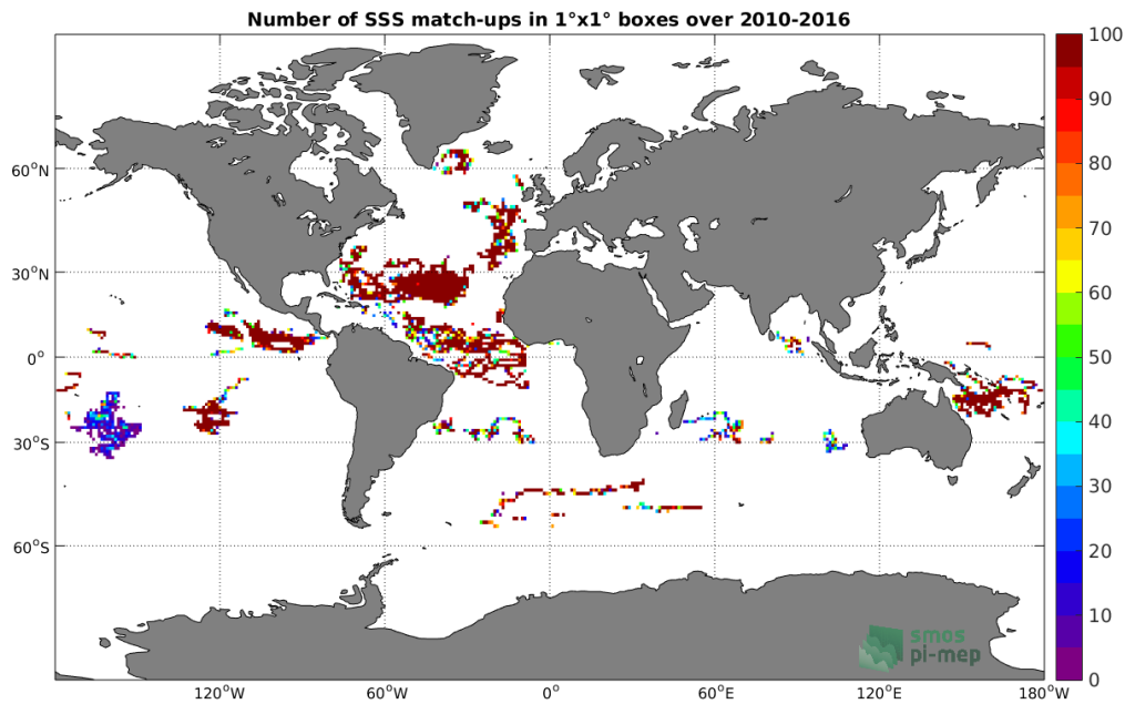
Figure 3: Number of SSS match-ups between Surface drifters SSS and the SMOS-L3-ICDC-V3-MONTHLY-0.5DEG SSS product for the Global Ocean Pi-MEP region over 1^\circ \times 1^\circ boxes and for the full satellite product period.
