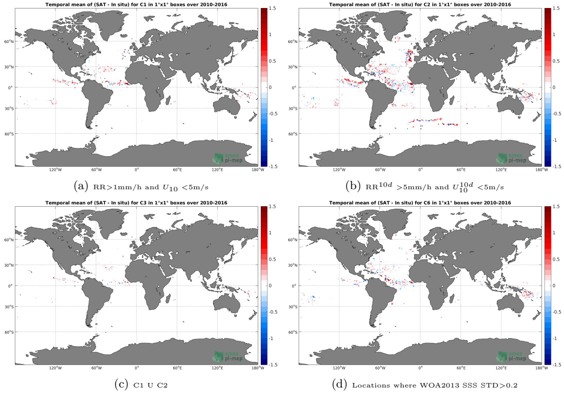
Figure 11: Temporal mean gridded over spatial boxes of size 1^\circ \times 1^\circ of \Delta SSS (SMOS-L3-ICDC-V3-MONTHLY-0.5DEG - Surface drifters) for 4 different subdatasets corresponding to: RR > 1\text{mm/h} and U_{10} < 5\text{m/s} (a), RR^{10d} > 5\text{mm/h} and U_{10}^{10d} < 5\text{m/s} (b), C1 U C2 (c), Locations where WOA2013 SSS STD > 0.2 (d).
