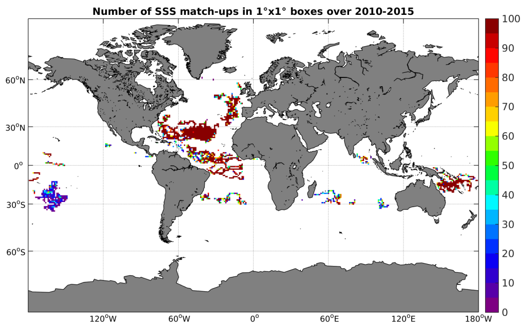
Figure 3: Number of SSS match-ups between Surface drifters SSS and the SMOS-L3-ICDC-V3-MONTHLY-0.5DEG SSS product for the Global Ocean Pi-MEP region over 1°x1° boxes and for the full satellite product period.
