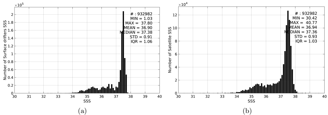
Figure 2: Histograms of SSS from Surface drifters (a) and SMOS-L3-ICDC-V3-MONTHLY-0.5DEG (b) considering all match-up pairs per bins of 0.1 over the Global Ocean Pi-MEP region and for the full satellite product period.
