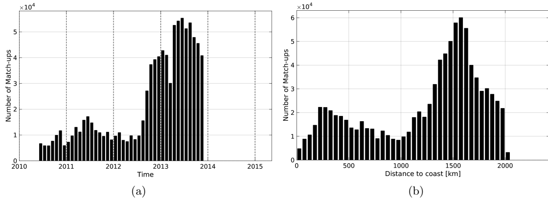
Figure 1: Number of match-ups between Surface drifters and SMOS-L3-ICDC-V3-MONTHLY-0.5DEG SSS as a function of time (a) and as function of the distance to coast (b) over the Global Ocean Pi-MEP region and for the full satellite product period.
