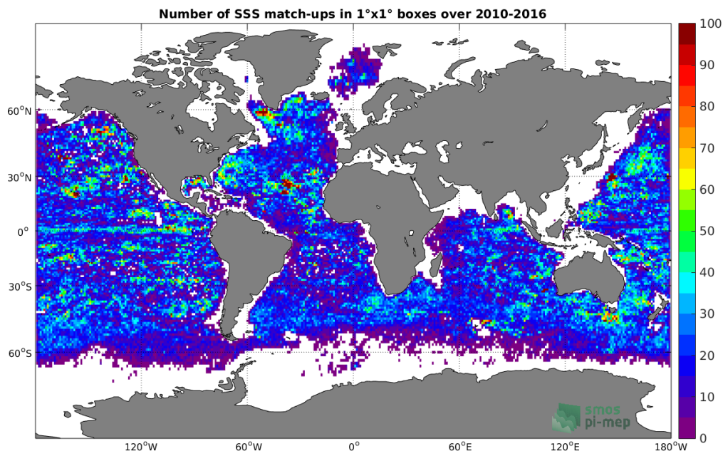
Figure 4: Number of SSS match-ups between Argo SSS and the SMOS SSS L3 v3 Monthly (ICDC) SSS product for the Global Ocean Pi-MEP region over 1^\circ \times 1^\circ boxes and for the full satellite product period.
