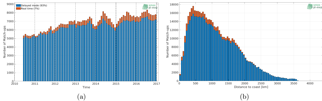
Figure 1: Number of match-ups between Argo and SMOS SSS L3 v3 Monthly (ICDC) SSS as a function of time (a) and as function of the distance to coast (b) over the Global Ocean Pi-MEP region and for the full satellite product period.
