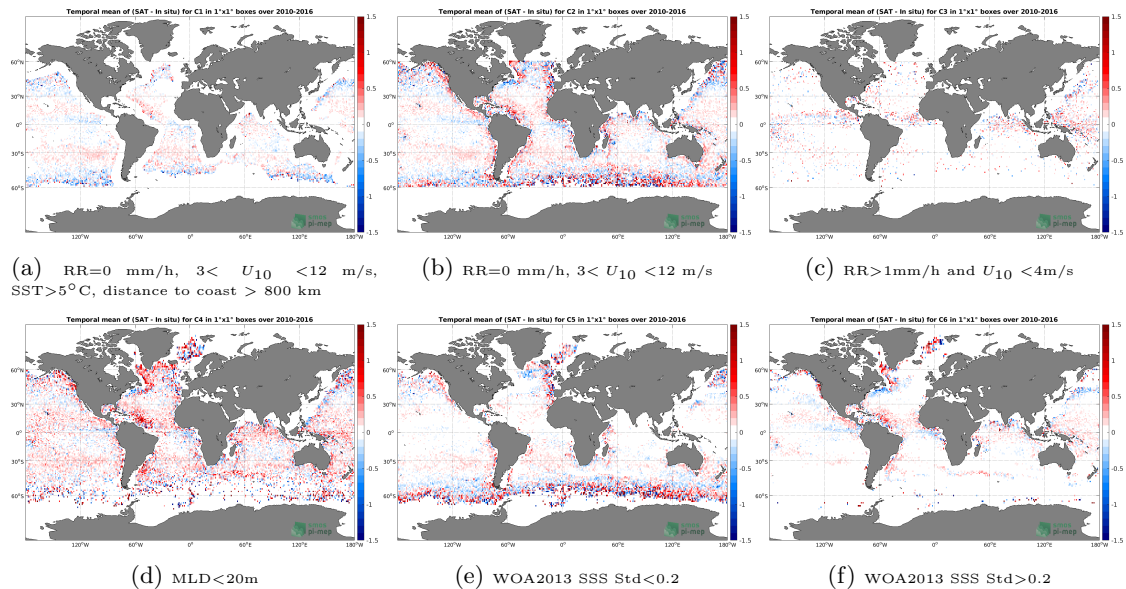
Figure 12: Temporal mean gridded over spatial boxes of size 1^\circ \times 1^\circ of \Delta SSS (SMOS SSS L3 v3 Monthly (ICDC) - Argo) for 6 different subdatasets corresponding to:RR=0 mm/h, 3 < U_{10} < 12 m/s, SST >5^\circ\text{C} , distance to coast > 800 km (a), RR=0 mm/h, 3 < U_{10} < 12 m/s (b), RR >1 mm/h and U_{10} < 4 m/s (c),MLD <20 m (d),WOA2013 SSS Std <0.2 (e),WOA2013 SSS Std >0.2 (f).
