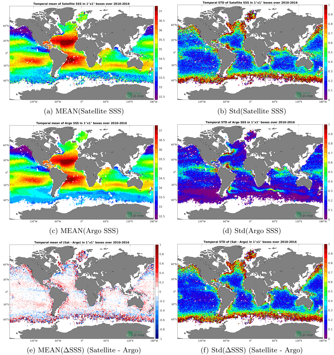
Figure 6: Temporal mean (left) and Std (right) of SSS from SMOS SSS L3 v3 Monthly (ICDC) (top), Argo (middle), and of \Delta SSS (Satellite - Argo). Only match-up pairs are used to generate these maps.
