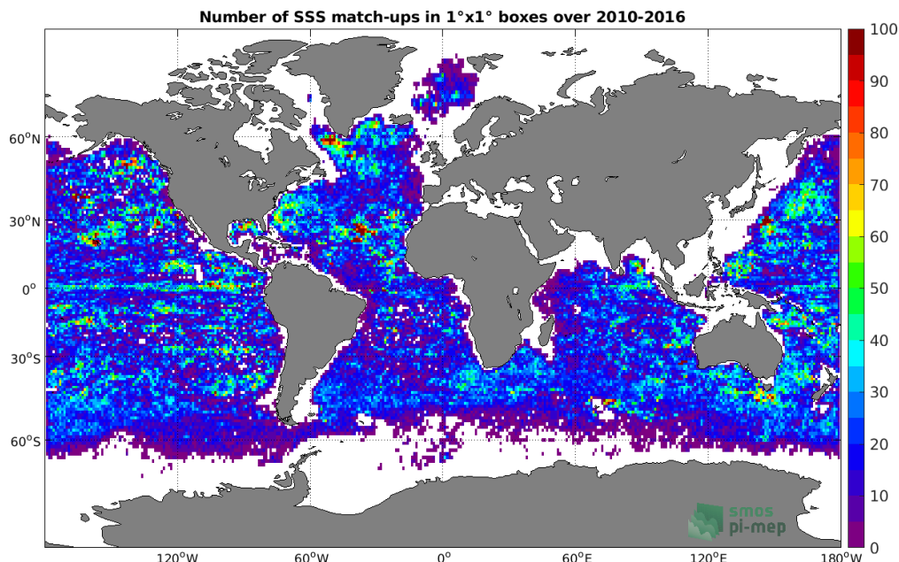
Figure 4: Number of SSS match-ups between Argo SSS and the SMOS SSS L3 v3 Monthly (ICDC) SSS product for the Global Ocean Pi-MEP region over 1°x1° boxes and for the full satellite product period.
