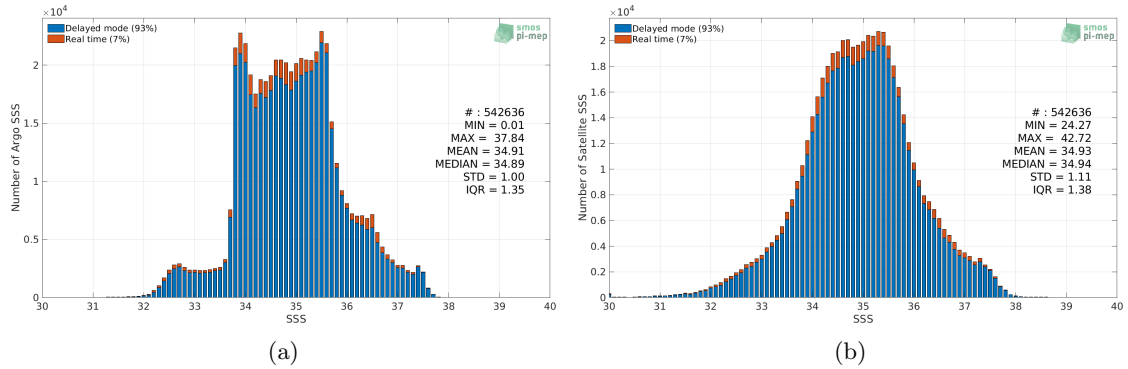
Figure 2: Histograms of SSS from Argo (a) and SMOS SSS L3 v3 Monthly (ICDC) (b) considering all match-up pairs per bins of 0.1 over the Global Ocean Pi-MEP region and for the full satellite product period.
