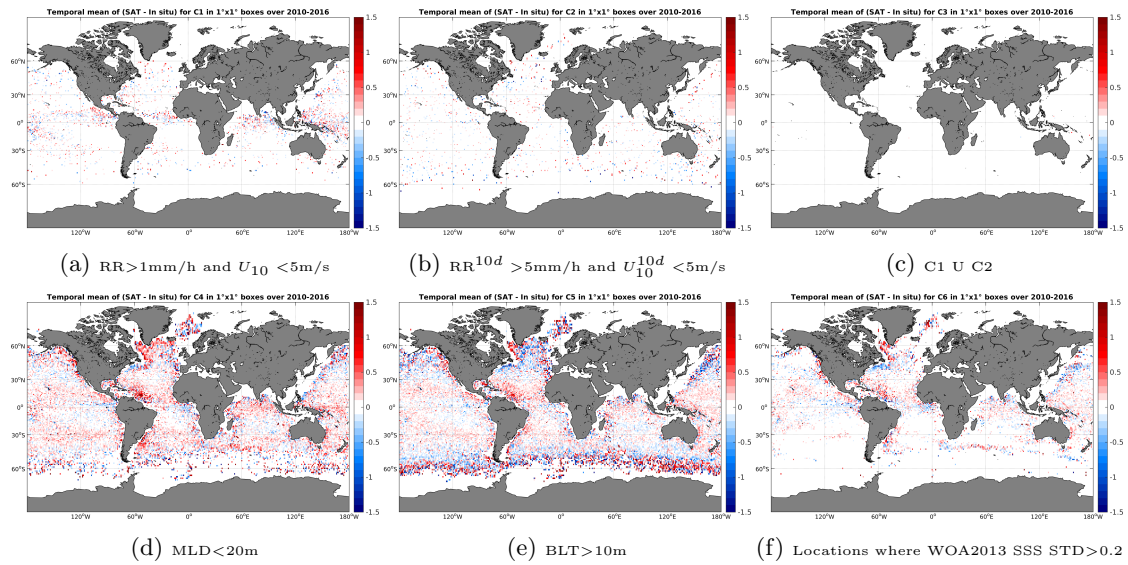
Figure 12: Temporal mean gridded over spatial boxes of size 1^\circ \times 1^\circ of \Delta SSS (SMOS-L3-ICDC-V3-MONTHLY-0.5DEG - Argo) for 6 different subdatasets corresponding to:RR>1mm/h and U_{10} < 5 m/s (a), RR^{10d} > 5 mm/h and U_{10}^{10d} < 5 m/s (b), C1 U C2 (c),MLD<20m (d),BLT>10m (e),Locations where WOA2013 SSS STD>0.2 (f).
