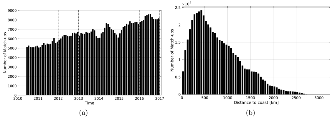
Figure 1: Number of match-ups between Argo and SMOS-L3-ICDC-V3-MONTHLY-0.5DEG SSS as a function of time (a) and as function of the distance to coast (b) over the Global Ocean Pi-MEP region and for the full satellite product period.
