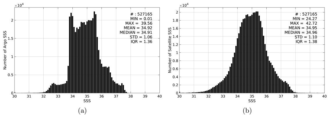
Figure 2: Histograms of SSS from Argo (a) and SMOS-L3-ICDC-V3-MONTHLY-0.5DEG (b) considering all match-up pairs per bins of 0.1 over the Global Ocean Pi-MEP region and for the full satellite product period.
