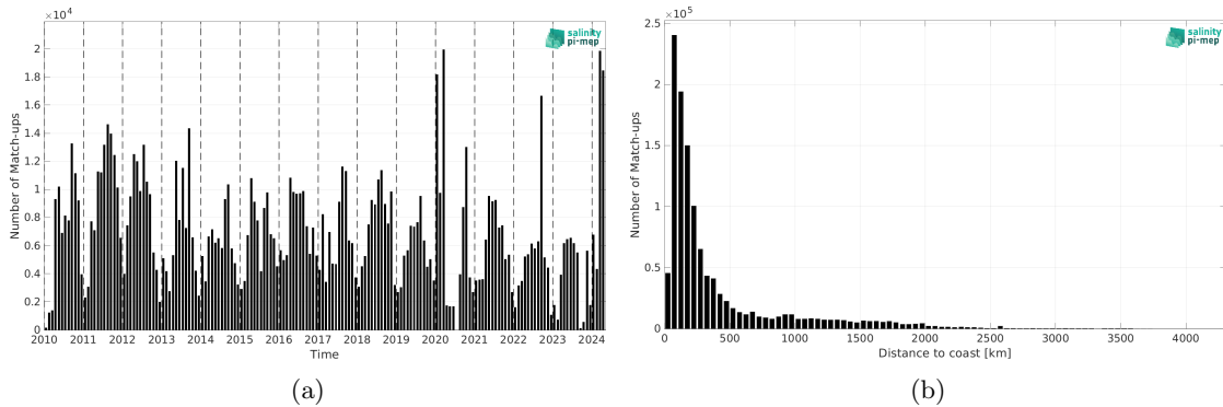
Figure 2: Number of match-ups between TSG (SAMOS) and SMOS SSS L2Q v331 - With FLAG (CMEMS-CATDS-CPDC) SSS as a function of time (a) and as function of the distance to coast (b) over the Global Ocean Pi-MEP region and for the full satellite product period.
