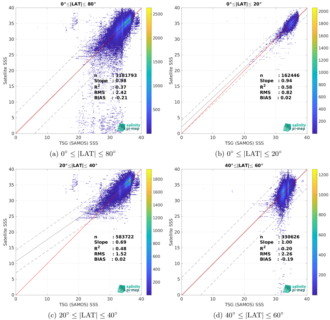
Figure 10: Contour maps of the concentration of SMOS SSS L2Q v331 - With FLAG (CMEMS-CATDS-CPDC) SSS (y-axis) versus TSG (SAMOS) SSS (x-axis) at match-up pairs for different latitude bands. For each plot, the red line shows x=y . The black thin and dashed lines indicate a linear fit through the data cloud and the \pm 95\% confidence levels, respectively. The number match-up pairs n , the slope and R^2 coefficient of the linear fit, the root mean square (RMS) and the mean bias between satellite and in situ data are indicated for each latitude band in each plots.
