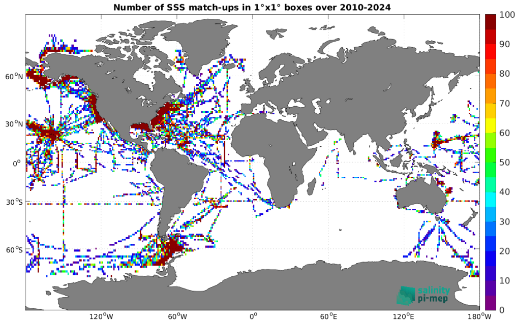
Figure 5: Number of SSS match-ups between TSG (SAMOS) SSS and the SMOS SSS L2Q v331 - With FLAG (CMEMS-CATDS-CPDC) SSS product for the Global Ocean Pi-MEP region over 1° × 1° boxes and for the full satellite product period.
