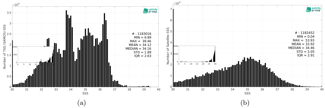
Figure 3: Histograms of SSS from TSG (SAMOS) (a) and SMOS SSS L2Q v331 - With FLAG (CMEMS-CATDS-CPDC) (b) considering all match-up pairs per bins of 0.1 over the Global Ocean Pi-MEP region and for the full satellite product period.
