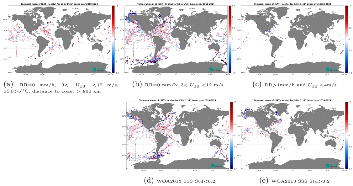
Figure 14: Temporal mean gridded over spatial boxes of size 1^\circ \times 1^\circ of \Delta\text{SSS} (SMOS SSS L2Q v331 - With FLAG (CMEMS-CATDS-CPDC) - TSG (SAMOS)) for 5 different subdatasets corresponding to:RR=0 mm/h, 3 < U_{10} < 12 m/s, SST > 5^\circ\text{C} , distance to coast > 800 km (a), RR=0 mm/h, 3 < U_{10} < 12 m/s (b), RR > 1 mm/h and U_{10} < 4 m/s (c), WOA2013 SSS Std < 0.2 (d), WOA2013 SSS Std > 0.2 (e).
