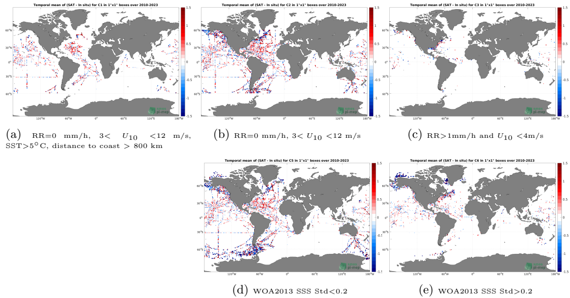
Figure 12: Temporal mean gridded over spatial boxes of size 1^\circ \times 1^\circ of \Delta\text{SSS} (SMOS SSS L2Q v331 - With FLAG (CMEMS-CATDS-CPDC) - TSG (SAMOS)) for 5 different subdatasets corresponding to:RR=0 mm/h, 3 < U_{10} < 12 m/s, SST >5^\circ\text{C} , distance to coast > 800 km (a), RR=0 mm/h, 3 < U_{10} < 12 m/s (b), RR >1 mm/h and U_{10} < 4 m/s (c), WOA2013 SSS Std <0.2 (d), WOA2013 SSS Std >0.2 (e).
