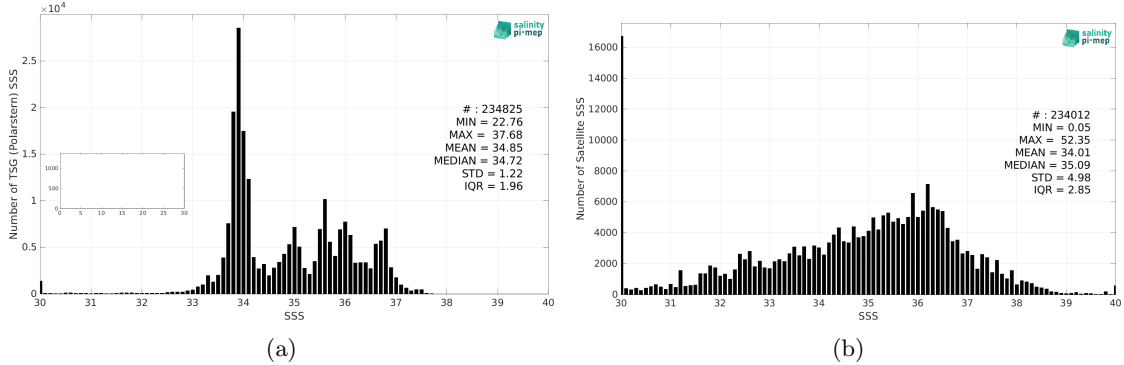
Figure 2: Histograms of SSS from TSG (Polarstern) (a) and SMOS SSS L2Q v331 - With FLAG (CMEMS-CATDS-CPDC) (b) considering all match-up pairs per bins of 0.1 over the Global Ocean Pi-MEP region and for the full satellite product period.
