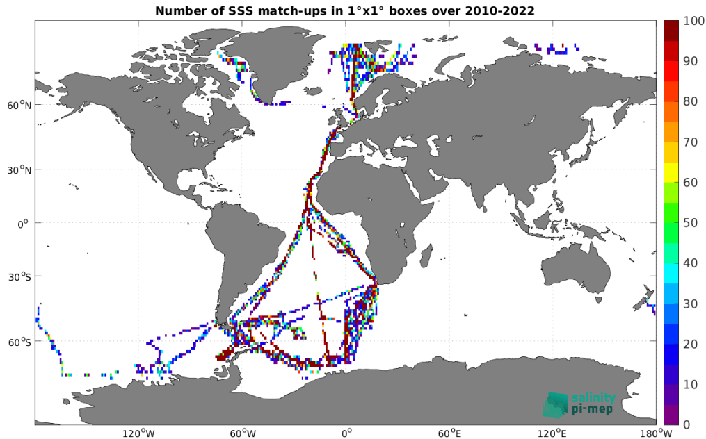
Figure 4: Number of SSS match-ups between TSG (Polarstern) SSS and the SMOS SSS L2Q v331 - With FLAG (CMEMS-CATDS-CPDC) SSS product for the Global Ocean Pi-MEP region over 1^\circ \times 1^\circ boxes and for the full satellite product period.
