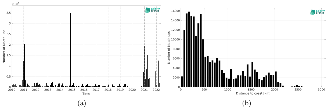
Figure 1: Number of match-ups between TSG (Polarstern) and SMOS SSS L2Q v331 - With FLAG (CMEMS-CATDS-CPDC) SSS as a function of time (a) and as function of the distance to coast (b) over the Global Ocean Pi-MEP region and for the full satellite product period.
