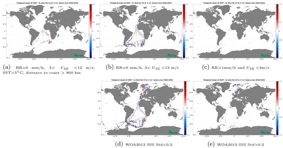
Figure 12: Temporal mean gridded over spatial boxes of size 1^\circ \times 1^\circ of \Delta SSS (SMOS SSS L2Q v331 - With FLAG (CMEMS-CATDS-CPDC) - TSG (Polarstern)) for 5 different subdatasets corresponding to: RR=0 mm/h, 3 < U_{10} < 12 m/s, SST > 5^\circ\text{C} , distance to coast > 800 km (a), RR=0 mm/h, 3 < U_{10} < 12 m/s (b), RR > 1 mm/h and U_{10} < 4 m/s (c), WOA2013 SSS Std < 0.2 (d), WOA2013 SSS Std > 0.2 (e).
