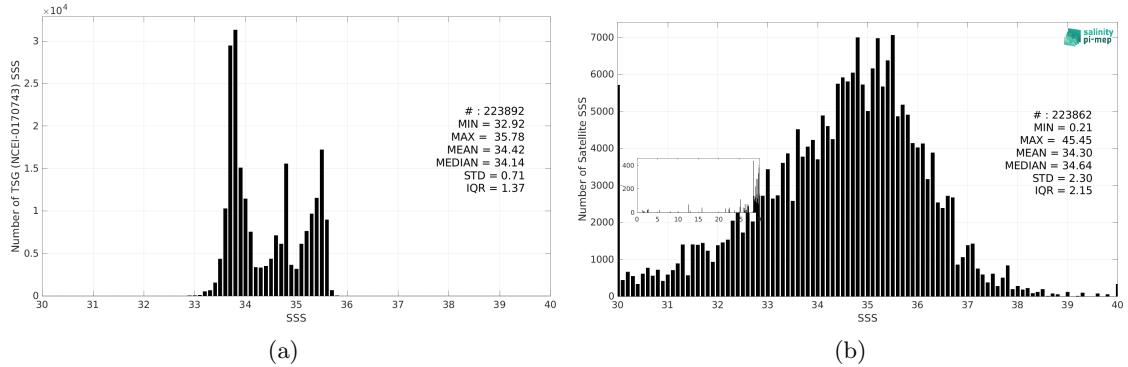
Figure 3: Histograms of SSS from TSG (NCEI-0170743) (a) and SMOS SSS L2Q v331 - With FLAG (CMEMS-CATDS-CPDC) (b) considering all match-up pairs per bins of 0.1 over the Global Ocean Pi-MEP region and for the full satellite product period.
