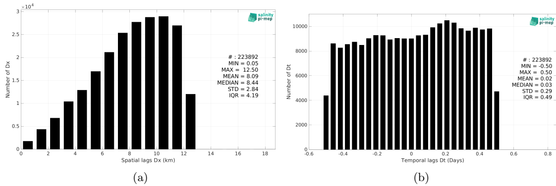
Figure 6: Histograms of the spatial (a) and temporal (b) lags between the location/time of the TSG (NCEI-0170743) measurement and the date of the corresponding SMOS SSS L2Q v331 - With FLAG (CMEMS-CATDS-CPDC) SSS pixel.
