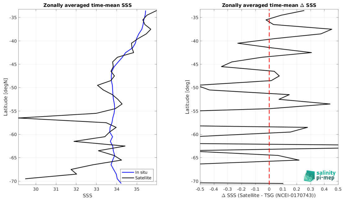
Figure 9: Left panel: Zonal mean SSS from SMOS SSS L2Q v331 - With FLAG (CMEMS-CATDS-CPDC) satellite product (black) and from TSG (NCEI-0170743) (blue). Right panel: Zonal mean of \Delta SSS (Satellite - TSG (NCEI-0170743)) for all the collected Pi-MEP match-up pairs estimated over the full satellite product period.
