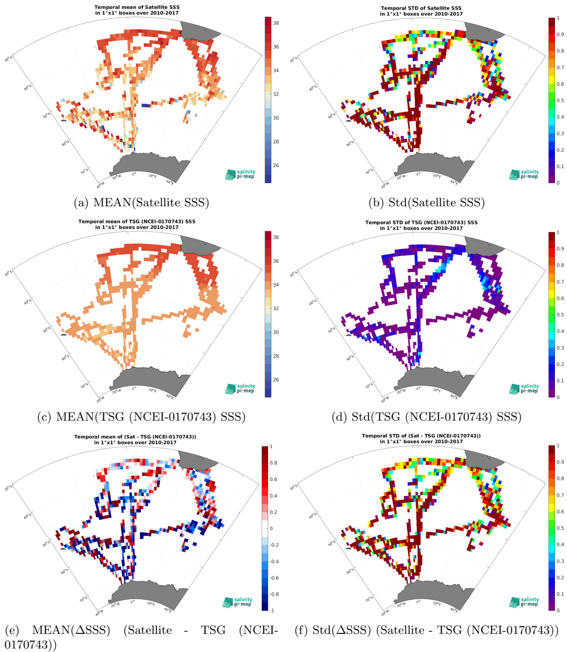
Figure 7: Temporal mean (left) and Std (right) of SSS from SMOS SSS L2Q v331 - With FLAG (CMEMS-CATDS-CPDC) (top), TSG (NCEI-0170743) (middle), and of \Delta SSS (Satellite - TSG (NCEI-0170743)). Only match-up pairs are used to generate these maps.
