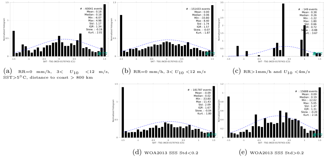
Figure 15: Normalized histogram of \Delta SSS (SMOS SSS L2Q v331 - With FLAG (CMEMS-CATDS-CPDC) - TSG (NCEI-0170743)) for 5 different subdatasets corresponding to: RR=0 mm/h, 3 < U_{10} < 12 m/s, SST>5°C, distance to coast > 800 km (a), RR=0 mm/h, 3 < U_{10} < 12 m/s (b), RR>1mm/h and U_{10} < 4 m/s (c), WOA2013 SSS Std<0.2 (d), WOA2013 SSS Std>0.2 (e).
