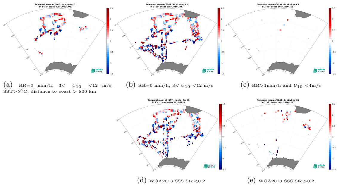
Figure 14: Temporal mean gridded over spatial boxes of size 1^\circ \times 1^\circ of \Delta SSS (SMOS SSS L2Q v331 - With FLAG (CMEMS-CATDS-CPDC) - TSG (NCEI-0170743)) for 5 different subdatasets corresponding to:RR=0 mm/h, 3 < U_{10} < 12 m/s, SST >5^\circ\text{C} , distance to coast > 800 km (a), RR=0 mm/h, 3 < U_{10} < 12 m/s (b), RR >1 mm/h and U_{10} < 4 m/s (c), WOA2013 SSS Std <0.2 (d), WOA2013 SSS Std >0.2 (e).
