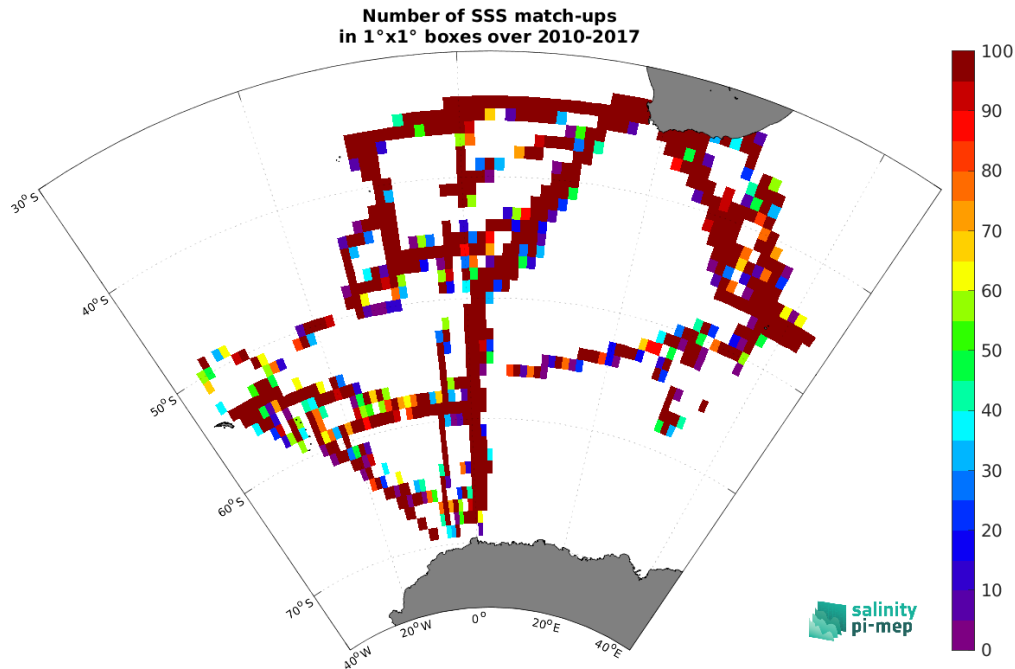
Figure 4: Number of SSS match-ups between TSG (NCEI-0170743) SSS and the SMOS SSS L2Q v331 - With FLAG (CMEMS-CATDS-CPDC) SSS product for the Global Ocean Pi-MEP region over 1^\circ \times 1^\circ boxes and for the full satellite product period.
