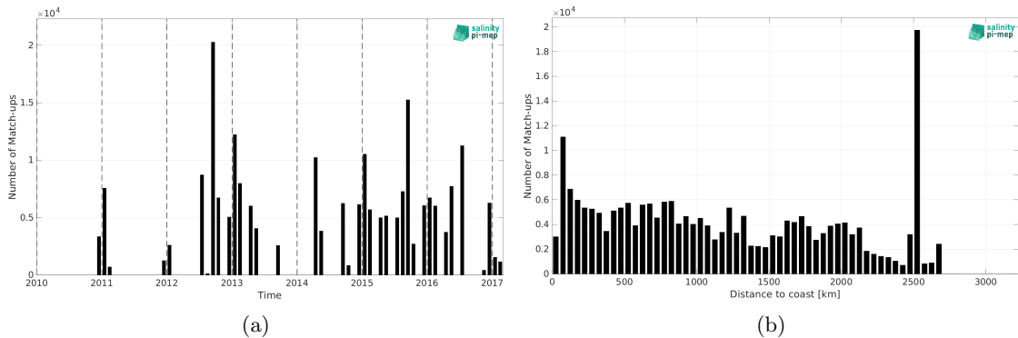
Figure 1: Number of match-ups between TSG (NCEI-0170743) and SMOS SSS L2Q v331 - With FLAG (CMEMS-CATDS-CPDC) SSS as a function of time (a) and as function of the distance to coast (b) over the Global Ocean Pi-MEP region and for the full satellite product period.
