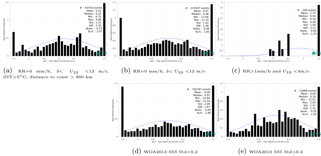
Figure 13: Normalized histogram of \Delta SSS (SMOS SSS L2Q v331 - With FLAG (CMEMS-CATDS-CPDC) - TSG (NCEI-0170743)) for 5 different subdatasets corresponding to: RR=0 mm/h, 3 < U_{10} < 12 m/s, SST>5°C, distance to coast > 800 km (a), RR=0 mm/h, 3 < U_{10} < 12 m/s (b), RR>1mm/h and U_{10} < 4 m/s (c), WOA2013 SSS Std<0.2 (d), WOA2013 SSS Std>0.2 (e).
