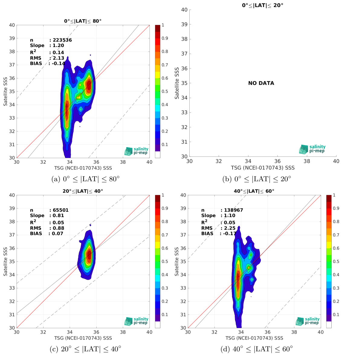
Figure 9: Contour maps of the concentration of SMOS SSS L2Q v331 - With FLAG (CMEMS-CATDS-CPDC) SSS (y-axis) versus TSG (NCEI-0170743) SSS (x-axis) at match-up pairs for different latitude bands. For each plot, the red line shows x=y . The black thin and dashed lines indicate a linear fit through the data cloud and the \pm 95\% confidence levels, respectively. The number match-up pairs n , the slope and R^2 coefficient of the linear fit, the root mean square (RMS) and the mean bias between satellite and in situ data are indicated for each latitude band in each plots.
