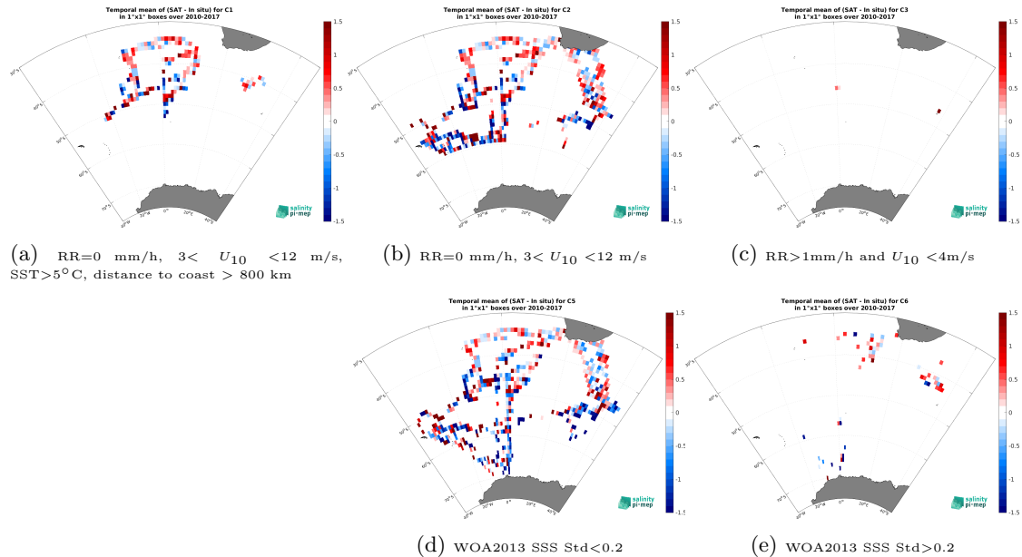
Figure 12: Temporal mean gridded over spatial boxes of size 1^{\circ}\times 1^{\circ} of \Delta\text{SSS} (SMOS SSS L2Q v331 - With FLAG (CMEMS-CATDS-CPDC) - TSG (NCEI-0170743)) for 5 different subdatasets corresponding to:RR=0 mm/h, 3 < U_{10} < 12 m/s, SST >5^{\circ}\text{C} , distance to coast > 800 km (a), RR=0 mm/h, 3 < U_{10} < 12 m/s (b), RR >1 mm/h and U_{10} < 4 m/s (c), WOA2013 SSS Std <0.2 (d), WOA2013 SSS Std >0.2 (e).
