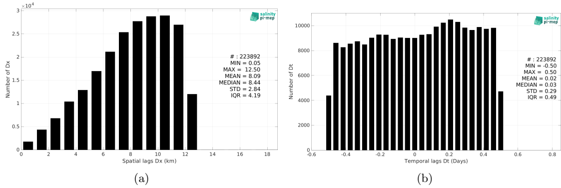
Figure 5: Histograms of the spatial (a) and temporal (b) lags between the location/time of the TSG (NCEI-0170743) measurement and the date of the corresponding SMOS SSS L2Q v331 - With FLAG (CMEMS-CATDS-CPDC) SSS pixel.
