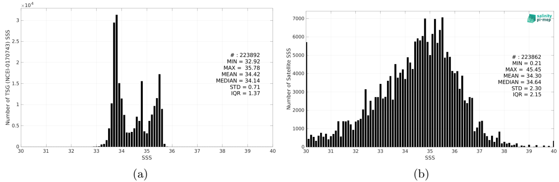
Figure 2: Histograms of SSS from TSG (NCEI-0170743) (a) and SMOS SSS L2Q v331 - With FLAG (CMEMS-CATDS-CPDC) (b) considering all match-up pairs per bins of 0.1 over the Global Ocean Pi-MEP region and for the full satellite product period.
