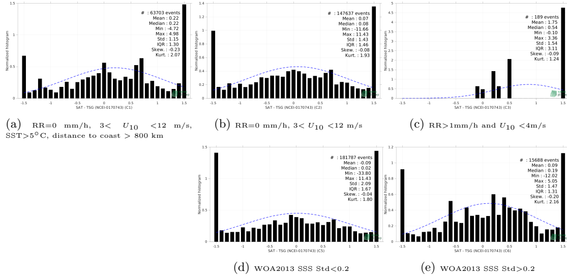
Figure 13: Normalized histogram of \Delta\text{SSS} (SMOS SSS L2Q v331 - With FLAG (CMEMS-CATDS-CPDC) - TSG (NCEI-0170743)) for 5 different subdatasets corresponding to: RR=0 mm/h, 3 < U_{10} < 12 m/s, SST>5°C, distance to coast > 800 km (a), RR=0 mm/h, 3 < U_{10} < 12 m/s (b), RR>1mm/h and U_{10} < 4 m/s (c), WOA2013 SSS Std<0.2 (d), WOA2013 SSS Std>0.2 (e).
