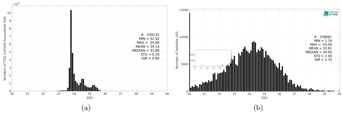
Figure 3: Histograms of SSS from TSG (LEGOS-Survostral) (a) and SMOS SSS L2Q v331 - With FLAG (CMEMS-CATDS-CPDC) (b) considering all match-up pairs per bins of 0.1 over the Global Ocean Pi-MEP region and for the full satellite product period.
