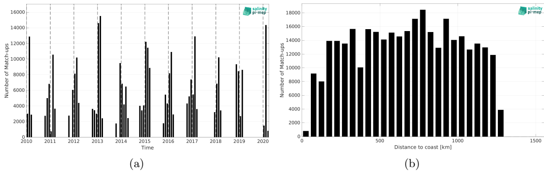
Figure 2: Number of match-ups between TSG (LEGOS-Survostral) and SMOS SSS L2Q v331 - With FLAG (CMEMS-CATDS-CPDC) SSS as a function of time (a) and as function of the distance to coast (b) over the Global Ocean Pi-MEP region and for the full satellite product period.
