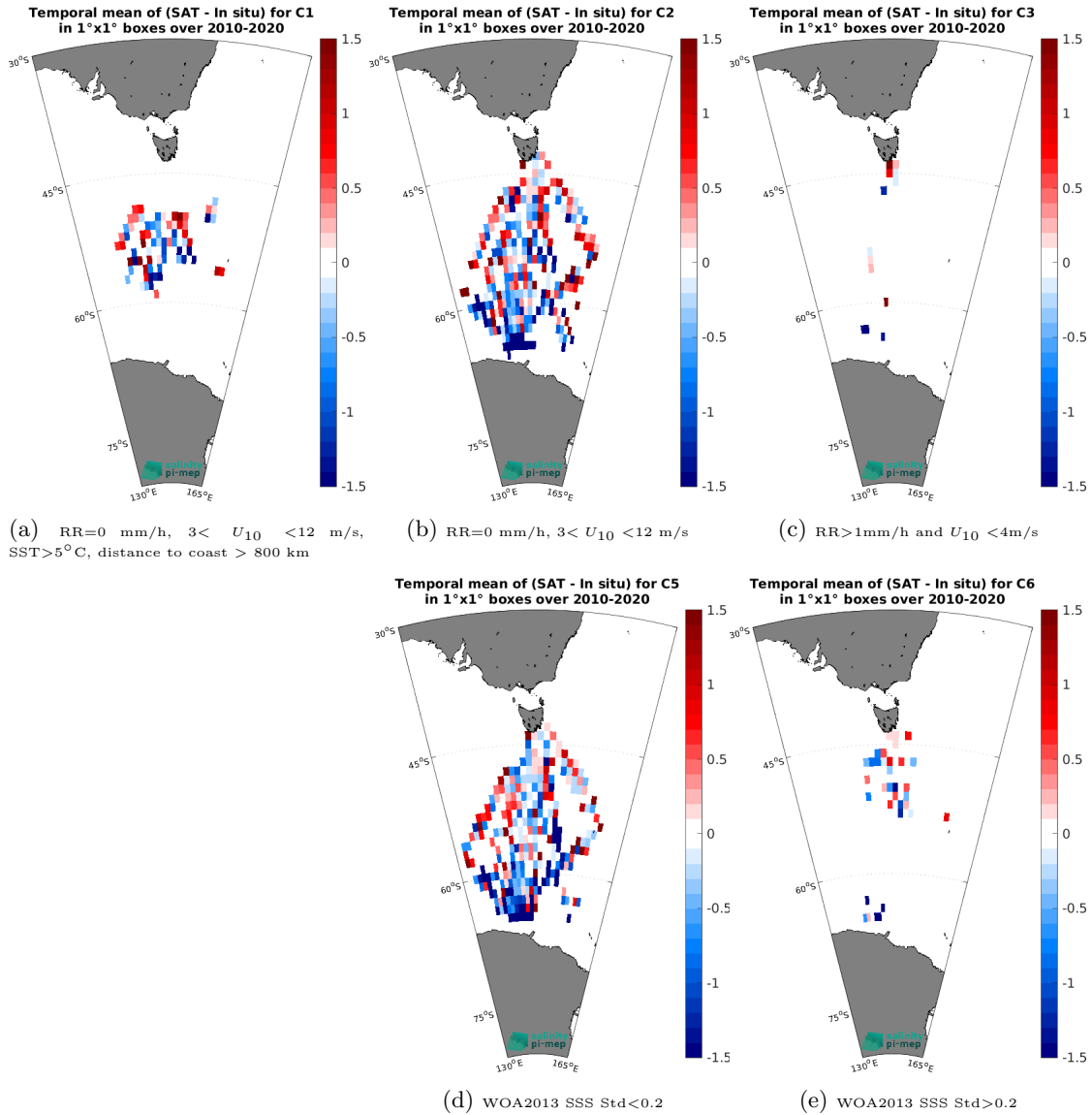
Figure 14: Temporal mean gridded over spatial boxes of size 1^\circ \times 1^\circ of \Delta SSS (SMOS SSS L2Q v331 - With FLAG (CMEMS-CATDS-CPDC) - TSG (LEGOS-Survostral)) for 5 different sub-datasets corresponding to: RR=0 mm/h, 3 < U_{10} < 12 m/s, SST>5°C, distance to coast > 800 km (a), RR=0 mm/h, 3 < U_{10} < 12 m/s (b), RR>1mm/h and U_{10} < 4 m/s (c), WOA2013 SSS Std<0.2 (d), WOA2013 SSS Std>0.2 (e).
