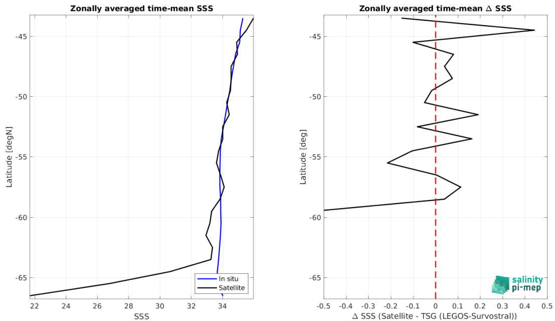
Figure 9: Left panel: Zonal mean SSS from SMOS SSS L2Q v331 - With FLAG (CMEMS-CATDS-CPDC) satellite product (black) and from TSG (LEGOS-Survostral) (blue). Right panel: Zonal mean of \Delta SSS (Satellite - TSG (LEGOS-Survostral)) for all the collected Pi-MEP match-up pairs estimated over the full satellite product period.
