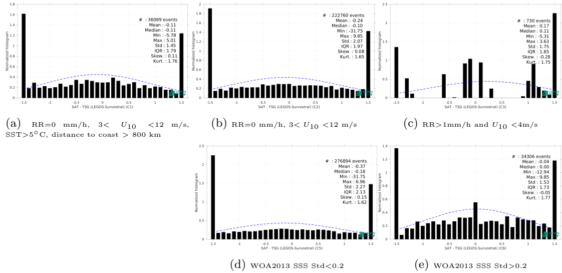
Figure 15: Normalized histogram of \Delta SSS (SMOS SSS L2Q v331 - With FLAG (CMEMS-CATDS-CPDC) - TSG (LEGOS-Survostral)) for 5 different subdatasets corresponding to: RR=0 mm/h, 3 < U_{10} < 12 m/s, SST>5°C, distance to coast > 800 km (a), RR=0 mm/h, 3 < U_{10} < 12 m/s (b), RR>1mm/h and U_{10} < 4 m/s (c), WOA2013 SSS Std<0.2 (d), WOA2013 SSS Std>0.2 (e).
