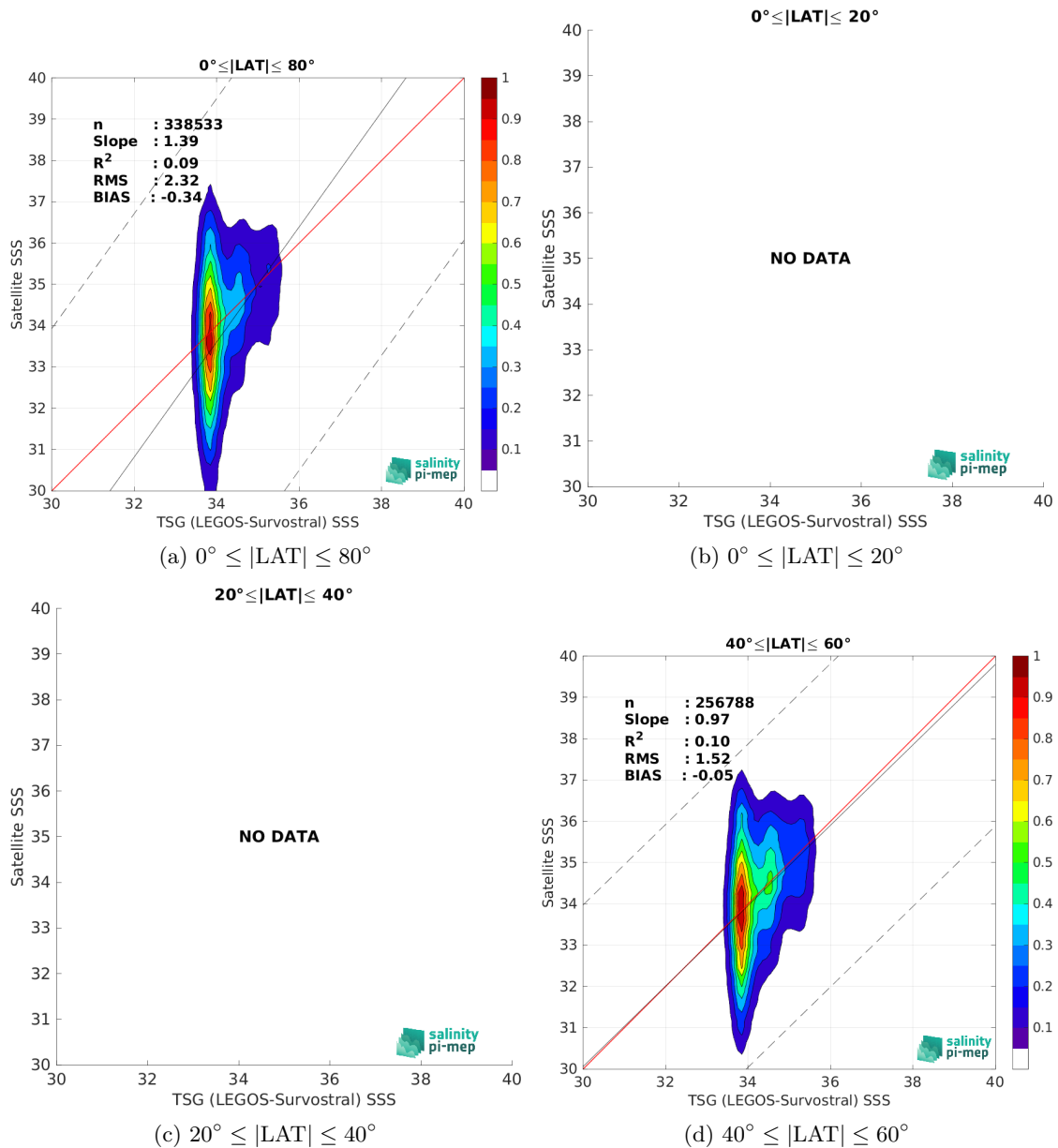
Figure 10: Contour maps of the concentration of SMOS SSS L2Q v331 - With FLAG (CMEMS-CATDS-CPDC) SSS (y-axis) versus TSG (LEGOS-Survostral) SSS (x-axis) at match-up pairs for different latitude bands. For each plot, the red line shows x=y . The black thin and dashed lines indicate a linear fit through the data cloud and the \pm 95\% confidence levels, respectively. The number match-up pairs n , the slope and R^2 coefficient of the linear fit, the root mean square (RMS) and the mean bias between satellite and in situ data are indicated for each latitude band in each plots.
