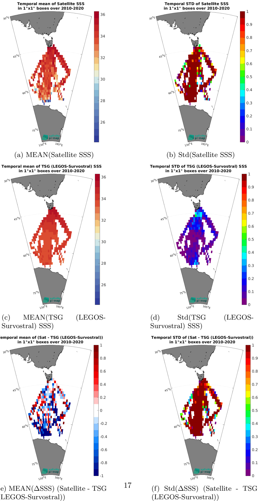
Figure 7: Temporal mean (left) and Std (right) of SSS from SMOS SSS L2Q v331 - With FLAG (CMEMS-CATDS-CPDC) (top), TSG (LEGOS-Survostral) (middle), and of \Delta SSS (Satellite - TSG (LEGOS-Survostral)). Only match-up pairs are used to generate these maps.
