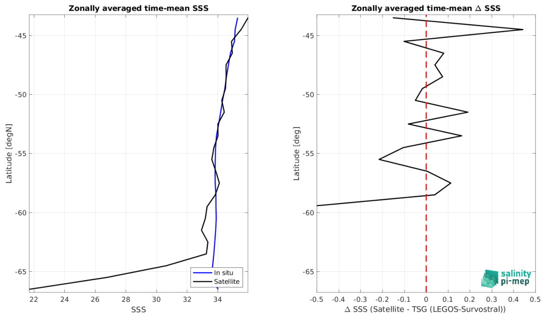
Figure 8: Left panel: Zonal mean SSS from SMOS SSS L2Q v331 - With FLAG (CMEMS-CATDS-CPDC) satellite product (black) and from TSG (LEGOS-Survostral) (blue). Right panel: Zonal mean of \Delta SSS (Satellite - TSG (LEGOS-Survostral)) for all the collected Pi-MEP match-up pairs estimated over the full satellite product period.
