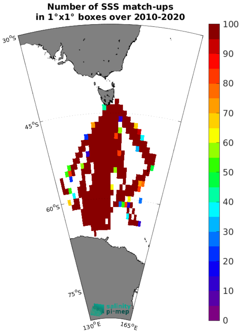
Figure 4: Number of SSS match-ups between TSG (LEGOS-Survostral) SSS and the SMOS SSS L2Q v331 - With FLAG (CMEMS-CATDS-CPDC) SSS product for the Global Ocean Pi-MEP region over 1°x1° boxes and for the full satellite product period.
