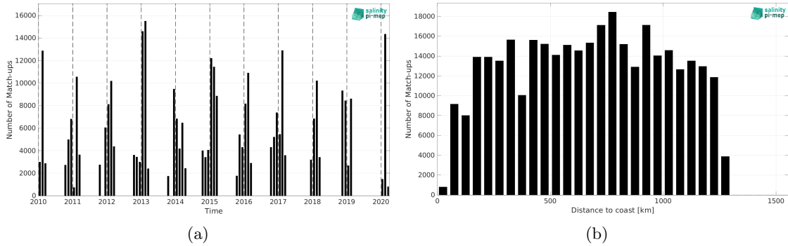
Figure 1: Number of match-ups between TSG (LEGOS-Survostral) and SMOS SSS L2Q v331 - With FLAG (CMEMS-CATDS-CPDC) SSS as a function of time (a) and as function of the distance to coast (b) over the Global Ocean Pi-MEP region and for the full satellite product period.
