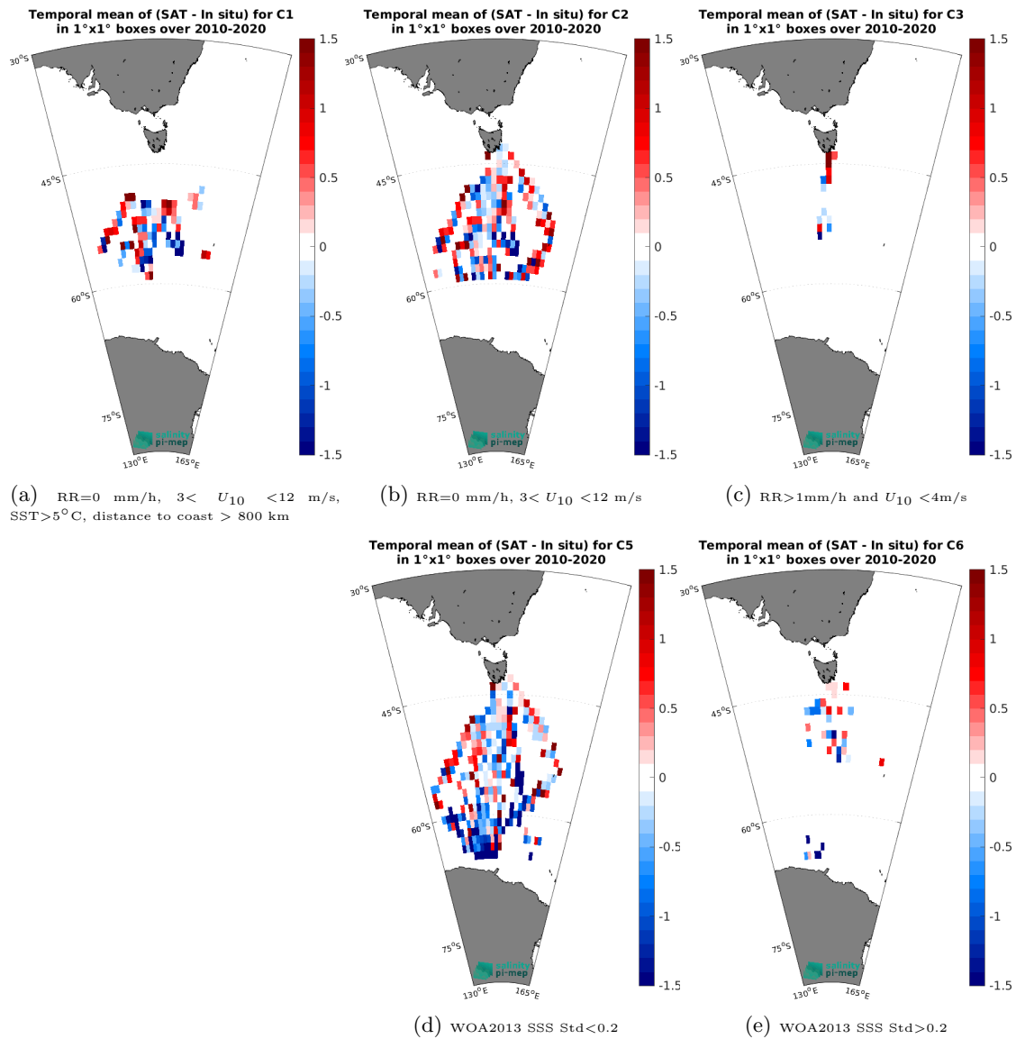
Figure 12: Temporal mean gridded over spatial boxes of size 1^\circ \times 1^\circ of \Delta SSS (SMOS SSS L2Q v331 - With FLAG (CMEMS-CATDS-CPDC) - TSG (LEGOS-Survostral)) for 5 different sub-datasets corresponding to: RR=0 mm/h, 3 < U_{10} < 12 m/s, SST>5°C, distance to coast > 800 km (a), RR=0 mm/h, 3 < U_{10} < 12 m/s (b), RR>1mm/h and U_{10} < 4 m/s (c), WOA2013 SSS Std<0.2 (d), WOA2013 SSS Std>0.2 (e).
