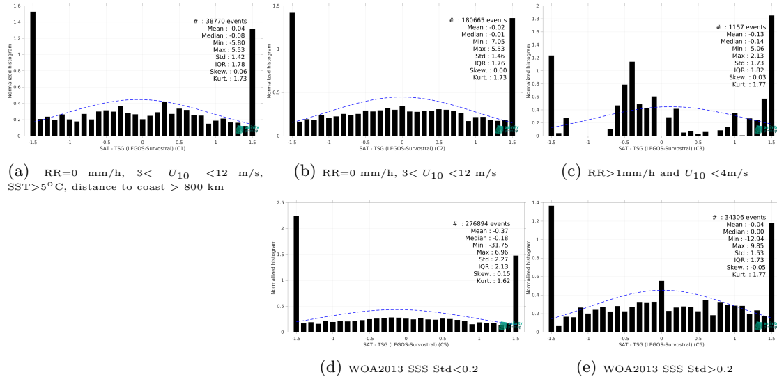
Figure 13: Normalized histogram of \Delta SSS (SMOS SSS L2Q v331 - With FLAG (CMEMS-CATDS-CPDC) - TSG (LEGOS-Survostral)) for 5 different subdatasets corresponding to: RR=0 mm/h, 3 < U_{10} < 12 m/s, SST>5°C, distance to coast > 800 km (a), RR=0 mm/h, 3 < U_{10} < 12 m/s (b), RR>1mm/h and U_{10} < 4 m/s (c), WOA2013 SSS Std<0.2 (d), WOA2013 SSS Std>0.2 (e).
