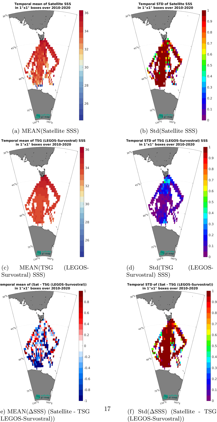
Figure 6: Temporal mean (left) and Std (right) of SSS from SMOS SSS L2Q v331 - With FLAG (CMEMS-CATDS-CPDC) (top), TSG (LEGOS-Survostral) (middle), and of \Delta SSS (Satellite - TSG (LEGOS-Survostral)). Only match-up pairs are used to generate these maps.
