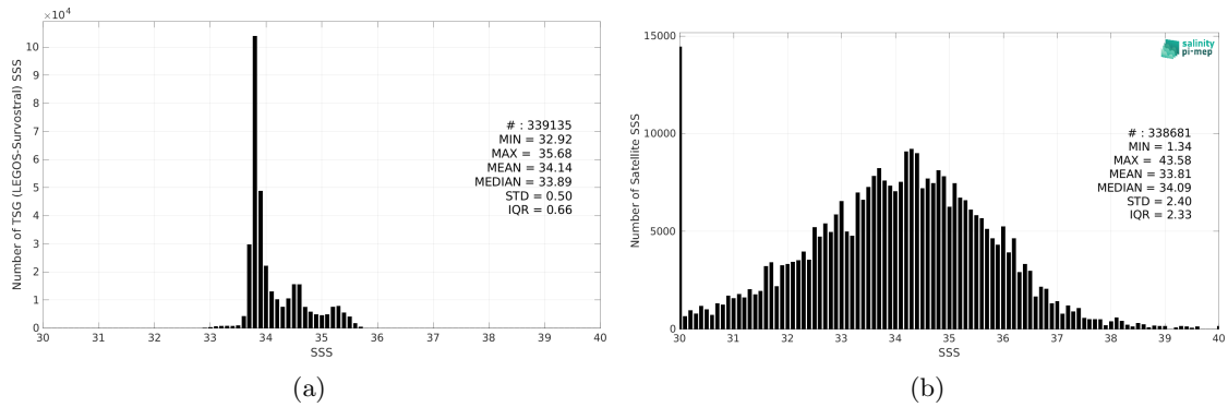
Figure 2: Histograms of SSS from TSG (LEGOS-Survostral) (a) and SMOS SSS L2Q v331 - With FLAG (CMEMS-CATDS-CPDC) (b) considering all match-up pairs per bins of 0.1 over the Global Ocean Pi-MEP region and for the full satellite product period.
