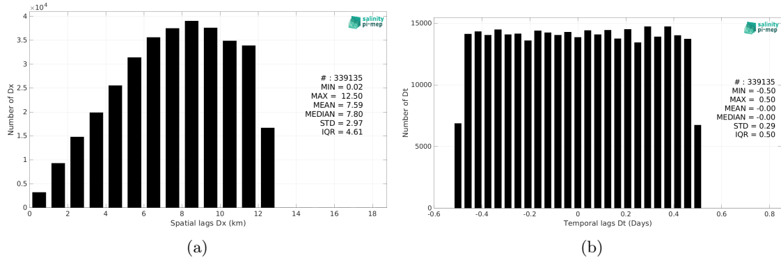
Figure 5: Histograms of the spatial (a) and temporal (b) lags between the location/time of the TSG (LEGOS-Survostral) measurement and the date of the corresponding SMOS SSS L2Q v331 - With FLAG (CMEMS-CATDS-CPDC) SSS pixel.
