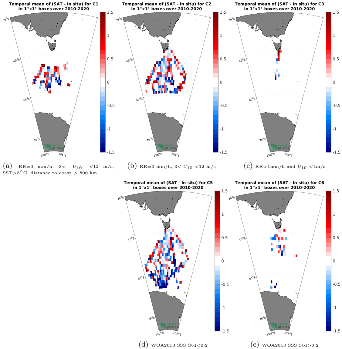
Figure 12: Temporal mean gridded over spatial boxes of size 1°x1° of \Delta SSS (SMOS SSS L2Q v331 - With FLAG (CMEMS-CATDS-CPDC) - TSG (LEGOS-Survostral)) for 5 different sub-datasets corresponding to:RR=0 mm/h, 3 < U_{10} < 12 m/s, SST>5°C, distance to coast > 800 km (a), RR=0 mm/h, 3 < U_{10} < 12 m/s (b), RR>1mm/h and U_{10} < 4 m/s (c), WOA2013 SSS Std<0.2 (d), WOA2013 SSS Std>0.2 (e).
