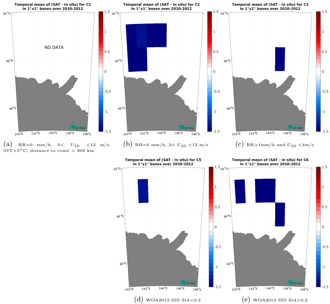
Figure 14: Temporal mean gridded over spatial boxes of size 1^{\circ} \times 1^{\circ} of \Delta SSS (SMOS SSS L2Q v331 - With FLAG (CMEMS-CATDS-CPDC) - TSG (LEGOS-Surv-Adel)) for 5 different sub-datasets corresponding to: RR=0 mm/h, 3 < U_{10} < 12 m/s, SST>5°C, distance to coast > 800 km (a), RR=0 mm/h, 3 < U_{10} < 12 m/s (b), RR>1mm/h and U_{10} < 4 m/s (c), WOA2013 SSS Std<0.2 (d), WOA2013 SSS Std>0.2 (e).
