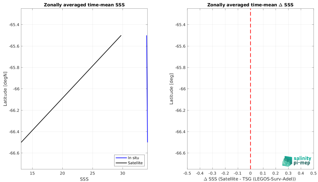
Figure 9: Left panel: Zonal mean SSS from SMOS SSS L2Q v331 - With FLAG (CMEMS-CATDS-CPDC) satellite product (black) and from TSG (LEGOS-Surv-Adel) (blue). Right panel: Zonal mean of \Delta SSS (Satellite - TSG (LEGOS-Surv-Adel)) for all the collected Pi-MEP match-up pairs estimated over the full satellite product period.
