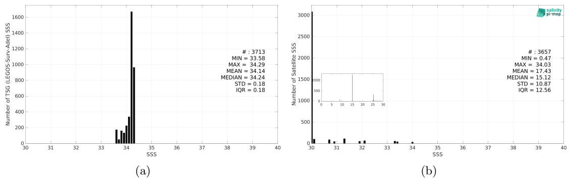
Figure 3: Histograms of SSS from TSG (LEGOS-Surv-Adel) (a) and SMOS SSS L2Q v331 - With FLAG (CMEMS-CATDS-CPDC) (b) considering all match-up pairs per bins of 0.1 over the Global Ocean Pi-MEP region and for the full satellite product period.
