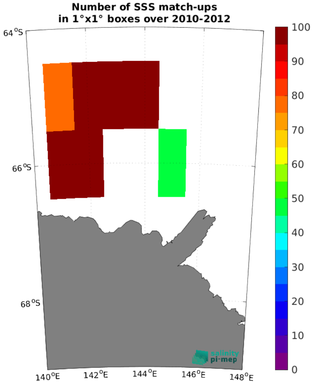
Figure 5: Number of SSS match-ups between TSG (LEGOS-Surv-Adel) SSS and the SMOS SSS L2Q v331 - With FLAG (CMEMS-CATDS-CPDC) SSS product for the Global Ocean Pi-MEP region over 1^\circ \times 1^\circ boxes and for the full satellite product period.
