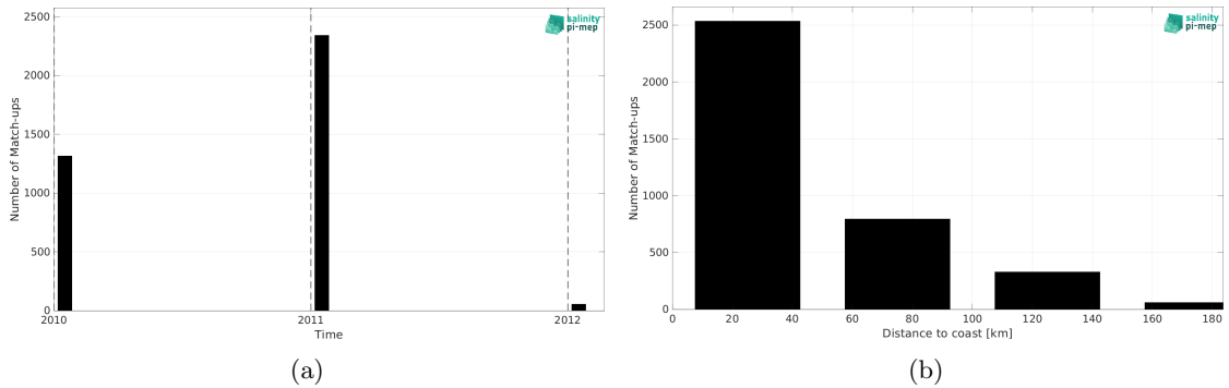
Figure 2: Number of match-ups between TSG (LEGOS-Surv-Adel) and SMOS SSS L2Q v331 - With FLAG (CMEMS-CATDS-CPDC) SSS as a function of time (a) and as function of the distance to coast (b) over the Global Ocean Pi-MEP region and for the full satellite product period.
