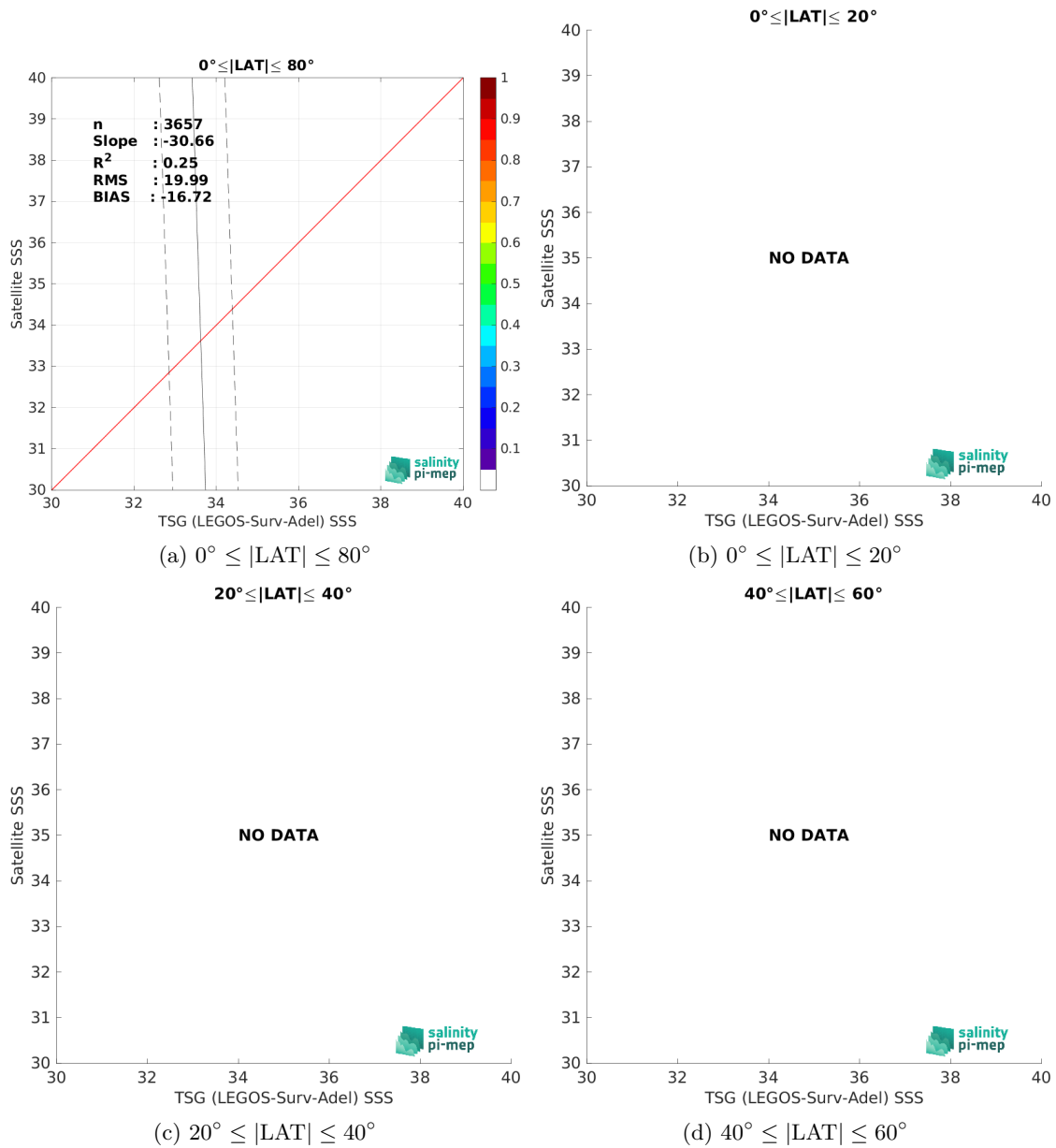
Figure 10: Contour maps of the concentration of SMOS SSS L2Q v331 - With FLAG (CMEMS-CATDS-CPDC) SSS (y-axis) versus TSG (LEGOS-Surv-Adel) SSS (x-axis) at match-up pairs for different latitude bands. For each plot, the red line shows x=y . The black thin and dashed lines indicate a linear fit through the data cloud and the \pm 95\% confidence levels, respectively. The number match-up pairs n , the slope and R^2 coefficient of the linear fit, the root mean square (RMS) and the mean bias between satellite and in situ data are indicated for each latitude band in each plots.
