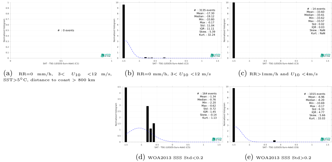
Figure 15: Normalized histogram of \Delta SSS (SMOS SSS L2Q v331 - With FLAG (CMEMS-CATDS-CPDC) - TSG (LEGOS-Surv-Adel)) for 5 different subdatasets corresponding to: RR=0 mm/h, 3 < U_{10} < 12 m/s, SST > 5°C, distance to coast > 800 km (a), RR=0 mm/h, 3 < U_{10} < 12 m/s (b), RR > 1mm/h and U_{10} < 4 m/s (c), WOA2013 SSS Std < 0.2 (d), WOA2013 SSS Std > 0.2 (e).
