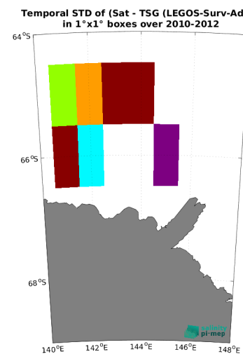
(f) Std( \Delta SSS) (Satellite - TSG (LEGOS-Surv-Adel))
