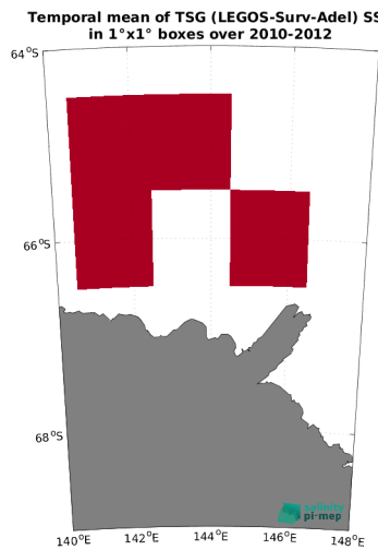
(c) MEAN(TSG (LEGOS-Surv-Adel) SSS)
