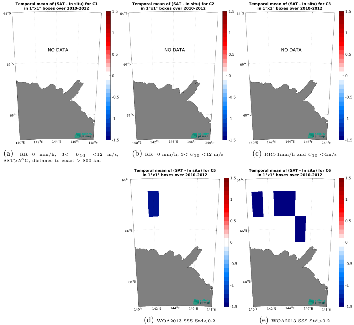
Figure 12: Temporal mean gridded over spatial boxes of size 1^\circ \times 1^\circ of \Delta SSS (SMOS SSS L2Q v331 - With FLAG (CMEMS-CATDS-CPDC) - TSG (LEGOS-Surv-Adel)) for 5 different sub-datasets corresponding to: RR=0 mm/h, 3 < U_{10} < 12 m/s, SST>5°C, distance to coast > 800 km (a), RR=0 mm/h, 3 < U_{10} < 12 m/s (b), RR>1mm/h and U_{10} < 4 m/s (c), WOA2013 SSS Std<0.2 (d), WOA2013 SSS Std>0.2 (e).
