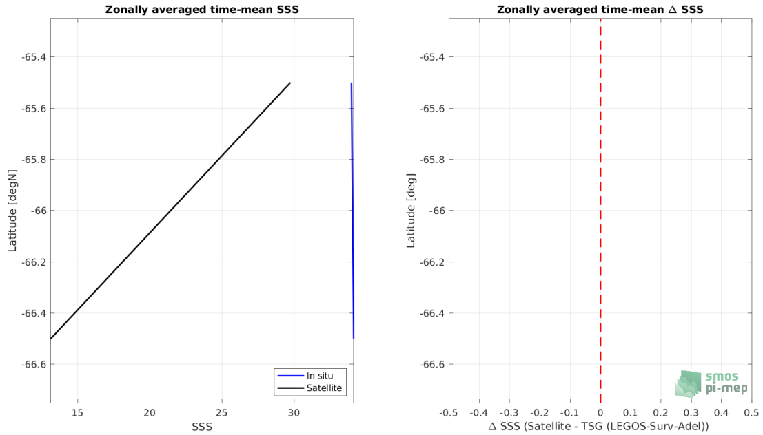
Figure 8: Left panel: Zonal mean SSS from SMOS SSS L2Q v331 - With FLAG (CMEMS-CATDS-CPDC) satellite product (black) and from TSG (LEGOS-Surv-Adel) (blue). Right panel: Zonal mean of \Delta SSS (Satellite - TSG (LEGOS-Surv-Adel)) for all the collected Pi-MEP match-up pairs estimated over the full satellite product period.
