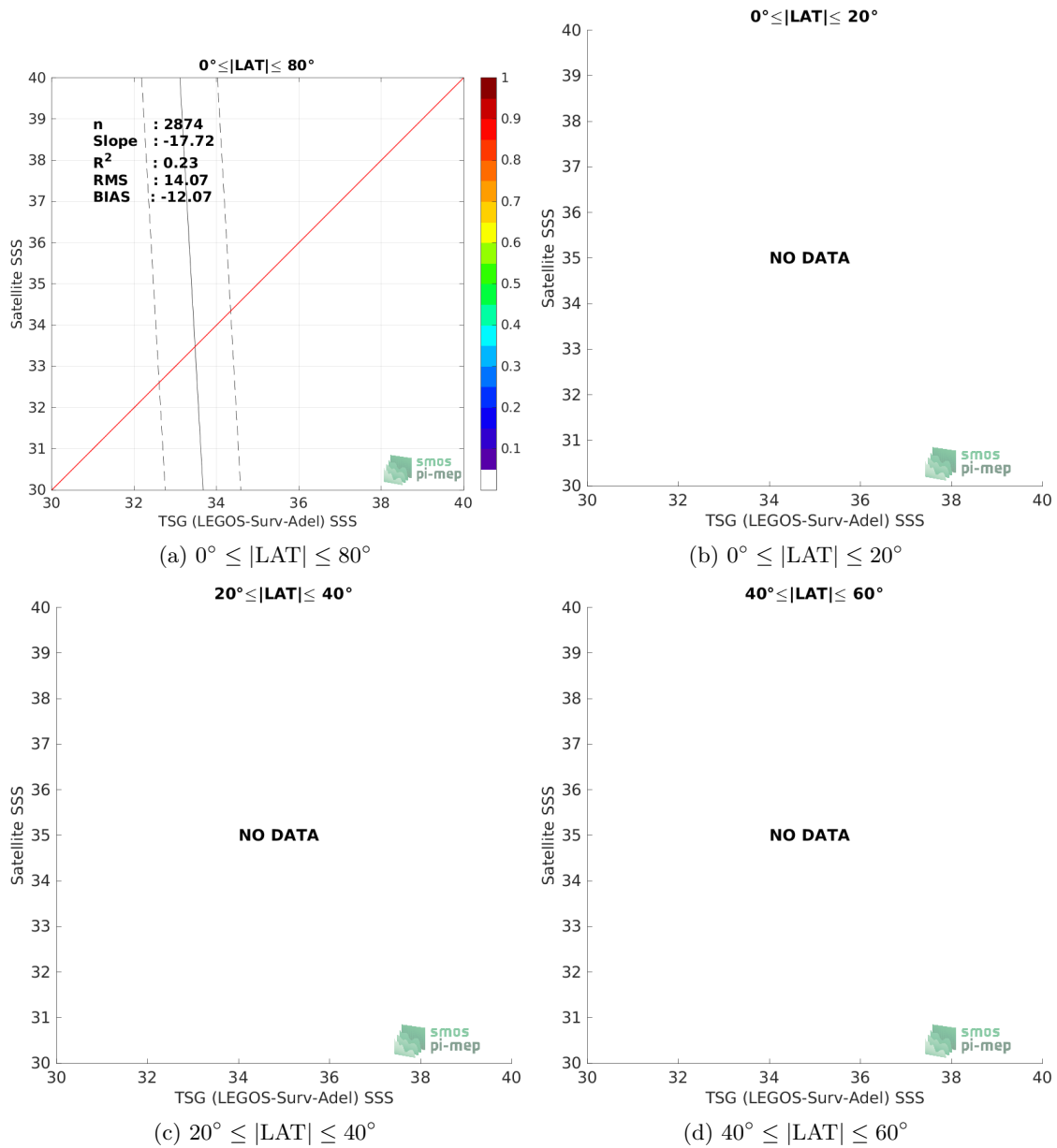
Figure 9: Contour maps of the concentration of SMOS SSS L2Q v331 - With FLAG (CMEMS-CATDS-CPDC) SSS (y-axis) versus TSG (LEGOS-Surv-Adel) SSS (x-axis) at match-up pairs for different latitude bands. For each plot, the red line shows x=y . The black thin and dashed lines indicate a linear fit through the data cloud and the \pm 95\% confidence levels, respectively. The number match-up pairs n , the slope and R^2 coefficient of the linear fit, the root mean square (RMS) and the mean bias between satellite and in situ data are indicated for each latitude band in each plots.
