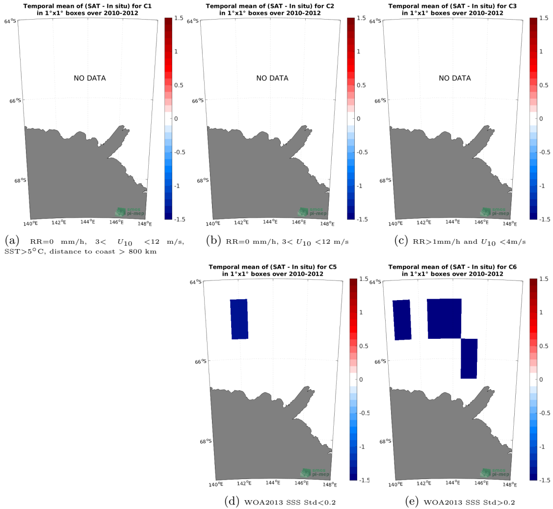
Figure 12: Temporal mean gridded over spatial boxes of size 1°x1° of \Delta SSS (SMOS SSS L2Q v331 - With FLAG (CMEMS-CATDS-CPDC) - TSG (LEGOS-Surv-Adel)) for 5 different sub-datasets corresponding to:RR=0 mm/h, 3 < U_{10} < 12 m/s, SST>5°C, distance to coast > 800 km (a), RR=0 mm/h, 3 < U_{10} < 12 m/s (b), RR>1mm/h and U_{10} < 4 m/s (c), WOA2013 SSS Std<0.2 (d), WOA2013 SSS Std>0.2 (e).
