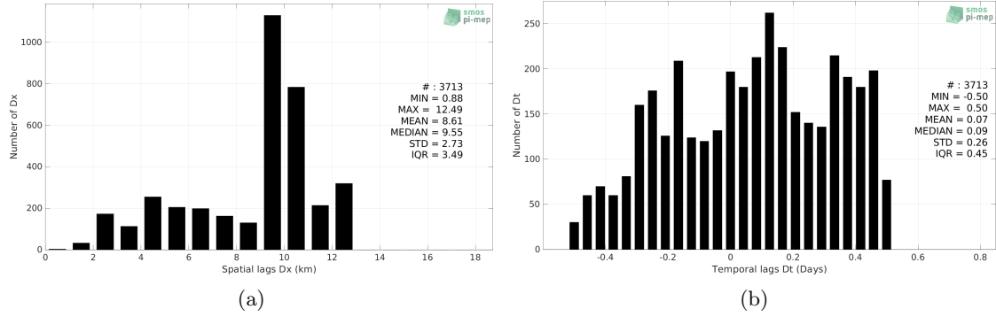
Figure 5: Histograms of the spatial (a) and temporal (b) lags between the location/time of the TSG (LEGOS-Surv-Adel) measurement and the date of the corresponding SMOS SSS L2Q v331 - With FLAG (CMEMS-CATDS-CPDC) SSS pixel.
