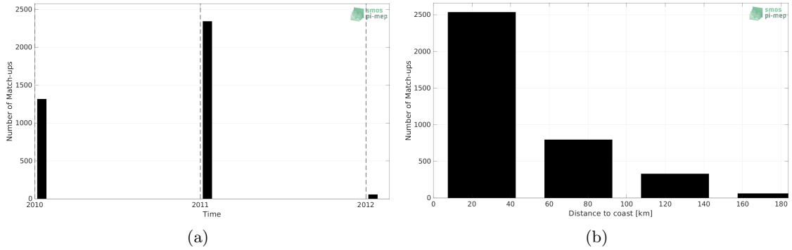
Figure 1: Number of match-ups between TSG (LEGOS-Surv-Adel) and SMOS SSS L2Q v331 - With FLAG (CMEMS-CATDS-CPDC) SSS as a function of time (a) and as function of the distance to coast (b) over the Global Ocean Pi-MEP region and for the full satellite product period.
