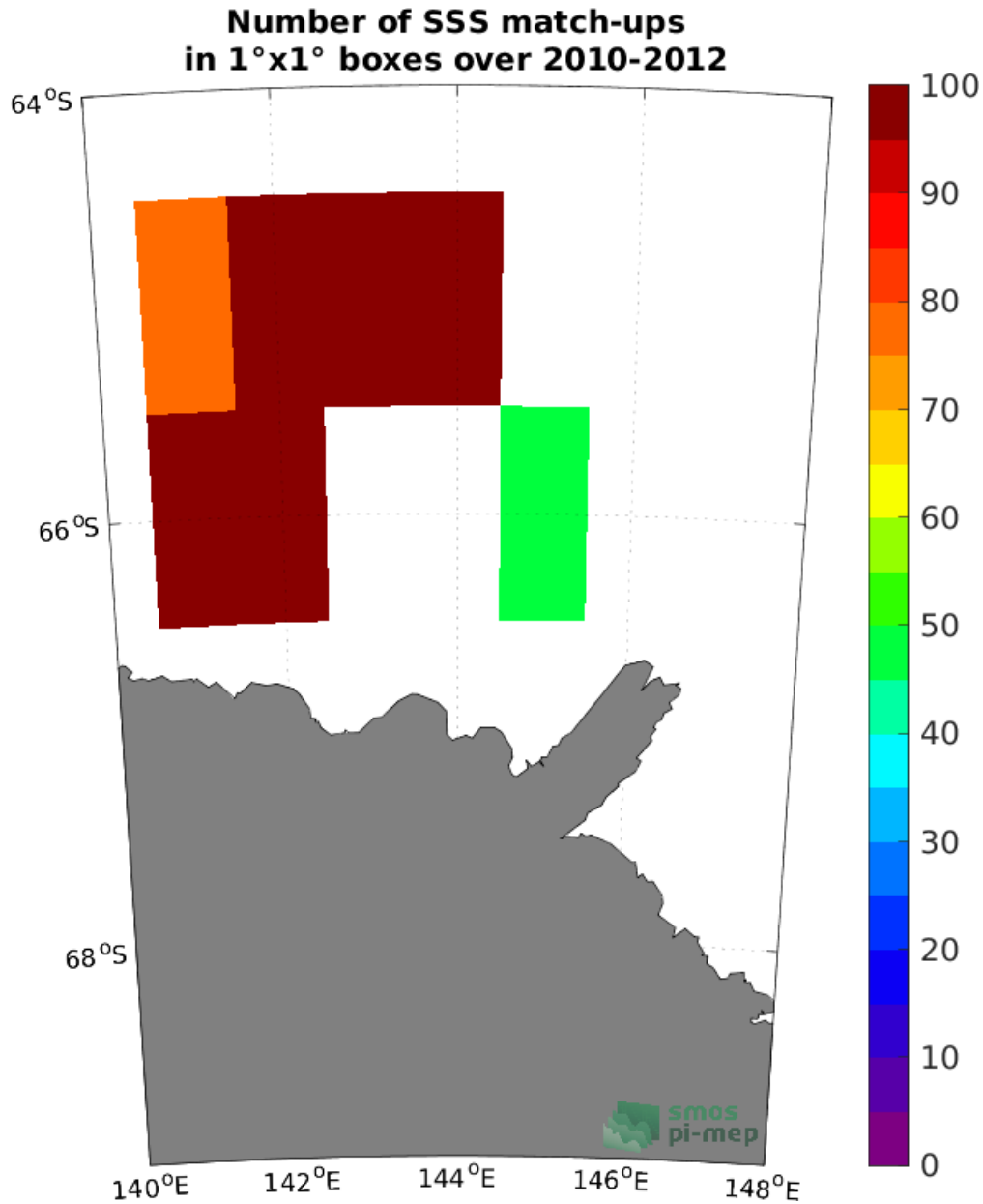
Figure 4: Number of SSS match-ups between TSG (LEGOS-Surv-Adel) SSS and the SMOS SSS L2Q v331 - With FLAG (CMEMS-CATDS-CPDC) SSS product for the Global Ocean Pi-MEP region over 1^\circ \times 1^\circ boxes and for the full satellite product period.
