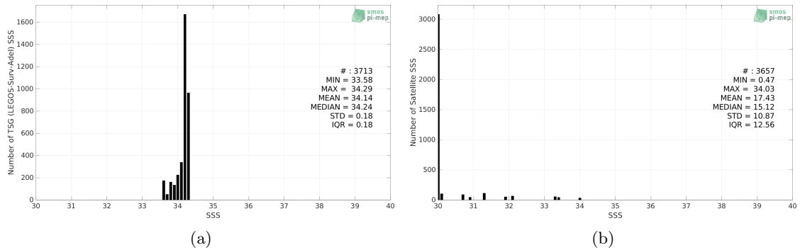
Figure 2: Histograms of SSS from TSG (LEGOS-Surv-Adel) (a) and SMOS SSS L2Q v331 - With FLAG (CMEMS-CATDS-CPDC) (b) considering all match-up pairs per bins of 0.1 over the Global Ocean Pi-MEP region and for the full satellite product period.
