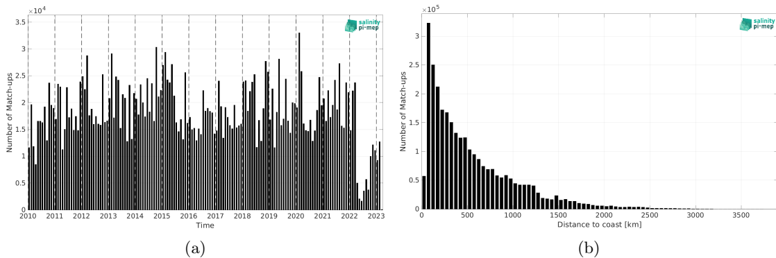
Figure 2: Number of match-ups between TSG (LEGOS-DM) and SMOS SSS L2Q v331 - With FLAG (CMEMS-CATDS-CPDC) SSS as a function of time (a) and as function of the distance to coast (b) over the Global Ocean Pi-MEP region and for the full satellite product period.
