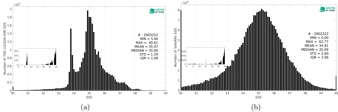
Figure 3: Histograms of SSS from TSG (LEGOS-DM) (a) and SMOS SSS L2Q v331 - With FLAG (CMEMS-CATDS-CPDC) (b) considering all match-up pairs per bins of 0.1 over the Global Ocean Pi-MEP region and for the full satellite product period.
