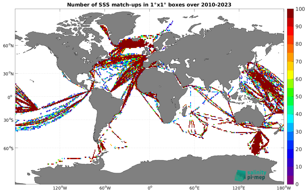
Figure 5: Number of SSS match-ups between TSG (LEGOS-DM) SSS and the SMOS SSS L2Q v331 - With FLAG (CMEMS-CATDS-CPDC) SSS product for the Global Ocean Pi-MEP region over 1^\circ \times 1^\circ boxes and for the full satellite product period.
