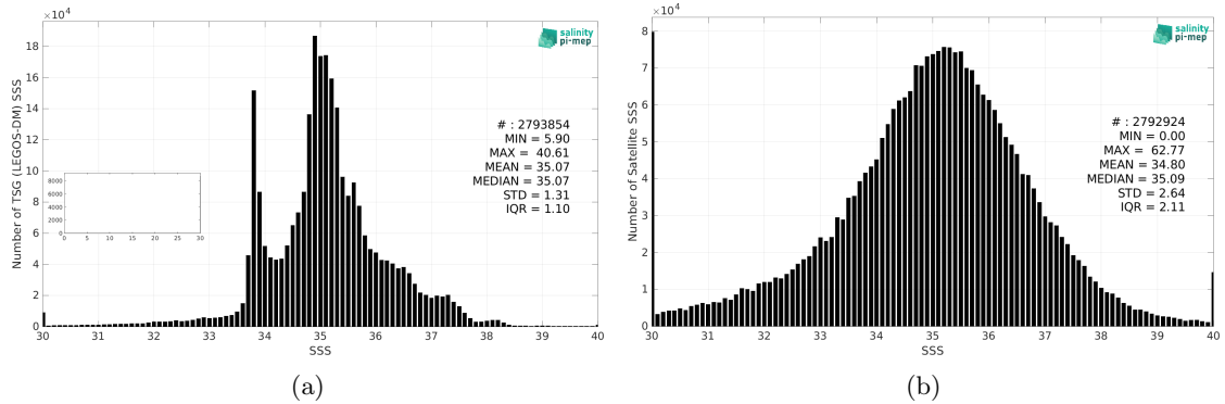
Figure 2: Histograms of SSS from TSG (LEGOS-DM) (a) and SMOS SSS L2Q v331 - With FLAG (CMEMS-CATDS-CPDC) (b) considering all match-up pairs per bins of 0.1 over the Global Ocean Pi-MEP region and for the full satellite product period.
