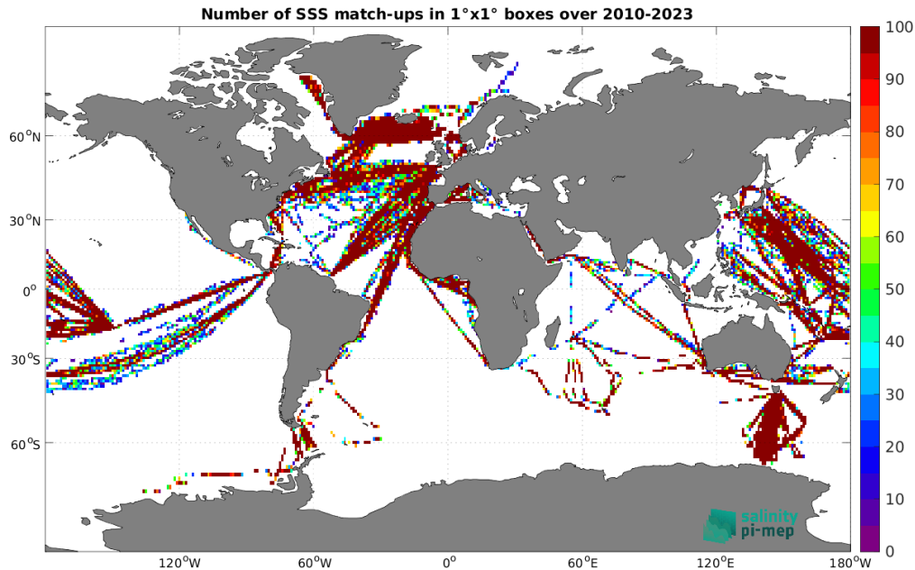
Figure 4: Number of SSS match-ups between TSG (LEGOS-DM) SSS and the SMOS SSS L2Q v331 - With FLAG (CMEMS-CATDS-CPDC) SSS product for the Global Ocean Pi-MEP region over 1^\circ \times 1^\circ boxes and for the full satellite product period.
