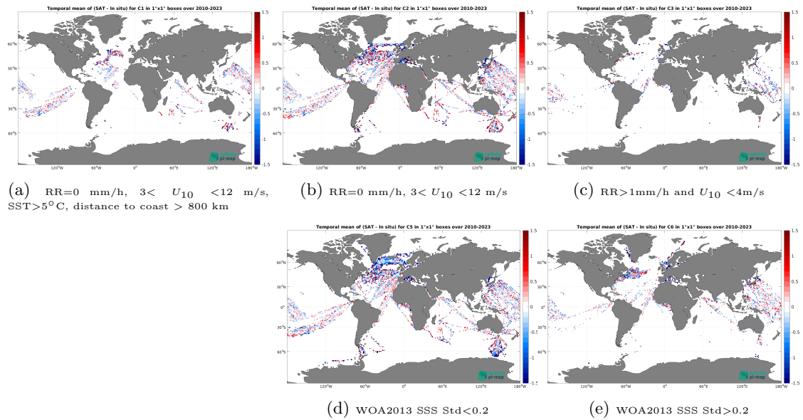
Figure 12: Temporal mean gridded over spatial boxes of size 1^\circ \times 1^\circ of \Delta\text{SSS} (SMOS SSS L2Q v331 - With FLAG (CMEMS-CATDS-CPDC) - TSG (LEGOS-DM)) for 5 different subdatasets corresponding to:RR=0 mm/h, 3 < U_{10} < 12 m/s, SST >5^\circ\text{C} , distance to coast > 800 km (a), RR=0 mm/h, 3 < U_{10} < 12 m/s (b), RR >1 mm/h and U_{10} < 4 m/s (c), WOA2013 SSS Std <0.2 (d), WOA2013 SSS Std >0.2 (e).
