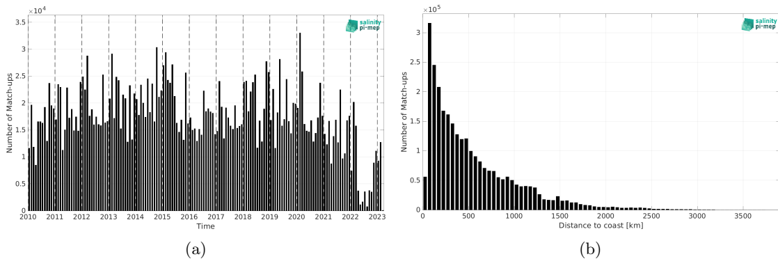
Figure 1: Number of match-ups between TSG (LEGOS-DM) and SMOS SSS L2Q v331 - With FLAG (CMEMS-CATDS-CPDC) SSS as a function of time (a) and as function of the distance to coast (b) over the Global Ocean Pi-MEP region and for the full satellite product period.
