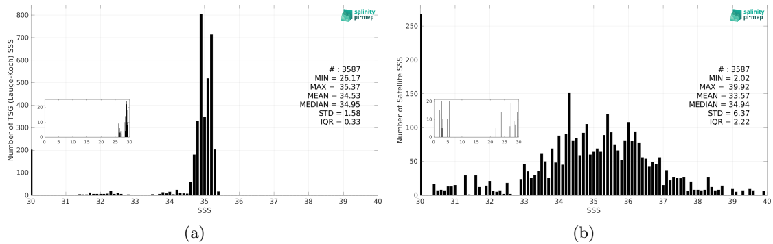
Figure 3: Histograms of SSS from TSG (Lauge-Koch) (a) and SMOS SSS L2Q v331 - With FLAG (CMEMS-CATDS-CPDC) (b) considering all match-up pairs per bins of 0.1 over the Global Ocean Pi-MEP region and for the full satellite product period.
