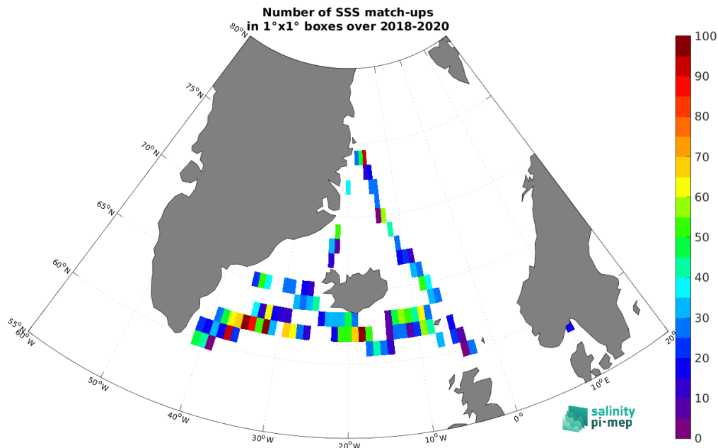
Figure 5: Number of SSS match-ups between TSG (Lauge-Koch) SSS and the SMOS SSS L2Q v331 - With FLAG (CMEMS-CATDS-CPDC) SSS product for the Global Ocean Pi-MEP region over 1^\circ \times 1^\circ boxes and for the full satellite product period.
