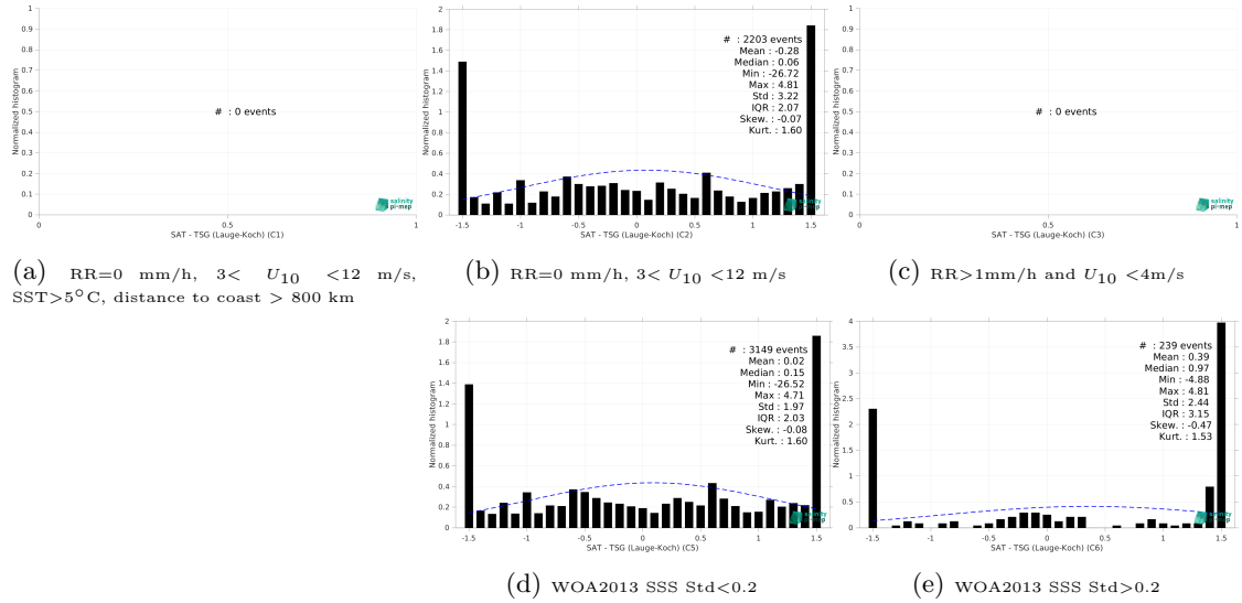
Figure 15: Normalized histogram of \Delta SSS (SMOS SSS L2Q v331 - With FLAG (CMEMS-CATDS-CPDC) - TSG (Laue-Koch)) for 5 different subdatasets corresponding to: RR=0 mm/h, 3 < U_{10} < 12 m/s, SST > 5°C, distance to coast > 800 km (a), RR=0 mm/h, 3 < U_{10} < 12 m/s (b), RR > 1mm/h and U_{10} < 4 m/s (c), WOA2013 SSS Std < 0.2 (d), WOA2013 SSS Std > 0.2 (e).
