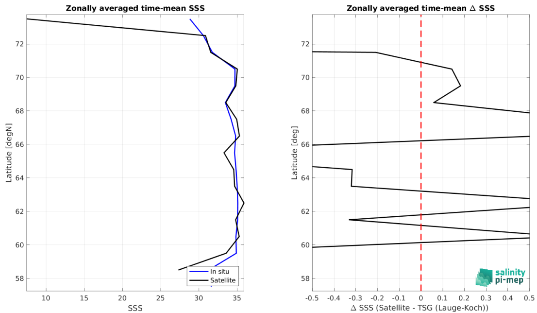
Figure 8: Left panel: Zonal mean SSS from SMOS SSS L2Q v331 - With FLAG (CMEMS-CATDS-CPDC) satellite product (black) and from TSG (Lauge-Koch) (blue). Right panel: Zonal mean of \Delta SSS (Satellite - TSG (Lauge-Koch)) for all the collected Pi-MEP match-up pairs estimated over the full satellite product period.
