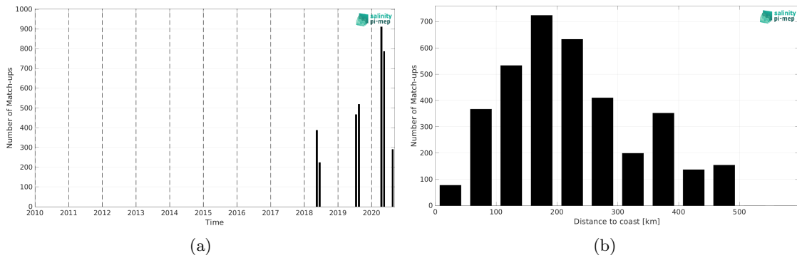
Figure 1: Number of match-ups between TSG (Lauge-Koch) and SMOS SSS L2Q v331 - With FLAG (CMEMS-CATDS-CPDC) SSS as a function of time (a) and as function of the distance to coast (b) over the Global Ocean Pi-MEP region and for the full satellite product period.
