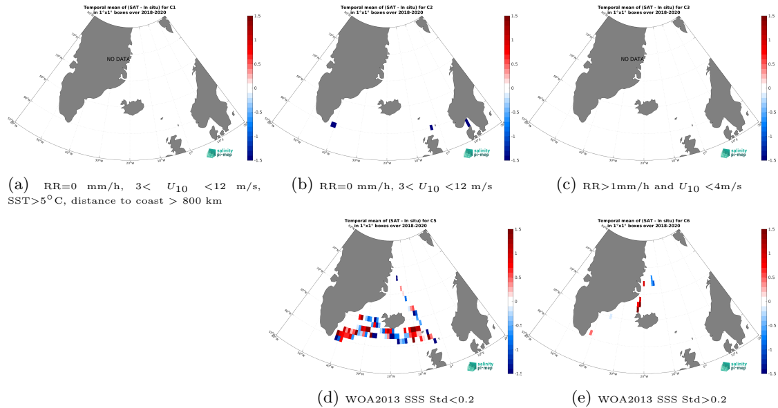
Figure 12: Temporal mean gridded over spatial boxes of size 1^{\circ}\times 1^{\circ} of \Delta\text{SSS} (SMOS SSS L2Q v331 - With FLAG (CMEMS-CATDS-CPDC) - TSG (Lauge-Koch)) for 5 different subdatasets corresponding to:RR=0 mm/h, 3 < U_{10} < 12 m/s, SST >5^{\circ}\text{C} , distance to coast > 800 km (a), RR=0 mm/h, 3 < U_{10} < 12 m/s (b), RR >1 mm/h and U_{10} < 4 m/s (c), WOA2013 SSS Std <0.2 (d), WOA2013 SSS Std >0.2 (e).
