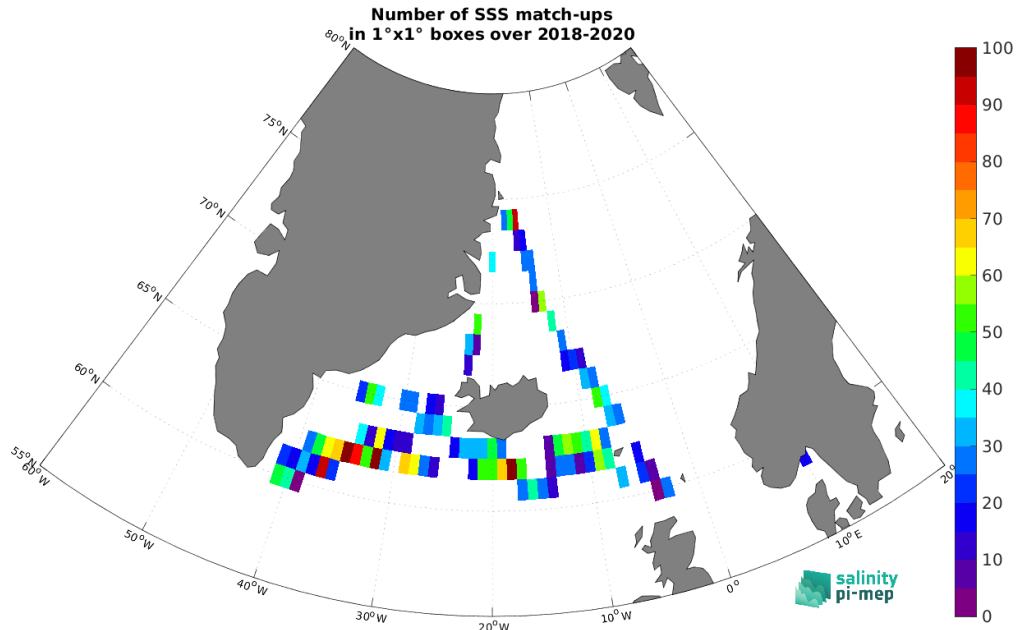
Figure 4: Number of SSS match-ups between TSG (Lauge-Koch) SSS and the SMOS SSS L2Q v331 - With FLAG (CMEMS-CATDS-CPDC) SSS product for the Global Ocean Pi-MEP region over 1^\circ \times 1^\circ boxes and for the full satellite product period.
