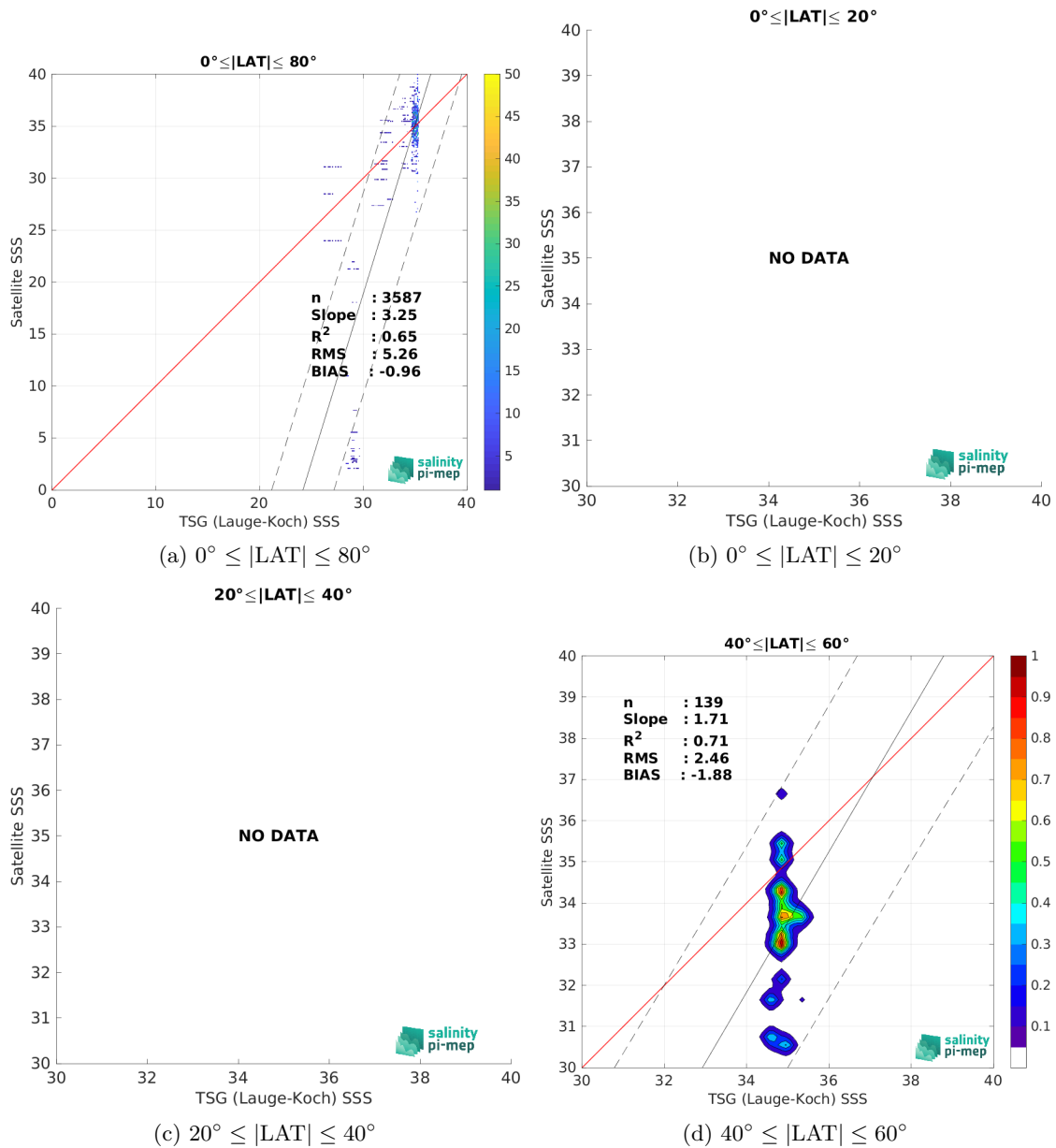
Figure 9: Contour maps of the concentration of SMOS SSS L2Q v331 - With FLAG (CMEMS-CATDS-CPDC) SSS (y-axis) versus TSG (Lauge-Koch) SSS (x-axis) at match-up pairs for different latitude bands. For each plot, the red line shows x=y . The black thin and dashed lines indicate a linear fit through the data cloud and the \pm 95\% confidence levels, respectively. The number match-up pairs n , the slope and R^2 coefficient of the linear fit, the root mean square (RMS) and the mean bias between satellite and in situ data are indicated for each latitude band in each plots.
