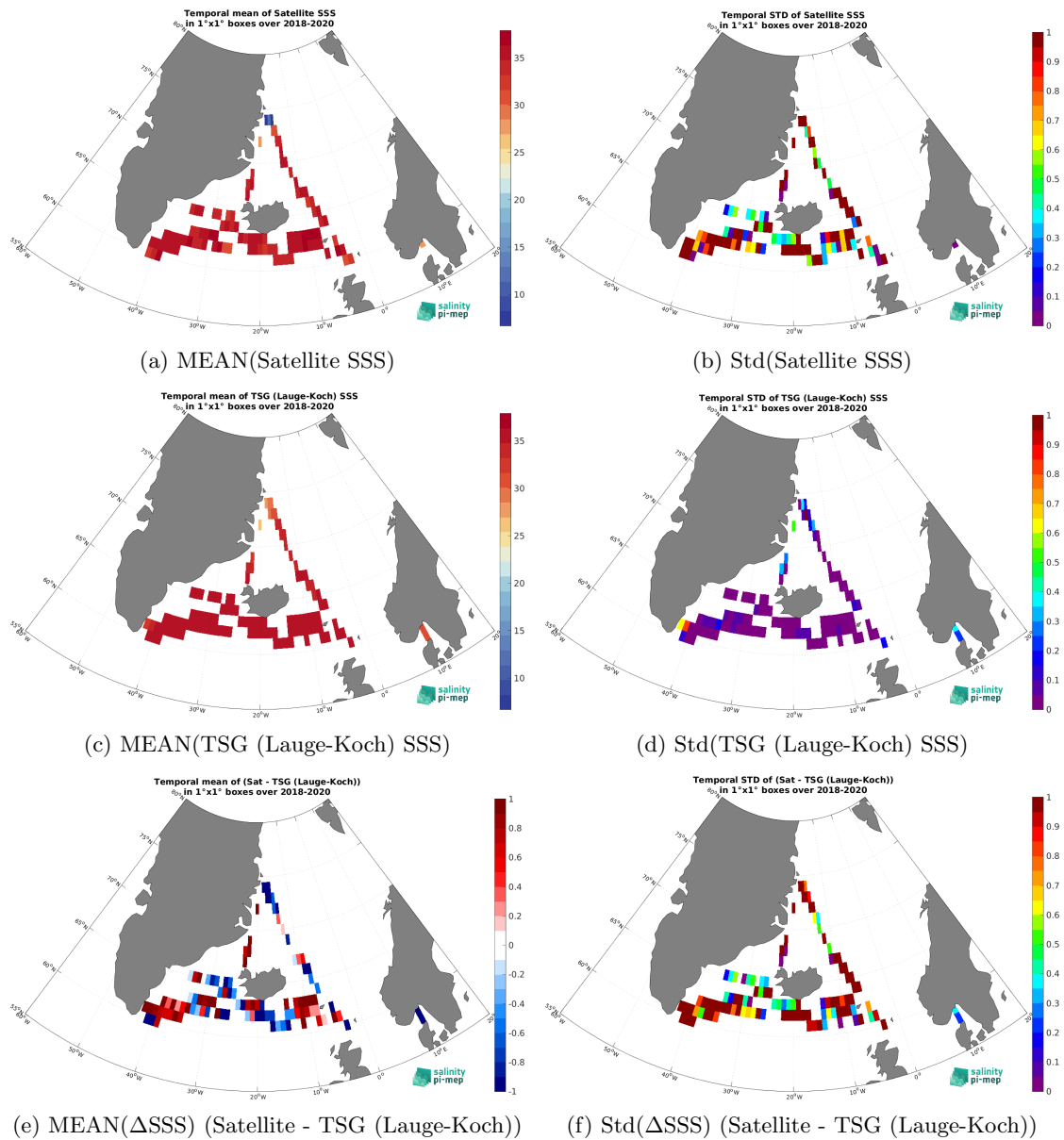
Figure 6: Temporal mean (left) and Std (right) of SSS from SMOS SSS L2Q v331 - With FLAG (CMEMS-CATDS-CPDC) (top), TSG (Lauge-Koch) (middle), and of \Delta SSS (Satellite - TSG (Lauge-Koch)). Only match-up pairs are used to generate these maps.
