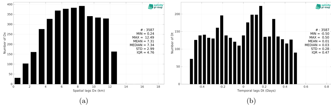
Figure 5: Histograms of the spatial (a) and temporal (b) lags between the location/time of the TSG (Lauge-Koch) measurement and the date of the corresponding SMOS SSS L2Q v331 - With FLAG (CMEMS-CATDS-CPDC) SSS pixel.
