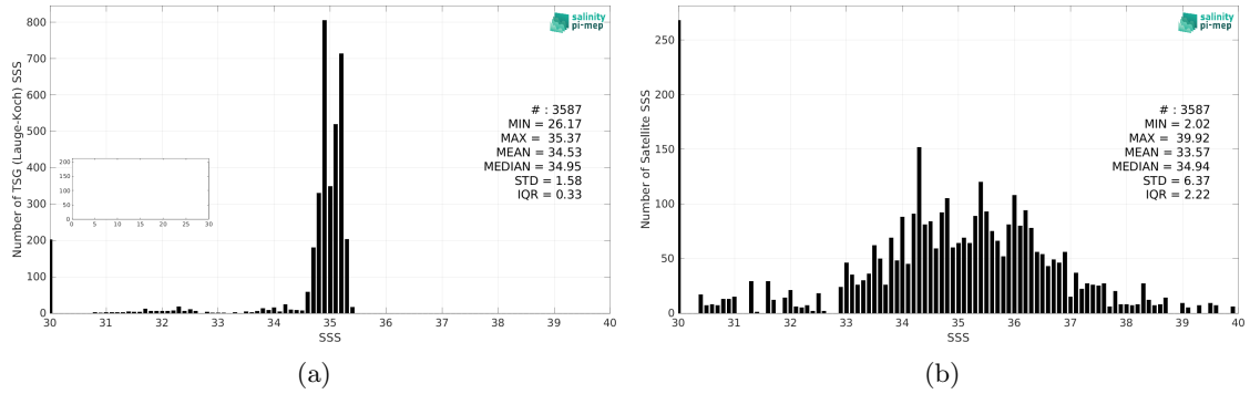
Figure 2: Histograms of SSS from TSG (Lauge-Koch) (a) and SMOS SSS L2Q v331 - With FLAG (CMEMS-CATDS-CPDC) (b) considering all match-up pairs per bins of 0.1 over the Global Ocean Pi-MEP region and for the full satellite product period.
