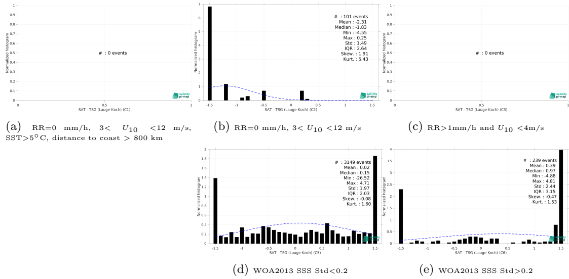
Figure 13: Normalized histogram of \Delta SSS (SMOS SSS L2Q v331 - With FLAG (CMEMS-CATDS-CPDC) - TSG (Lauge-Koch)) for 5 different subdatasets corresponding to: RR=0 mm/h, 3 < U_{10} < 12 m/s, SST > 5°C, distance to coast > 800 km (a), RR=0 mm/h, 3 < U_{10} < 12 m/s (b), RR > 1mm/h and U_{10} < 4 m/s (c), WOA2013 SSS Std < 0.2 (d), WOA2013 SSS Std > 0.2 (e).
