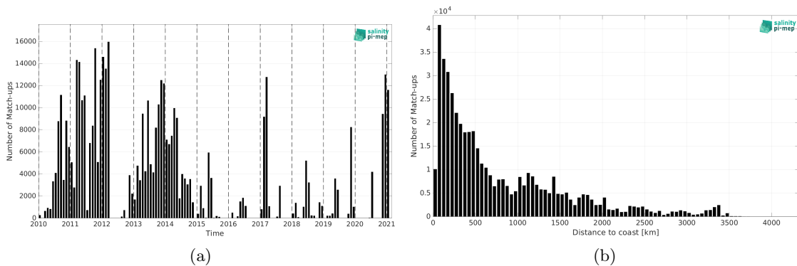
Figure 2: Number of match-ups between TSG (GOSUD-Sailing-ship) and SMOS SSS L2Q v331 - With FLAG (CMEMS-CATDS-CPDC) SSS as a function of time (a) and as function of the distance to coast (b) over the Global Ocean Pi-MEP region and for the full satellite product period.
