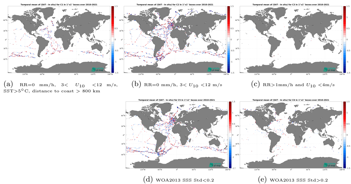
Figure 14: Temporal mean gridded over spatial boxes of size 1^\circ \times 1^\circ of \Delta SSS (SMOS SSS L2Q v331 - With FLAG (CMEMS-CATDS-CPDC) - TSG (GOSUD-Sailing-ship)) for 5 different subdatasets corresponding to:RR=0 mm/h, 3 < U_{10} < 12 m/s, SST > 5^\circ\text{C} , distance to coast > 800 km (a), RR=0 mm/h, 3 < U_{10} < 12 m/s (b), RR > 1 mm/h and U_{10} < 4 m/s (c), WOA2013 SSS Std < 0.2 (d), WOA2013 SSS Std > 0.2 (e).
