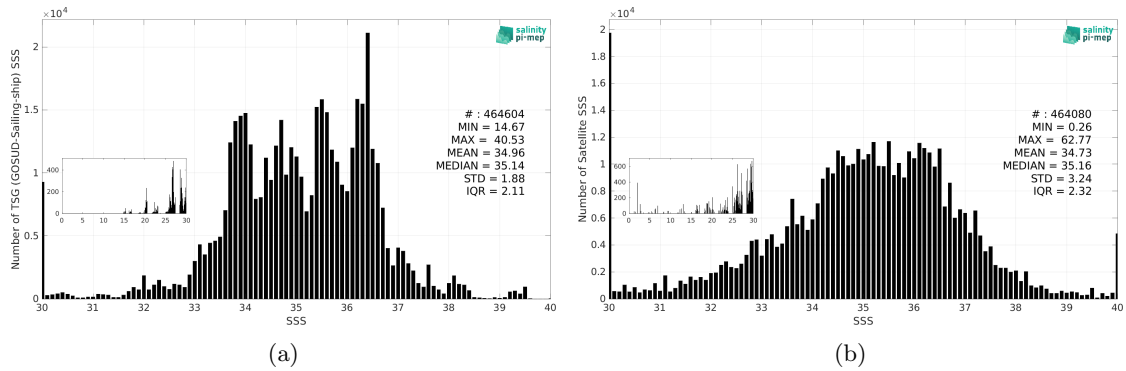
Figure 3: Histograms of SSS from TSG (GOSUD-Sailing-ship) (a) and SMOS SSS L2Q v331 - With FLAG (CMEMS-CATDS-CPDC) (b) considering all match-up pairs per bins of 0.1 over the Global Ocean Pi-MEP region and for the full satellite product period.
