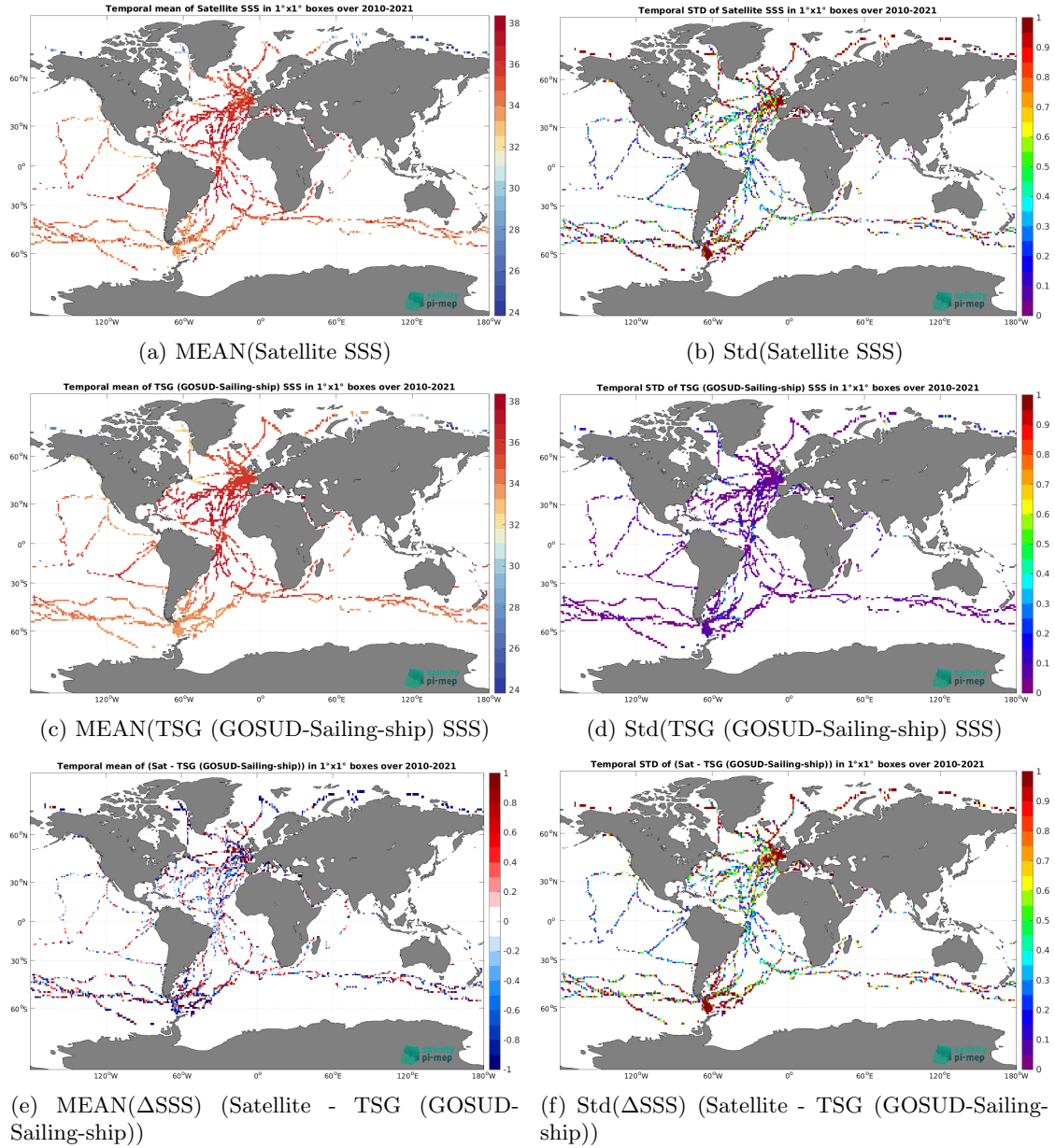
Figure 7: Temporal mean (left) and Std (right) of SSS from SMOS SSS L2Q v331 - With FLAG (CMEMS-CATDS-CPDC) (top), TSG (GOSUD-Sailing-ship) (middle), and of \Delta SSS (Satellite - TSG (GOSUD-Sailing-ship)). Only match-up pairs are used to generate these maps.
