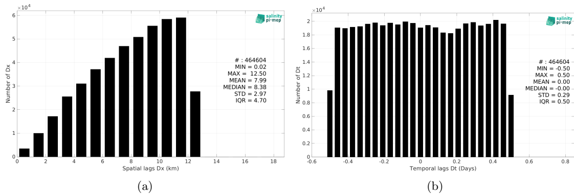
Figure 6: Histograms of the spatial (a) and temporal (b) lags between the location/time of the TSG (GOSUD-Sailing-ship) measurement and the date of the corresponding SMOS SSS L2Q v331 - With FLAG (CMEMS-CATDS-CPDC) SSS pixel.
