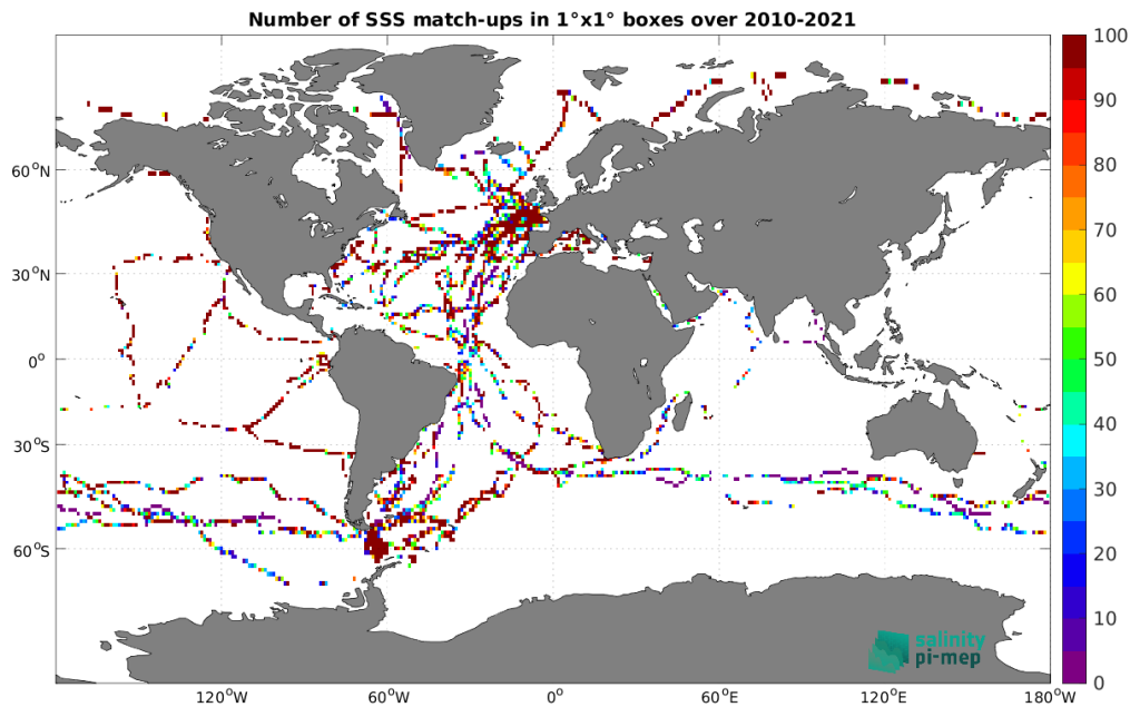
Figure 5: Number of SSS match-ups between TSG (GOSUD-Sailing-ship) SSS and the SMOS SSS L2Q v331 - With FLAG (CMEMS-CATDS-CPDC) SSS product for the Global Ocean Pi-MEP region over 1°×1° boxes and for the full satellite product period.
