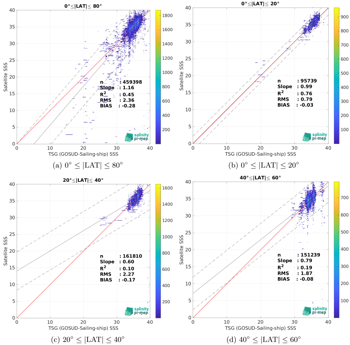
Figure 10: Contour maps of the concentration of SMOS SSS L2Q v331 - With FLAG (CMEMS-CATDS-CPDC) SSS (y-axis) versus TSG (GOSUD-Sailing-ship) SSS (x-axis) at match-up pairs for different latitude bands. For each plot, the red line shows x=y . The black thin and dashed lines indicate a linear fit through the data cloud and the \pm 95\% confidence levels, respectively. The number match-up pairs n , the slope and R^2 coefficient of the linear fit, the root mean square (RMS) and the mean bias between satellite and in situ data are indicated for each latitude band in each plots.
