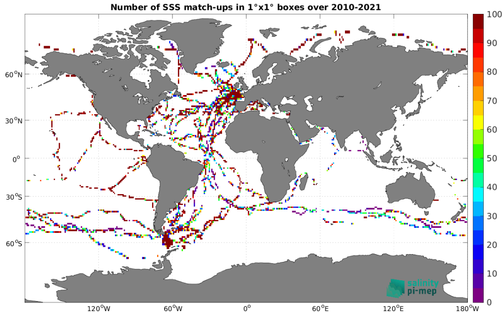
Figure 4: Number of SSS match-ups between TSG (GOSUD-Sailing-ship) SSS and the SMOS SSS L2Q v331 - With FLAG (CMEMS-CATDS-CPDC) SSS product for the Global Ocean Pi-MEP region over 1^\circ \times 1^\circ boxes and for the full satellite product period.
