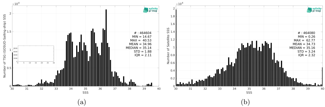
Figure 2: Histograms of SSS from TSG (GOSUD-Sailing-ship) (a) and SMOS SSS L2Q v331 - With FLAG (CMEMS-CATDS-CPDC) (b) considering all match-up pairs per bins of 0.1 over the Global Ocean Pi-MEP region and for the full satellite product period.
