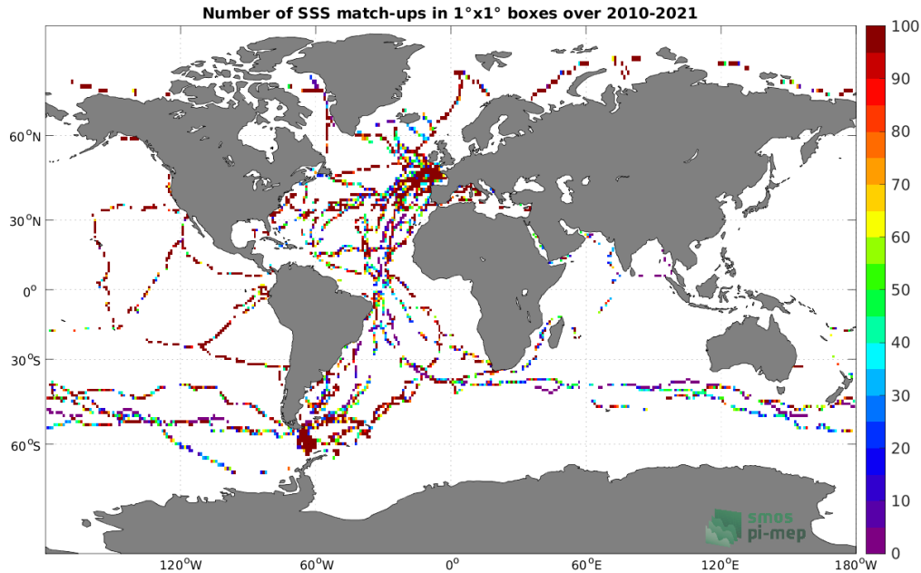
Figure 4: Number of SSS match-ups between TSG (GOSUD-Sailing-ship) SSS and the SMOS SSS L2Q v331 - With FLAG (CMEMS-CATDS-CPDC) SSS product for the Global Ocean Pi-MEP region over 1°×1° boxes and for the full satellite product period.
