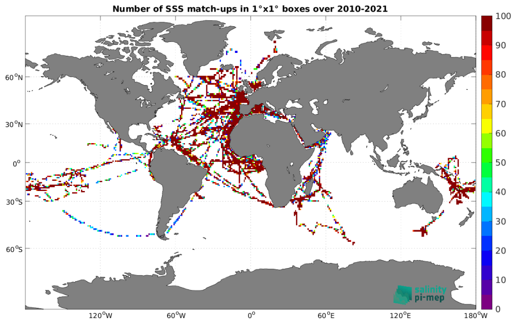
Figure 5: Number of SSS match-ups between TSG (GOSUD-Research-vessel) SSS and the SMOS SSS L2Q v331 - With FLAG (CMEMS-CATDS-CPDC) SSS product for the Global Ocean Pi-MEP region over 1^\circ \times 1^\circ boxes and for the full satellite product period.
