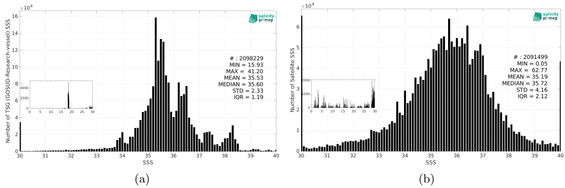
Figure 3: Histograms of SSS from TSG (GOSUD-Research-vessel) (a) and SMOS SSS L2Q v331 - With FLAG (CMEMS-CATDS-CPDC) (b) considering all match-up pairs per bins of 0.1 over the Global Ocean Pi-MEP region and for the full satellite product period.
