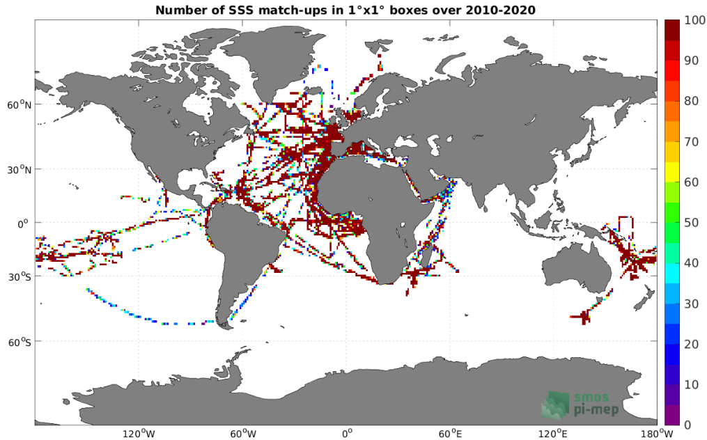
Figure 4: Number of SSS match-ups between TSG (GOSUD-Research-vessel) SSS and the SMOS SSS L2Q v331 - With FLAG (CMEMS-CATDS-CPDC) SSS product for the Global Ocean Pi-MEP region over 1^\circ \times 1^\circ boxes and for the full satellite product period.
