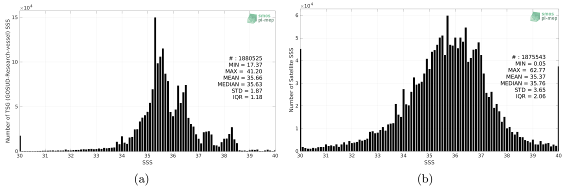
Figure 2: Histograms of SSS from TSG (GOSUD-Research-vessel) (a) and SMOS SSS L2Q v331 - With FLAG (CMEMS-CATDS-CPDC) (b) considering all match-up pairs per bins of 0.1 over the Global Ocean Pi-MEP region and for the full satellite product period.
